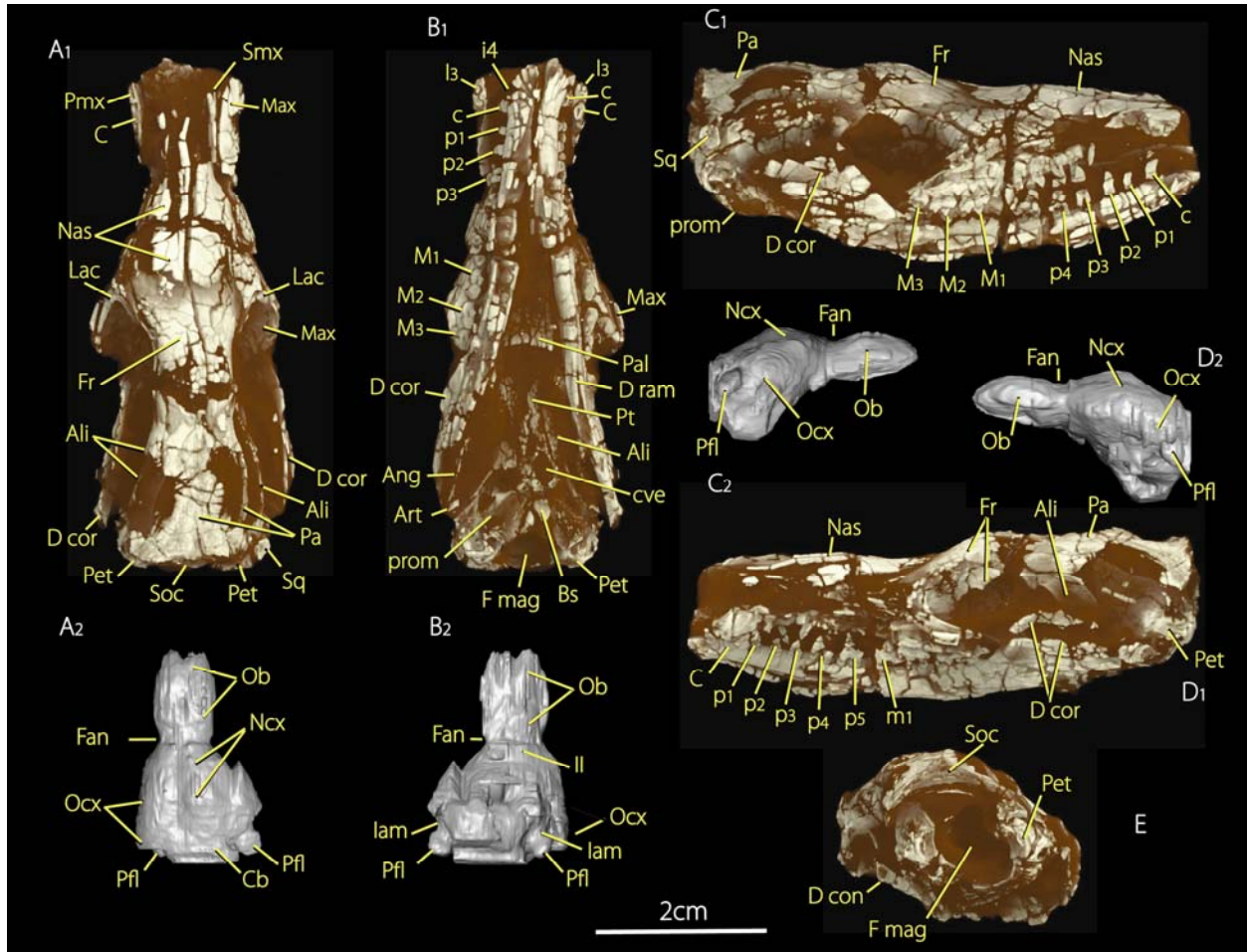
Figure S1. 3D reconstruction from HRXCT data of the skull and endocast of Morganucodon oehleri (IVPP 8685). Skull and endocast in dorsal (A1, A2), ventral (B1, B2), right lateral (C1, C2), left lateral (D1, D2), and (E) occipital views. Abbreviations are listed below (p. 14).
