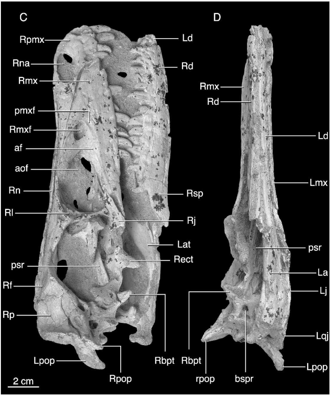
Fig. 3. (Continued). C, holotype of Tsaagan mangas (IGM 100/1015) in right lateral view. D, holotype of Tsaagan mangas (IGM 100/1015) in ventral view. Abbreviations are in appendix 1.
