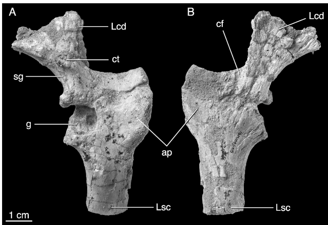
Fig. 21. Left scapulocoracoid of the holotype of Tsaagan mangas (IGM 100/1015) in lateral (A) and medial (B) views. Abbreviations are in appendix 1.
