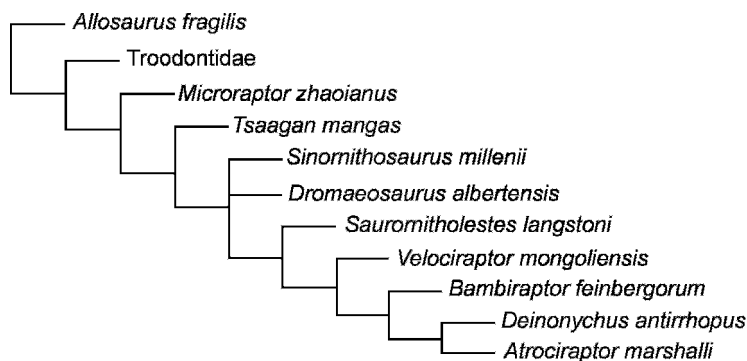
Fig. 23. The phylogenetic result of incorporating Tsaagan mangas into the revised dataset of Currie and Varrichio (2004). A strict consensus shows the results of a branch-and-bound search conducted in PAUP* (v. 4.0b10). Two most parsimonious trees of length 64 (CI = 0.7344, RI = 0.7733) were found. See the text for tree shape details.
