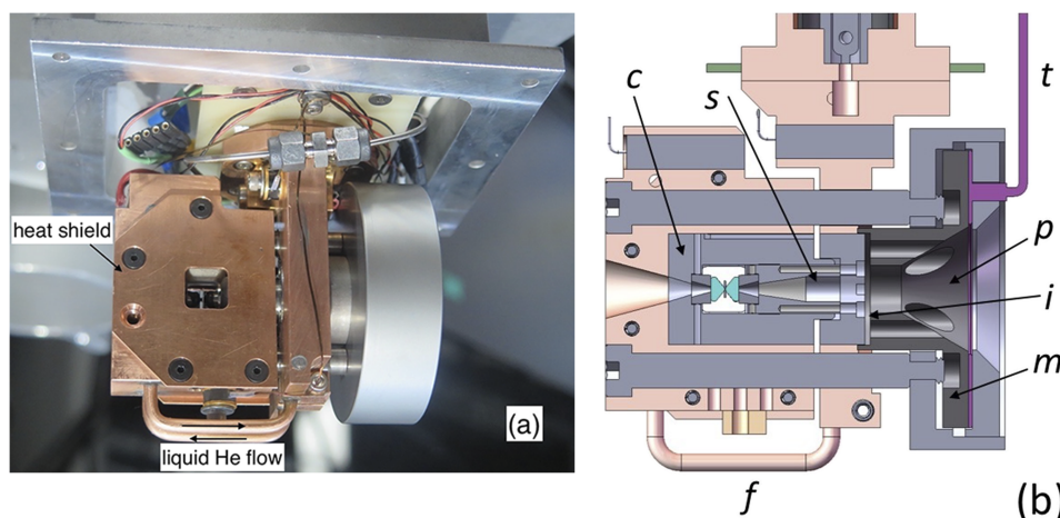
FIG. 2. (a) Picture of the cryostat cold head, gas membrane system, and diamond anvil cell holder. (b) A cross-sectional view of the instrument. “c”: cylinder and “s”: piston of the mini-pDAC; “p”: the pusher of the membrane; “t”: a 1.5875 mm OD steel capillary tube extended to outside the cryostat for helium gas supply; “i”: a ceramic thermal insulation layer between the cell and the pusher; “f”: liquid helium flow line around the cell; “m”: the membrane.
