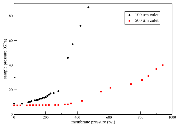
FIG. 4. Testing results of the pressure reached on the sample versus the membrane pressure in mini-pDACs. The anvil size is 100 \mu m and 500 \mu m, respectively. Sample pressures were altered when the sample temperature was around 120 K.
