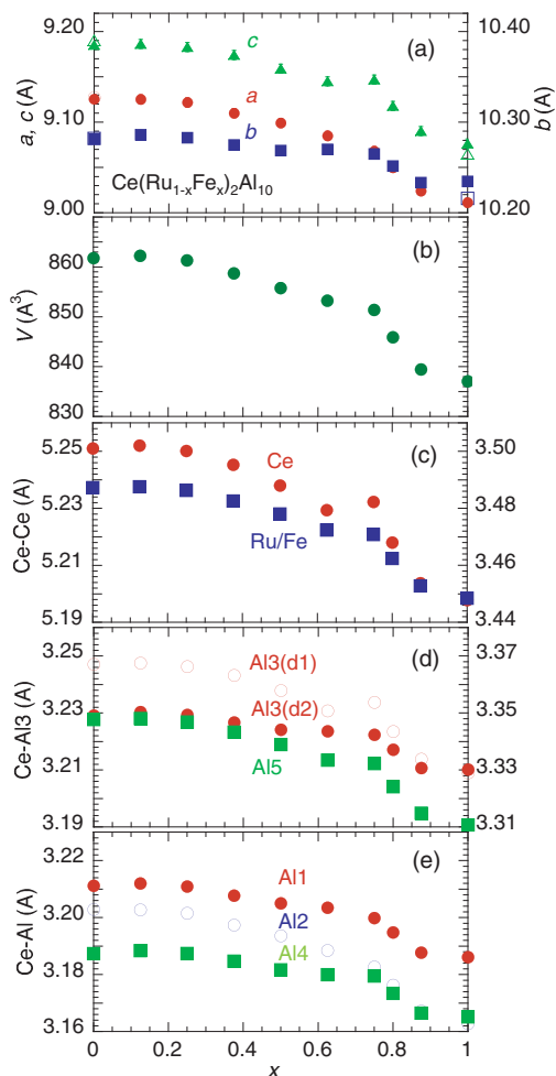
FIG. 1. (Color online) (a) Change in the orthorhombic lattice parameters of a , b , and c as a function of x for \text{Ce}(\text{Ru}_{1-x}\text{Fe}_x)_2\text{Al}_{10} ( x = 0 to 1.0) at 300 K. (b) Change in the volume as a function of x . Data errors are comparable to the symbol sizes. (c)–(e) Interatomic distance as a function of x for \text{Ce}(\text{Ru}_{1-x}\text{Fe}_x)_2\text{Al}_{10} .
