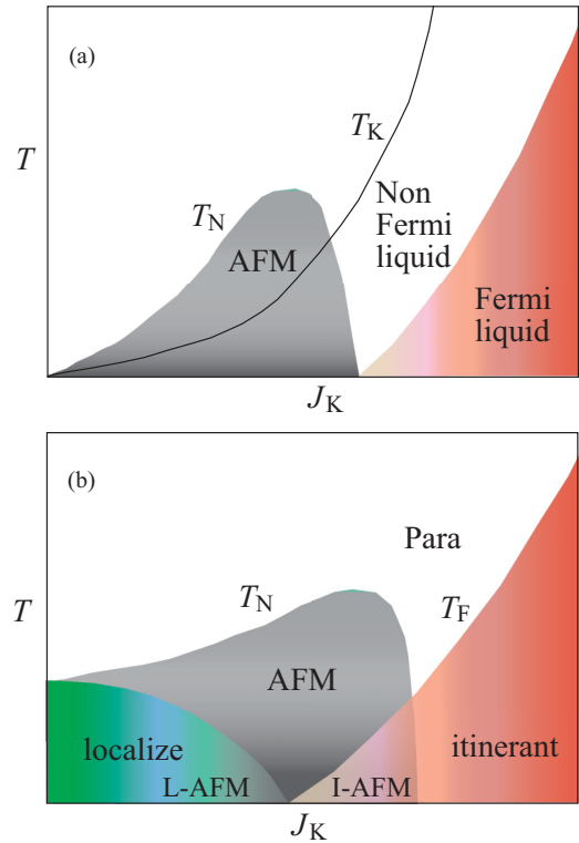
FIG. 4. (Color online) (a) Conventional Doniach phase diagram. There is a clear separation between the magnetically ordered state and the itinerant Fermi liquid [1]. (b) A phase diagram based on the calculation for the Kondo-Heisenberg lattice at finite temperatures [4].
