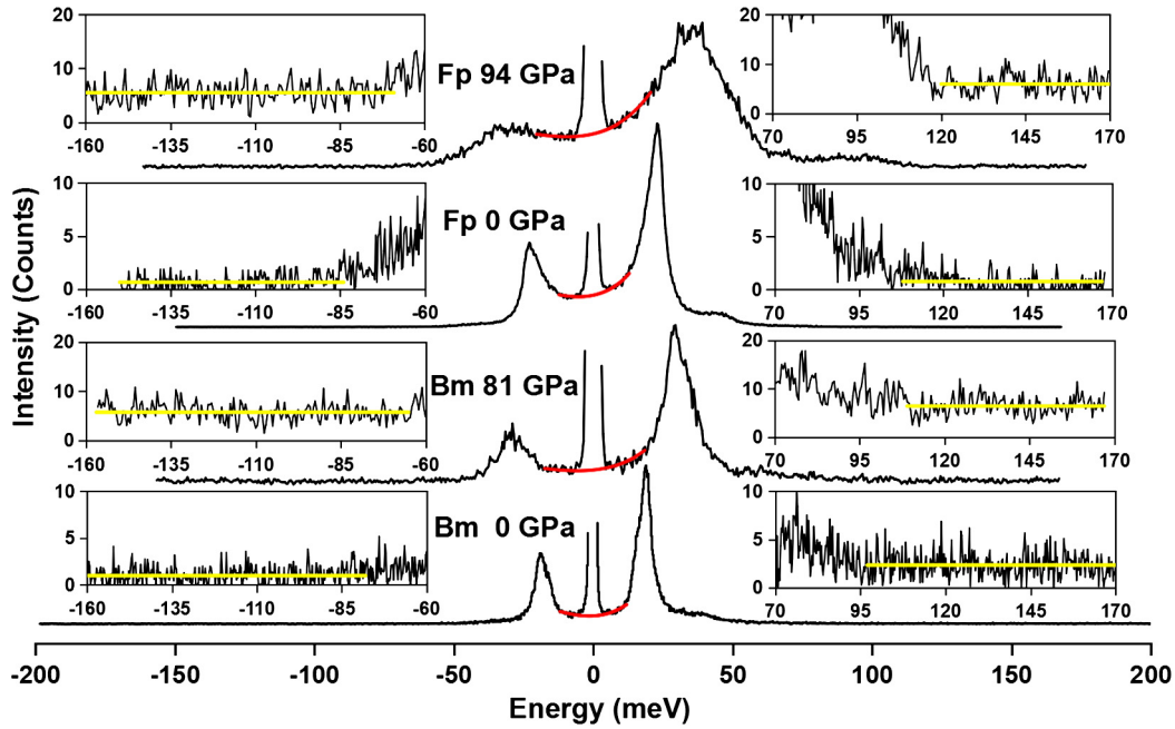
Fig. 2. Representative energy spectra of (Fe,Al)-bearing bridgmanite ( \text{Mg}_{0.89}\text{Fe}_{0.024}^{2+}\text{Fe}_{0.096}^{3+}\text{Al}_{0.11}\text{Si}_{0.89}\text{O}_3 ) and ferropericase ( (\text{Mg}_{0.75}\text{Fe}_{0.25})\text{O} ) at high pressure. The central peaks located near 0 meV (partially truncated in the plots) correspond to the nuclear elastic scattering of the incident X-rays, while the other spectral features correspond to inelastically-scattered photons either due to phonon creation ( E > 0 ) or phonon annihilation ( E < 0 ). The red curves are interpolations of the energy spectra used to remove the elastic peak. The yellow horizontal lines are averages in the close-up views of the spectrum tails at low and high energy ends of the scans, which were interpolated for the subtraction of the baseline. Elastic peak removal and baseline subtraction were conducted using SciPhon (Dauphas et al., 2018). The extended energy range reaching \pm 200 meV, together with the extremely low baseline level, were critical for an accurate evaluation of the force constants of iron in the samples at high pressure (see Fig. 3 for details). (For interpretation of the colors in the figure(s), the reader is referred to the web version of this article.)
