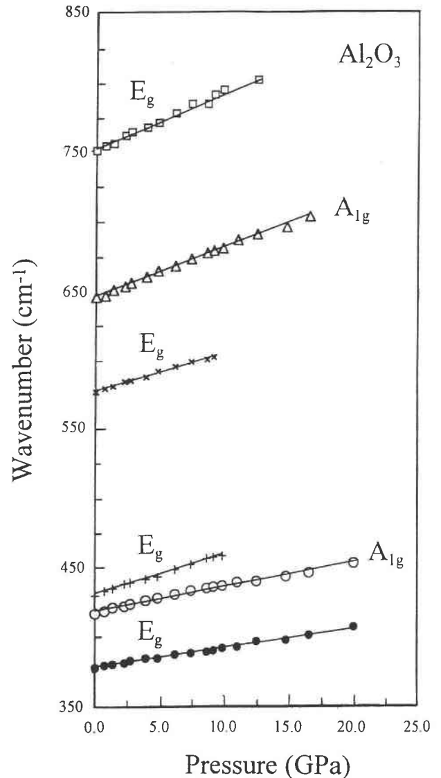
Fig. 2. Variation of Raman mode frequencies with pressure.
