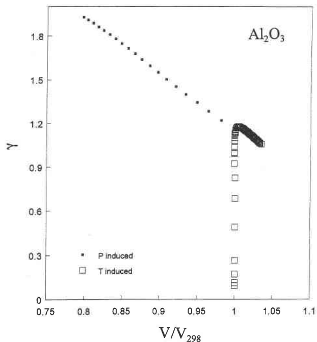
Fig. 7. Gruneisen parameter \gamma as a function of the volume of corundum by pressure (small squares) and temperature (large squares). It is evident that the hypothesis that the Gruneisen parameter is solely a function of volume ( V ) is correct except in low-temperature conditions.
