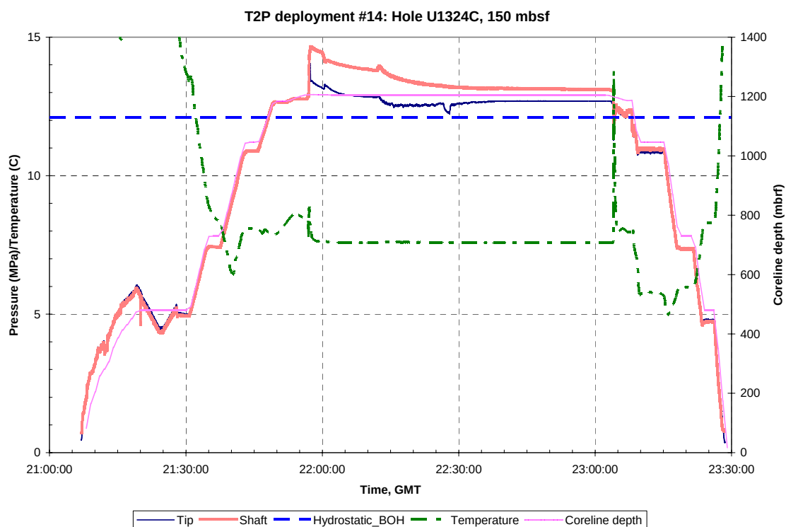
Figure A.B.20.a: Pressure, temperature and Truview data for T2P deployment #14, Hole U1324C, 150 mbsf. GMT = Greenwich Mean Time, Hydrostatic_BOH is the hydrostatic pressure at the bottom of the hole.
