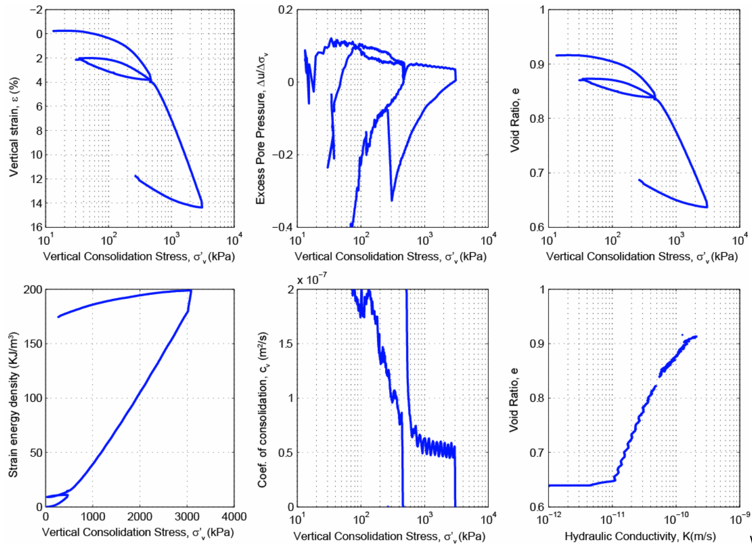
Figure B.13: CRS812 consolidation data for Sample U1324B-23H-5WR, 200 mbsf.
