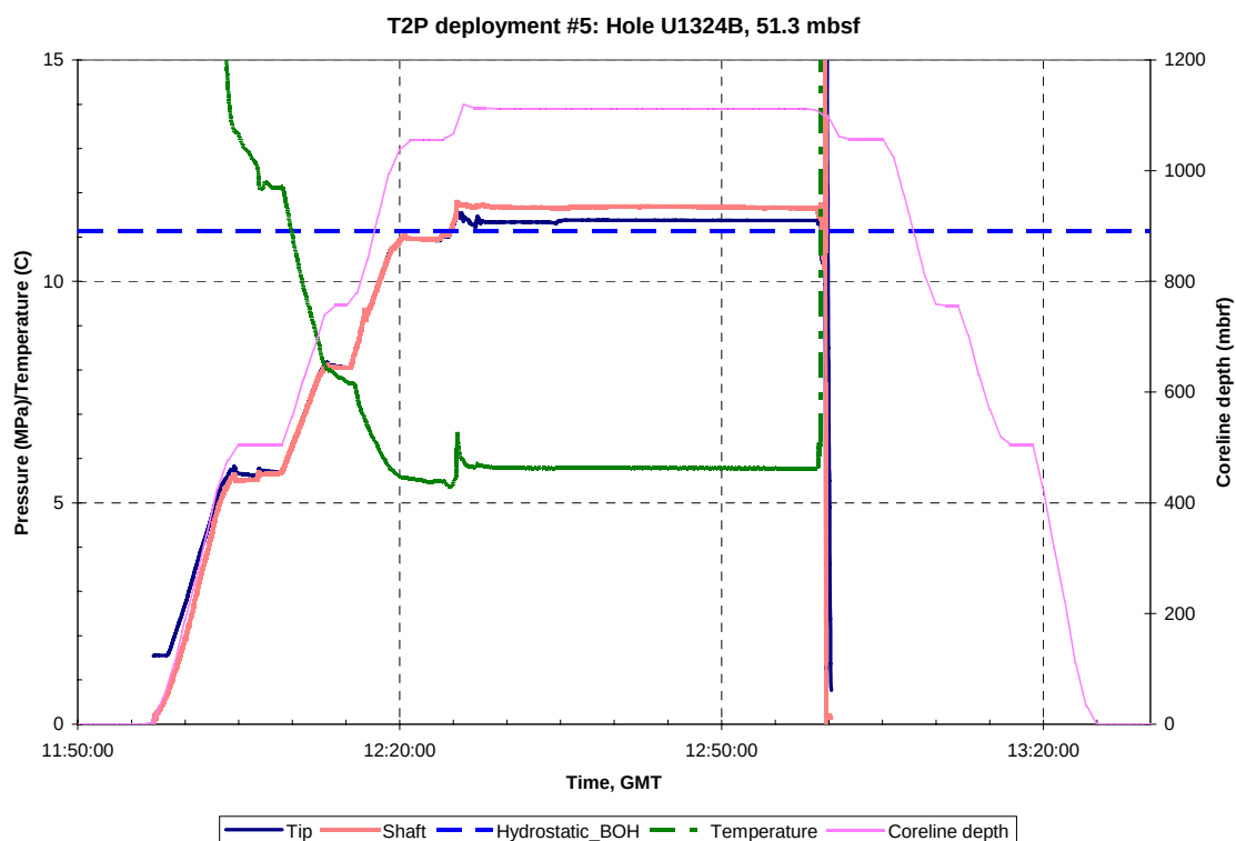
Figure A.B.12.a: Pressure, temperature and Truview data for T2P deployment #5, Hole U1324B, 51.3 mbsf. GMT = Greenwich Mean Time, Hydrostatic_BOH is the hydrostatic pressure at the bottom of the hole.
