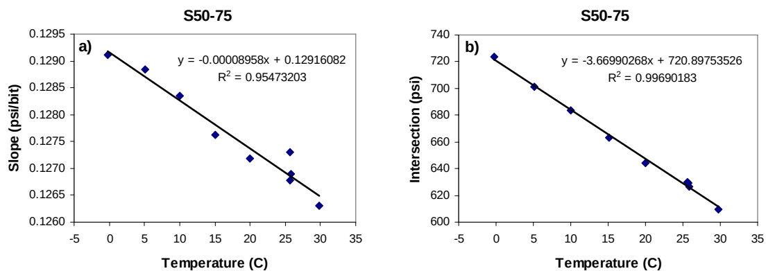
Figure A.B.6 : Calibration coefficients of transducer S50-75 vs. temperature. a) The slope of the calibration curve vs. temperature. b) The intersection on y-axis of the calibration curve vs. temperature.
