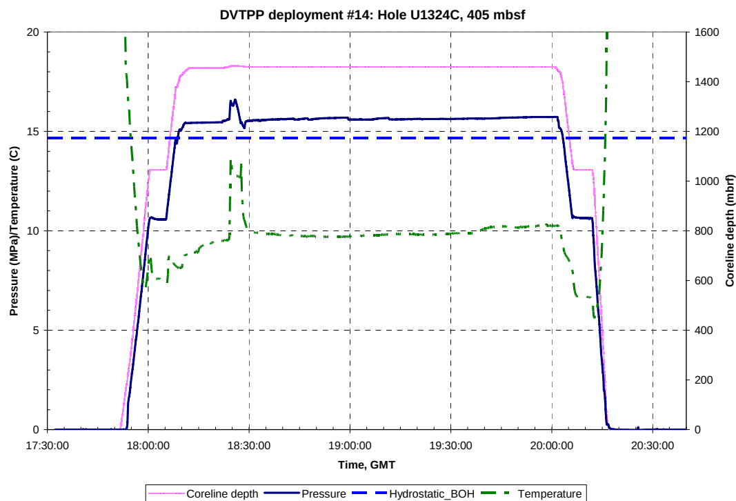
Figure A.A.13.a: Pressure, temperature and Truview data for DVTPP Deployment #14, Hole U1324C, 405 mbsf. GMT = Greenwich Mean Time, Hydrostatic_BOH is the hydrostatic pressure at the bottom of the hole.
