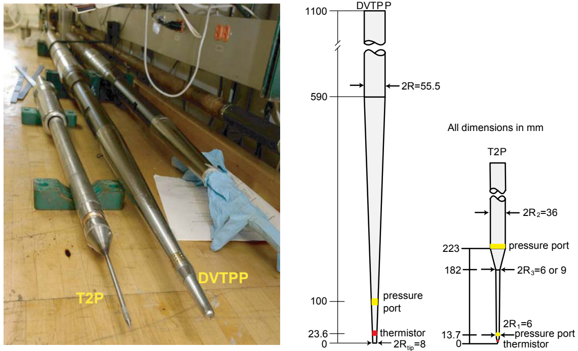
Figure 2.1: The DVTPP and T2P pore pressure penetrometers have very different geometries. The DVTPP has a long, tapered tip that extends beyond the constant diameter shaft. Its tip tapers continuously from 8 to 55.5 mm in diameter. The pressure port is located 100 mm above the tip. The T2P has a tapered extension piece 223 mm long which fits onto the end of a standard 36 mm diameter cone rod. Its modular design allows the use of multiple tip geometries and it measures pore pressure at its narrow tip and at the larger diameter shaft behind the narrow tip.
