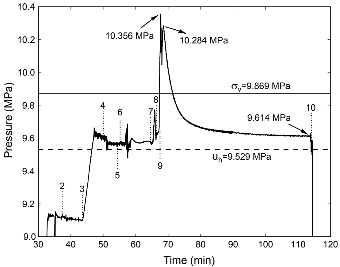
Figure 1.A2: Pressure records for the Piezoprobe deployment. The deployment events are identified by numbers and are explained in Table 1.3. See Appendix 1.A for discussion.
