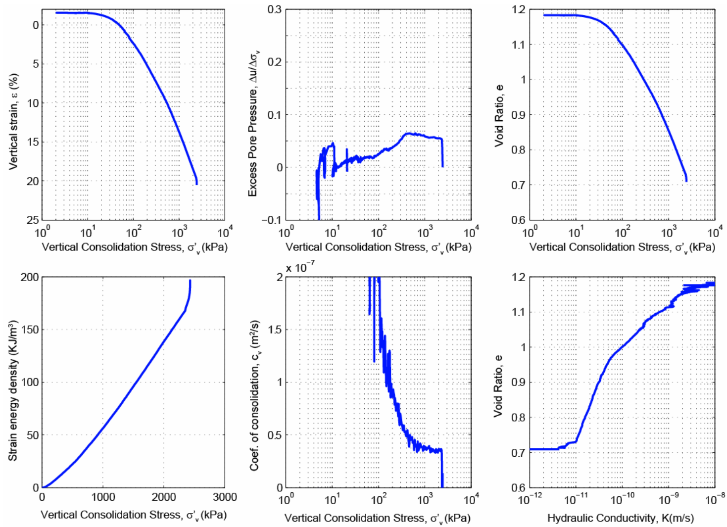
Figure B.16: CRS824 consolidation data for Sample U1322B-25H-6WR, 209.81 mbsf.
