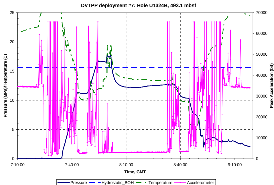
Figure A.A.7: Pressure, temperature and acceleration data for DVTPP Deployment #7, Hole U1324B, 493.1 mbsf. GMT = Greenwich Mean Time, Hydrostatic_BOH is the hydrostatic pressure at the bottom of the hole.
