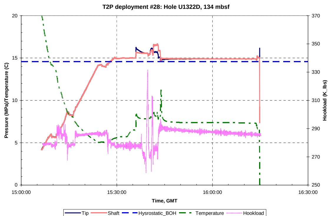
Figure A.B.31.e: Pressure, temperature and Truview data for T2P deployment #28, Hole U1322D, 134 mbsf. GMT = Greenwich Mean Time, Hydrostatic_BOH is the hydrostatic pressure at the bottom of the hole.
