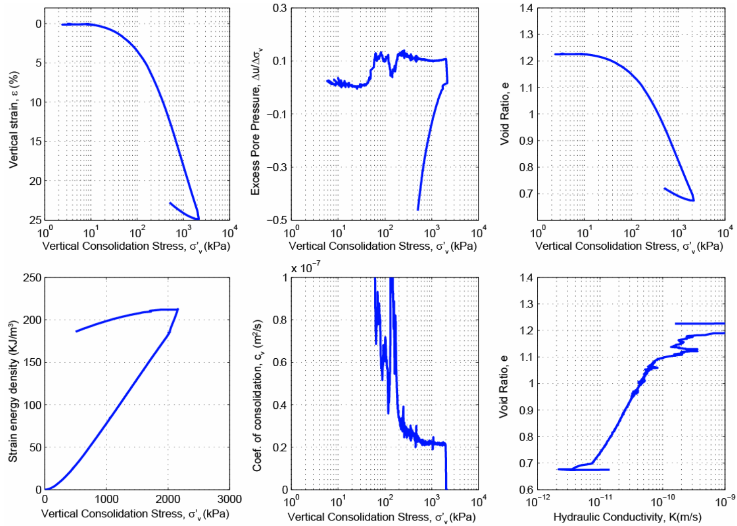
Figure B.8: CRS802 consolidation data for Sample U1324B-7H-7WR, 60.31 mbsf.
