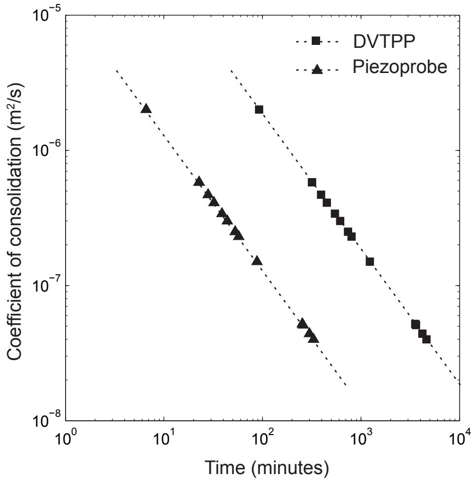
Figure 1.16: Time to dissipate 90% of the induced pressure as a function of coefficient of consolidation for the DVTPP (squares) and the Piezoprobe (triangles). The Piezoprobe reaches 90% dissipation 14 times sooner than the DVTPP. Coefficients of consolidation for sediments penetrated in the Ocean Drilling Program range from 4 \times 10^{-8} to 2 \times 10^{-6} \text{ m}^2/\text{s} (Table 5). The initial excess pore pressure distribution is assumed to be that modeled for Hydrate Ridge soil in this study.
