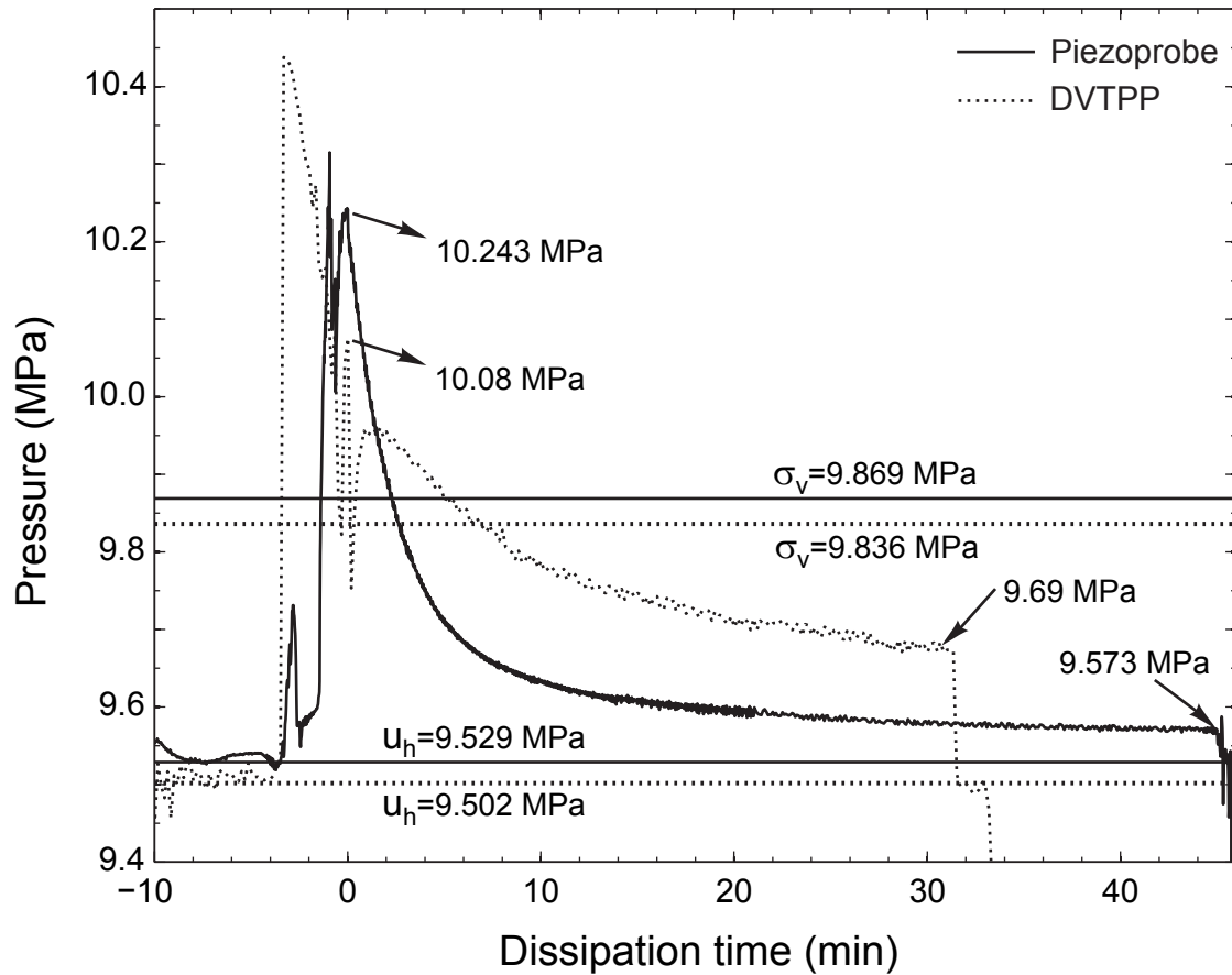
Figure 1.4: Corrected pressure records for DVTPP (dashed line) and Piezoprobe (solid line). The second pressure peak was selected as the initial pressure for both tools and the Dissipation Time is set to zero at this point. Hydrostatic pressure ( u_h ) and overburden stress ( \sigma_v ) are shown at the deployment depth of each tool (dotted = DVTPP, solid = Piezoprobe). They differ slightly for the two deployments because the Piezoprobe was deployed at a slightly deeper depth than the DVTPP. Appendix 1.A describes how these data were corrected.
