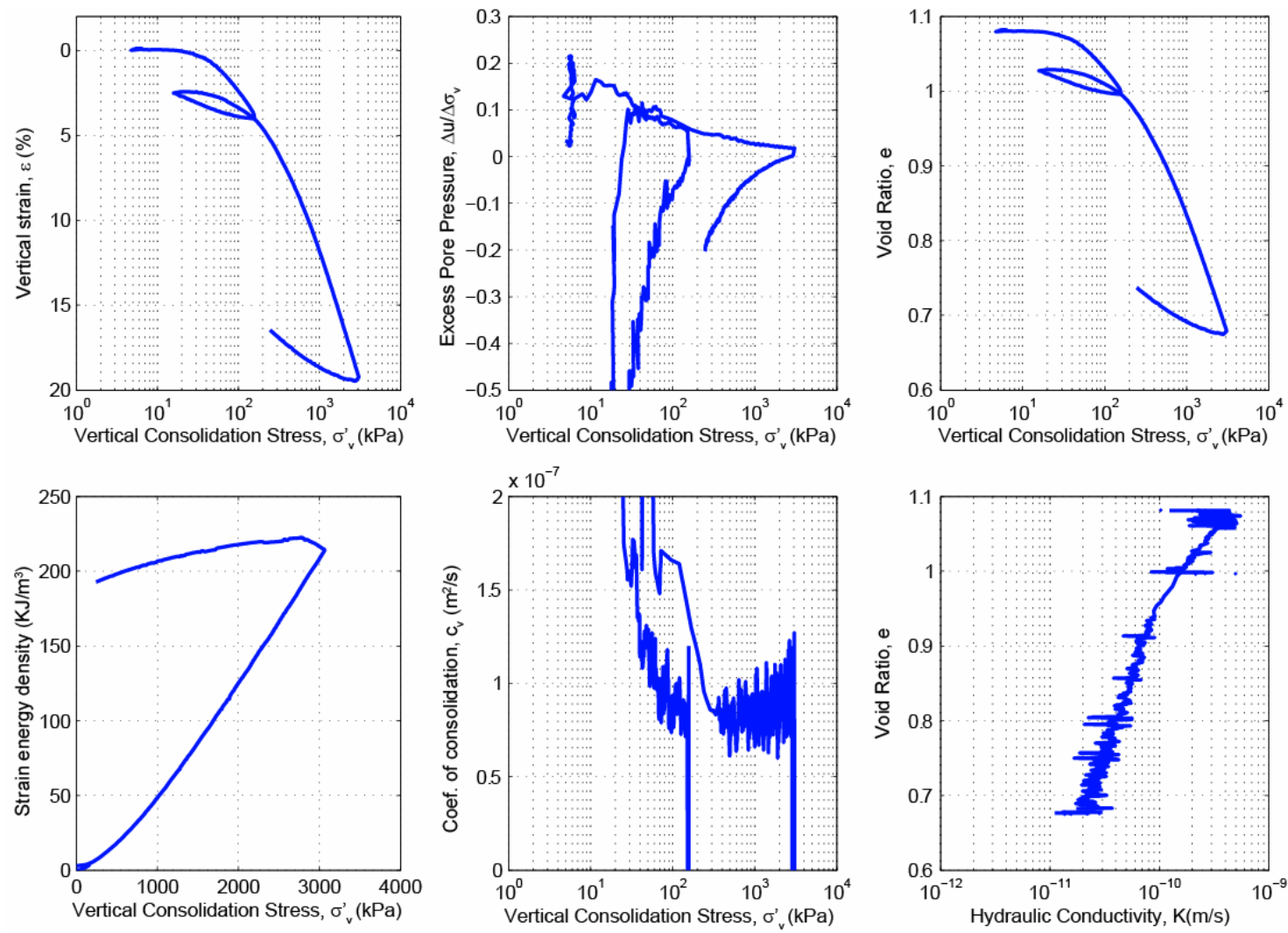
Figure B.11: CRS808 consolidation data for Sample U1322B-15H-1WR, 126.28 mbsf.
