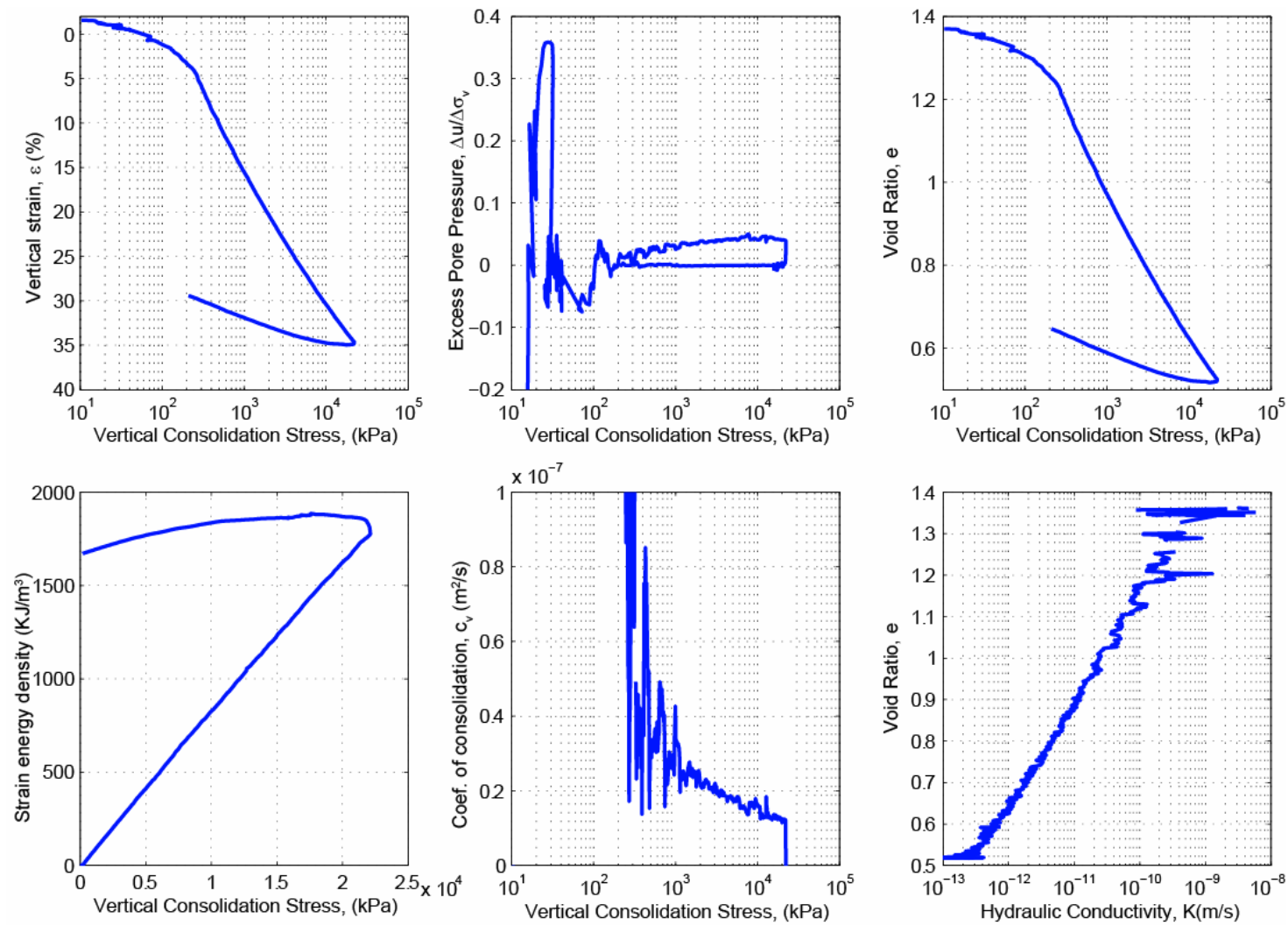
Figure B.20: CRS003 consolidation data for Sample U1324C-1H-1WR, 51.21 mbsf.
