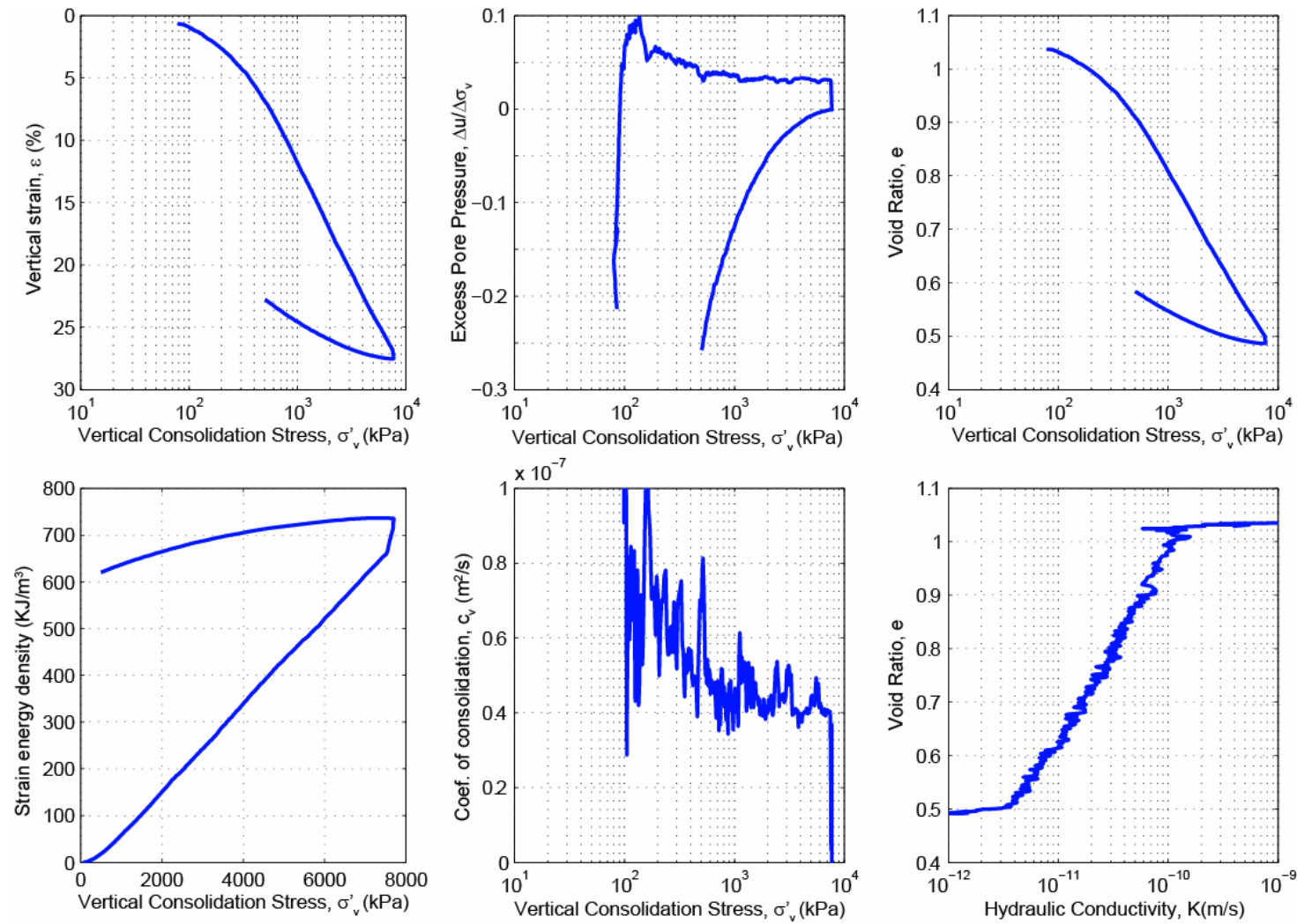
Figure B.22: CRS005 consolidation data for Sample U1324B-13H-7WR, 117.4 mbsf.
