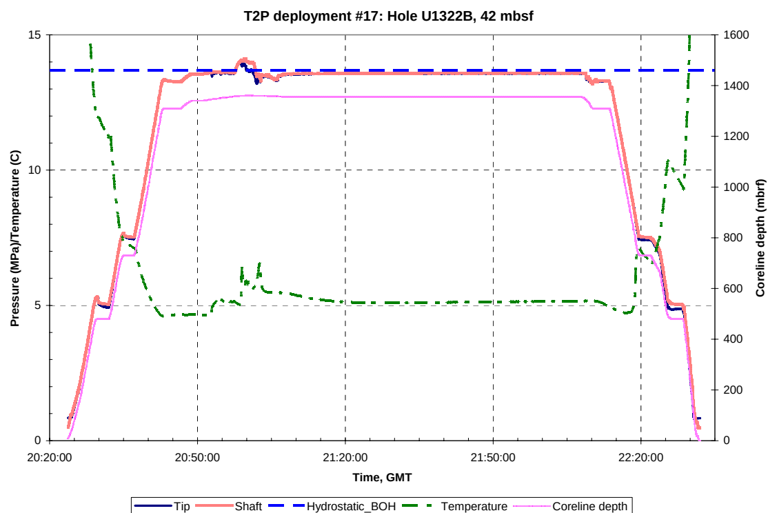
Figure A.B.23.a: Pressure, temperature and Truview data for T2P deployment #17, Hole U1322B, 42 mbsf. GMT = Greenwich Mean Time, Hydrostatic_BOH is the hydrostatic pressure at the bottom of the hole.
