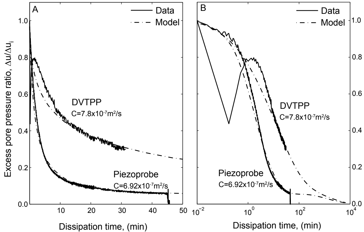
Figure 1.14: Predicted and measured excess pore pressure ratio vs. time for A) linear time and B) log time. For the Piezoprobe, we assume the in situ pressure is equal to the pore pressure estimated using the “bench” behavior. For DVTPP, the in situ pressure is calculated by assuming the same overpressure ratio as inferred at the Piezoprobe location. Based on the best fit between the model prediction and the observed data we find a coefficient of consolidation of 6.92 \times 10^{-7} \text{ m}^2/\text{s} for the Piezoprobe data and 7.8 \times 10^{-7} \text{ m}^2/\text{s} for the DVTPP data.
