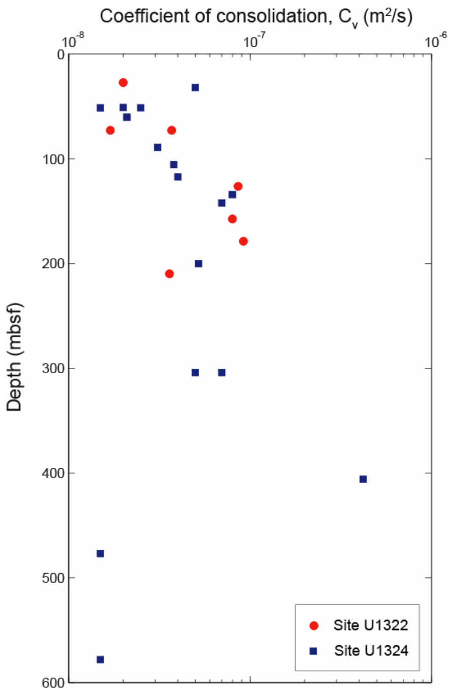
Figure B.28: Coefficient of consolidation for Ursa sediments (Table B.3, columns 2 and 9).
