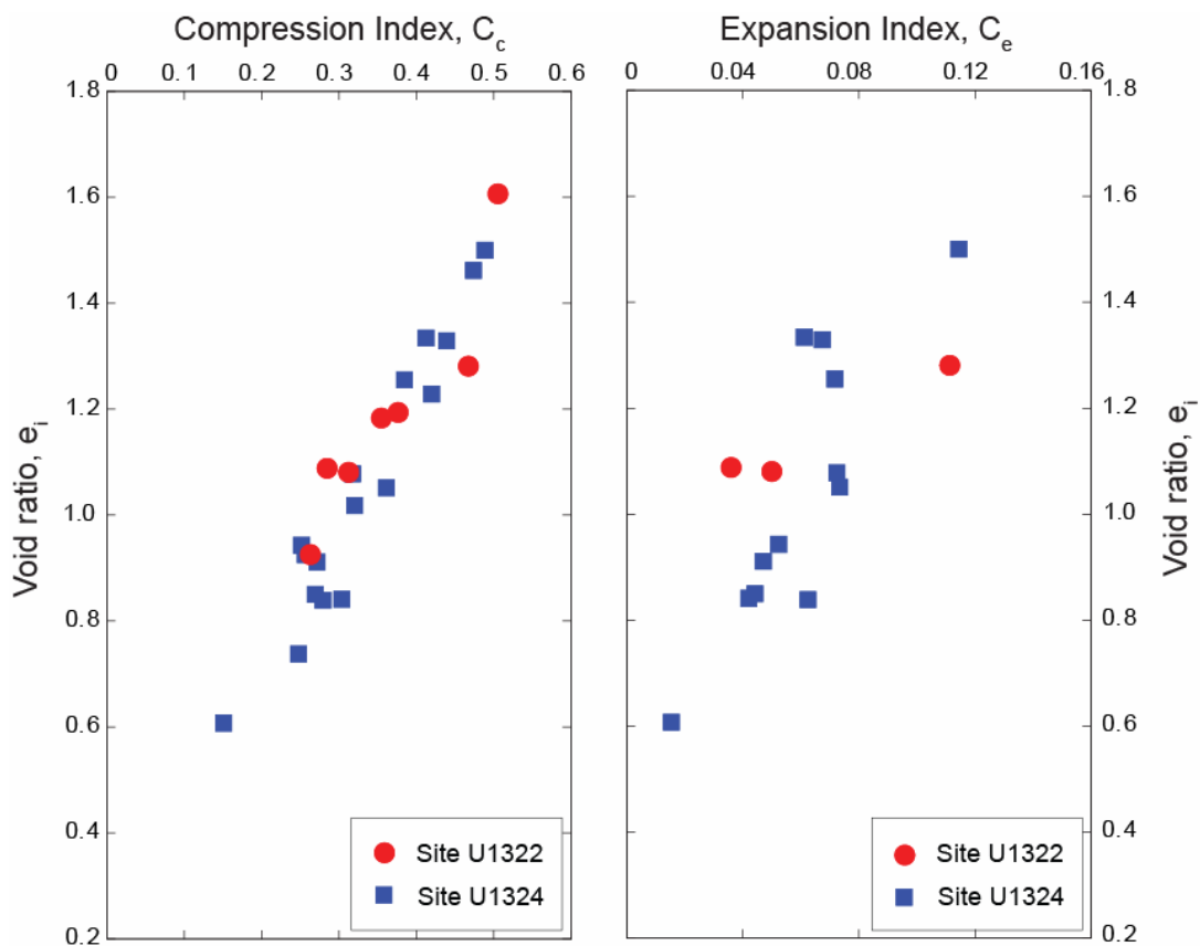
Figure B.26: Compression and expansion indices for Ursa sediments (Table B.3, columns 3 and 8).
