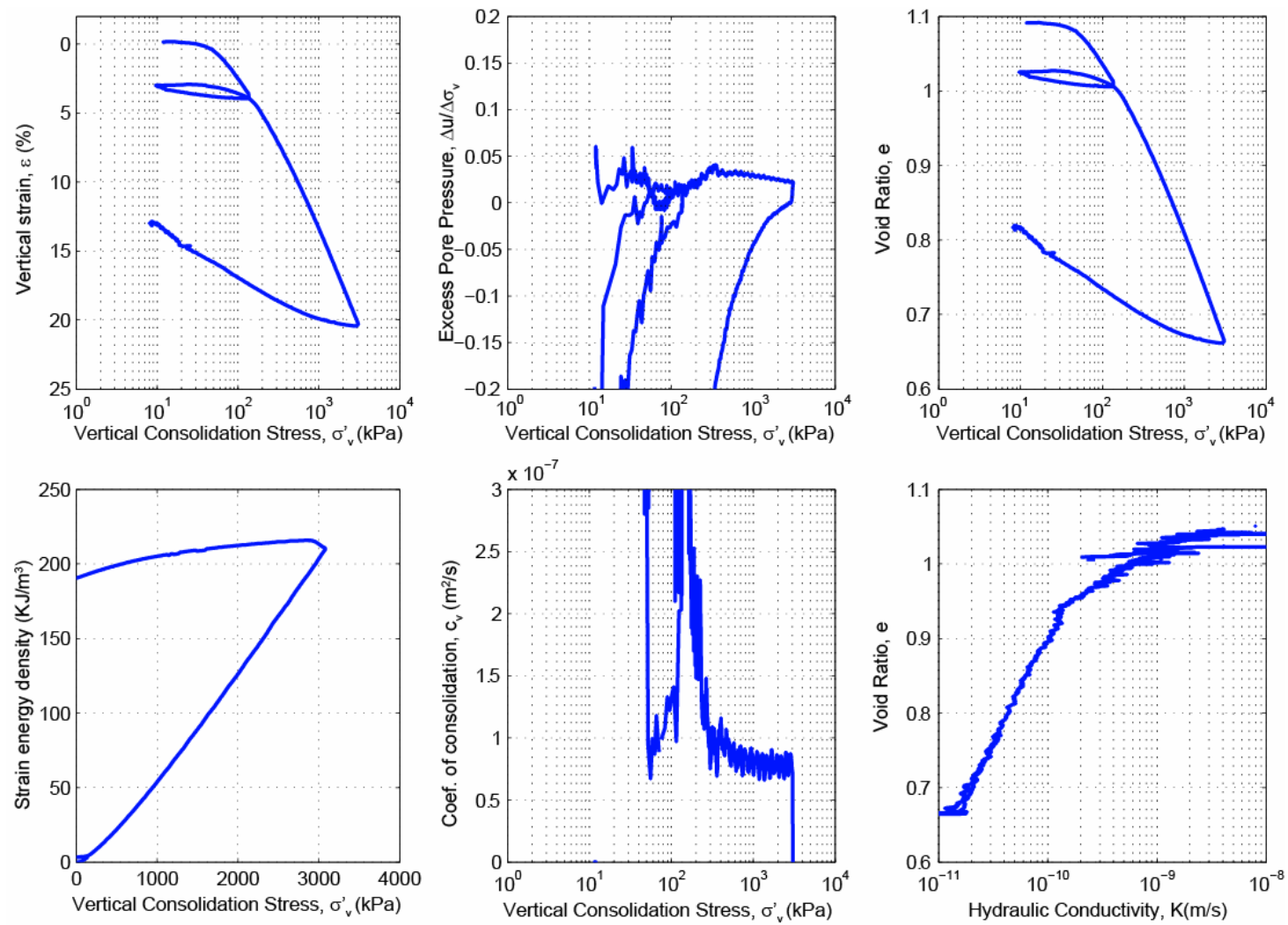
Figure B.12: CRS810 consolidation data for Sample U1322B-18H-6WR, 157.42 mbsf.
