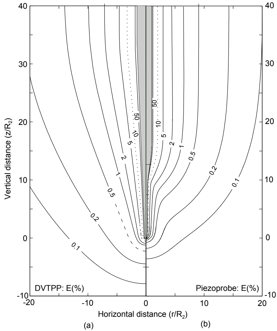
Figure 1.9: Octahedral shear strain ( E ) around the DVTPP (left) and the Piezoprobe (right). The zone of high shear strains, E > 10\% , is confined to a thin annular zone similar in radius to the probe itself. There is much greater shear strain around the DVTPP tip than the Piezoprobe tip at equivalent radial distances. The shapes of the small strain contours ( E < 0.1\% ) show no significant similarity to probe geometry. The coordinates ( r, z ) are normalized by the radius of the shaft of the Piezoprobe ( R_2 ).
