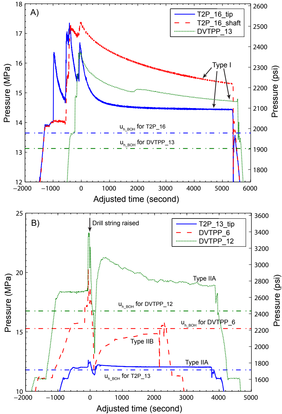
Figure 2.5: Pressure records for the DVTTP and the T2P. Zero time is marked at the start of the dissipation phase of the deployment. Time is plotted in seconds. Hydrostatic pressure at the bottom of the hole (BOH) is calculated assuming a seawater density of 1.024 g/cc. A) Type I deployments with type pressure dissipation curves. B) Type II deployments: pressure drops rapidly due to tool dislodgement, after rebounds to certain level, pressure decays towards formation pressure (Type IIA); pressure drops rapidly due to tool dislodgement and then
