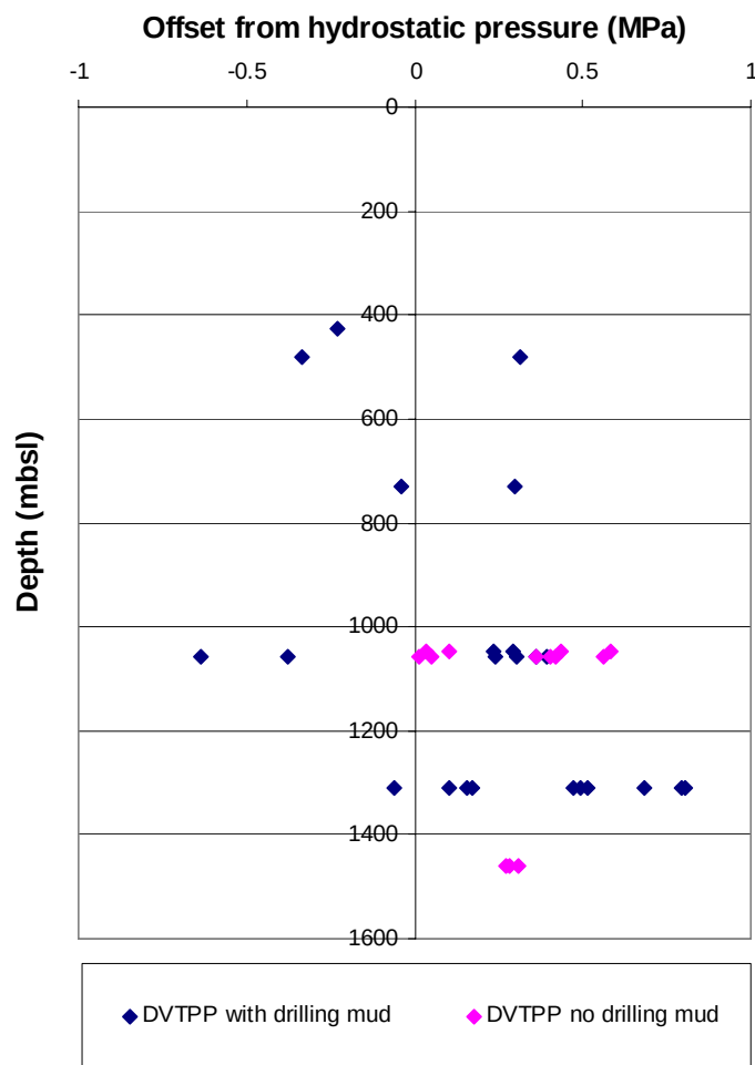
Figure A.C.1 : Offset between the tool pressure and the hydrostatic pressure for tool stops at or above the seafloor. The hydrostatic pressure was calculated assuming a seawater density of 1.024 g/cc.
