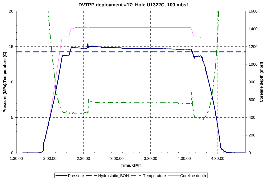
Figure A.A.16.a: Pressure, temperature and Truview data for DVTPP Deployment #17, Hole U1322C, 100 mbsf. GMT = Greenwich Mean Time, Hydrostatic_BOH is the hydrostatic pressure at the bottom of the hole.
