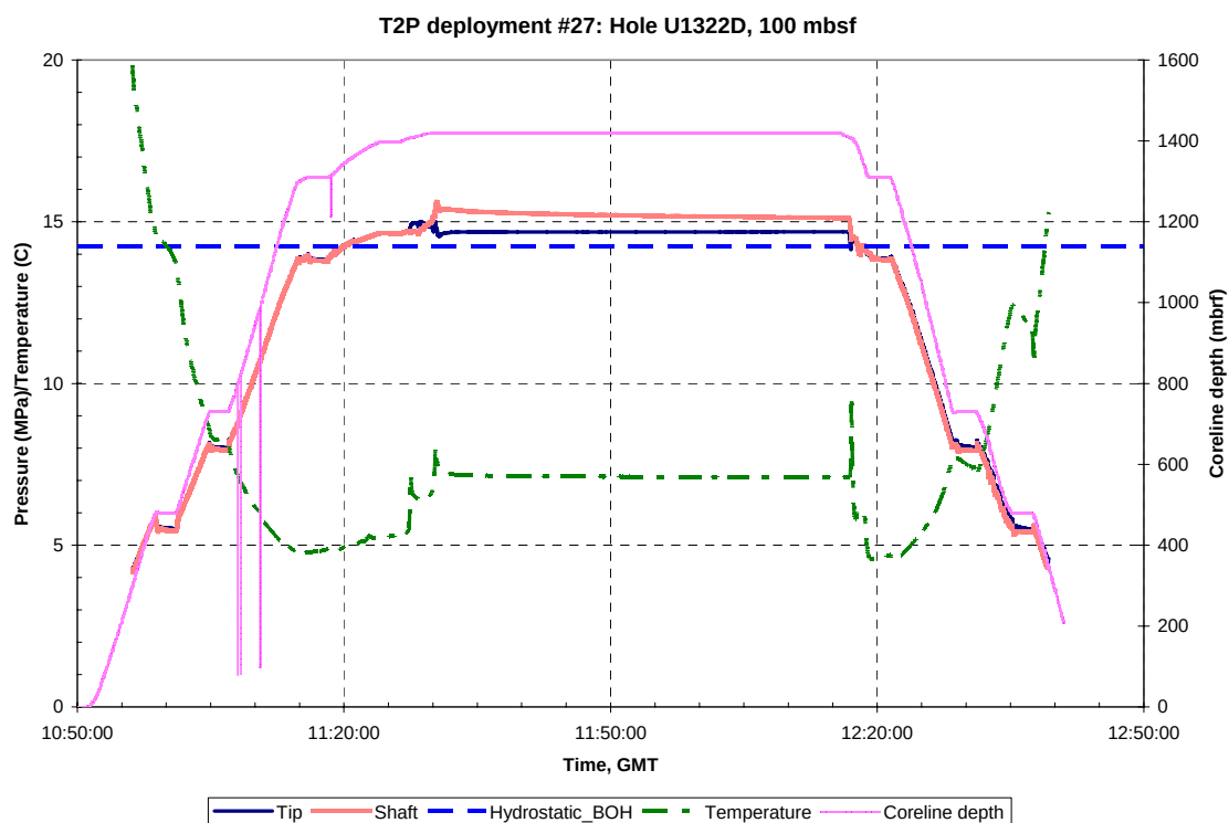
Figure A.B.30.a: Pressure, temperature and Truview data for T2P deployment #27, Hole U1322D, 100 mbsf. GMT = Greenwich Mean Time, Hydrostatic_BOH is the hydrostatic pressure at the bottom of the hole.
