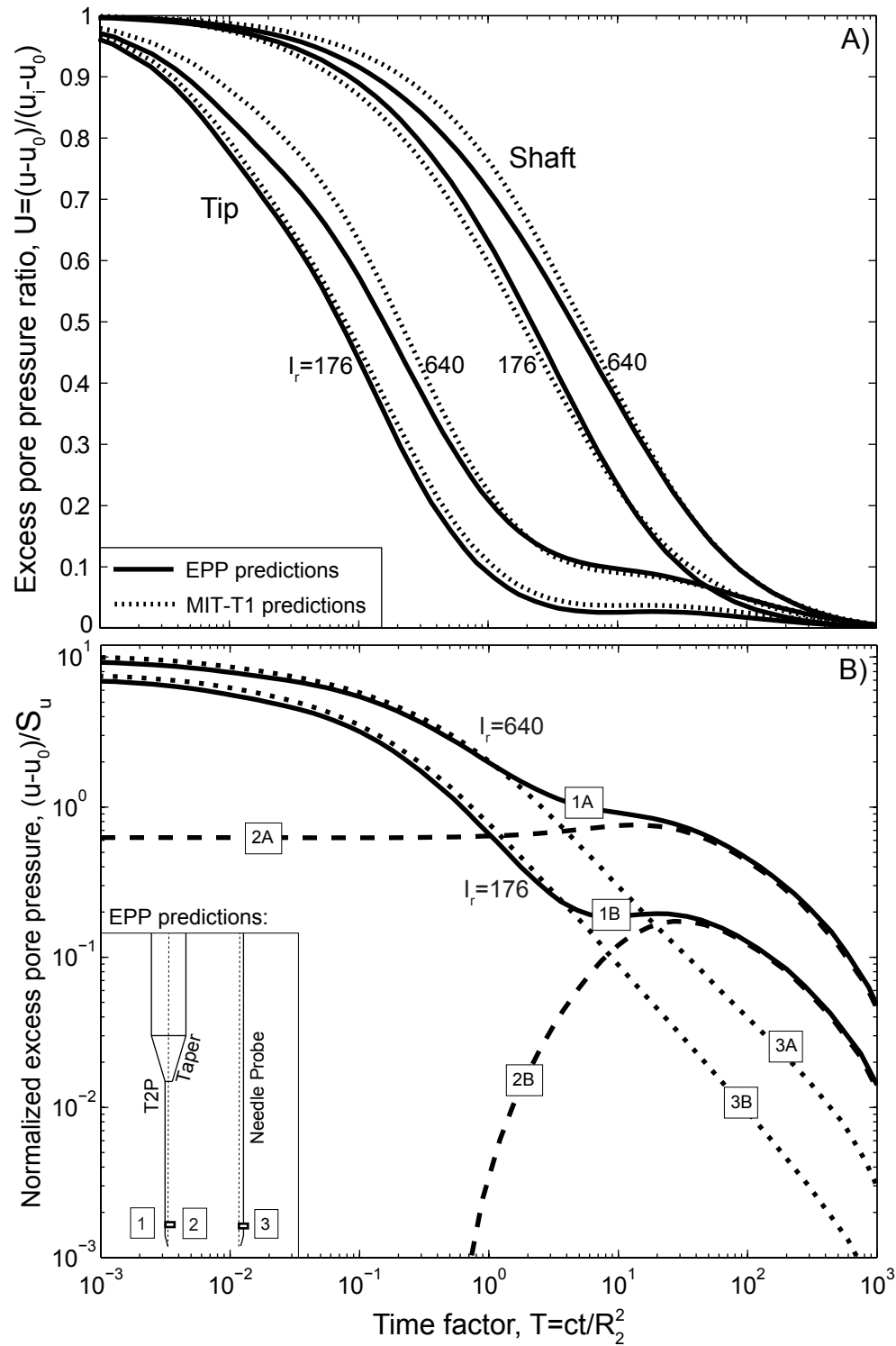
Figure 3.6: Pore pressure dissipation for soils with different I_r . A) Excess pore pressure ratio ( U ) plotted against time factor T . Solid lines represent the EPP model predictions and dotted lines represent the MIT-T1 predictions. B) Normalized excess pore pressure plotted against time factor T for EPP model predictions. Line #1A and Line #1B (solid line) record the dissipation response at tip of the T2P for I_r = 176 and 640 , respectively. Line #2A and Line #2B (dashed line) record the dissipation response of the overlying tapered shaft at location 2 (inset figure) for I_r = 176 and 640 , respectively. Line #3A and #3B (dotted line) is the dissipation response of a constant diameter needle probe ( R = 3.2 mm), for I_r = 176 and 640 , respectively. Dissipation at the tip of the tapered probe clearly follows the dissipation response of only the tip geometry in early time.
