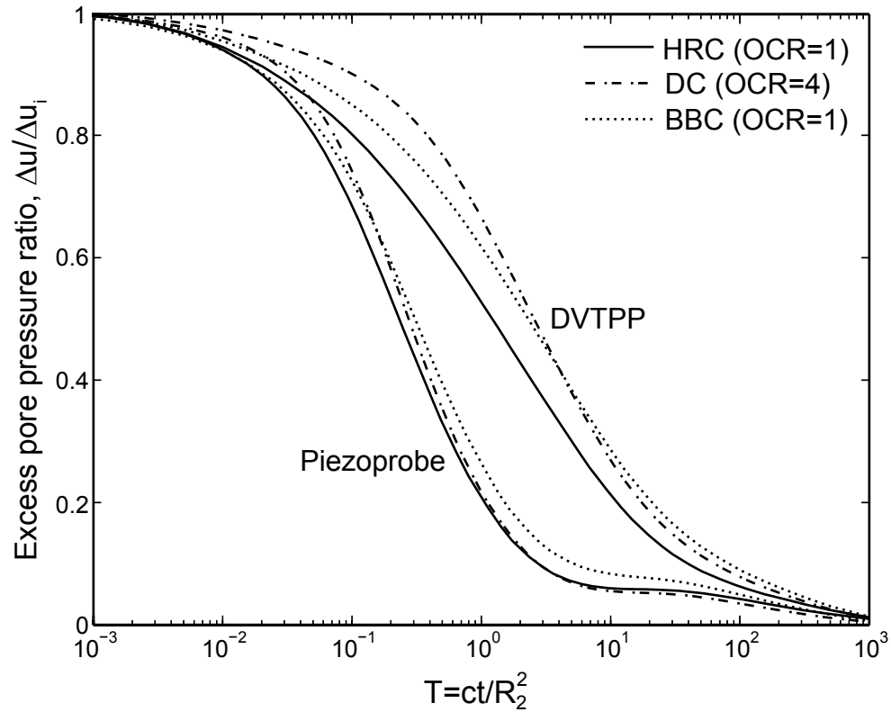
Figure 1.15: Pressure dissipation of the DVTTP and the Piezoprobe for penetration in different soils. HRC = uniaxially normally consolidated resedimented Hydrate Ridge Clay (also illustrated in Figure 1.12 and 1.14). DC=uniaxially over-consolidated ( K_o ) Drammen Clay [Prévost, 1978]. BBC = uniaxially normally consolidated ( K_o ) Boston Blue Clay [Levadoux and Baligh, 1980]. (OCR= Over Consolidation Ratio).
