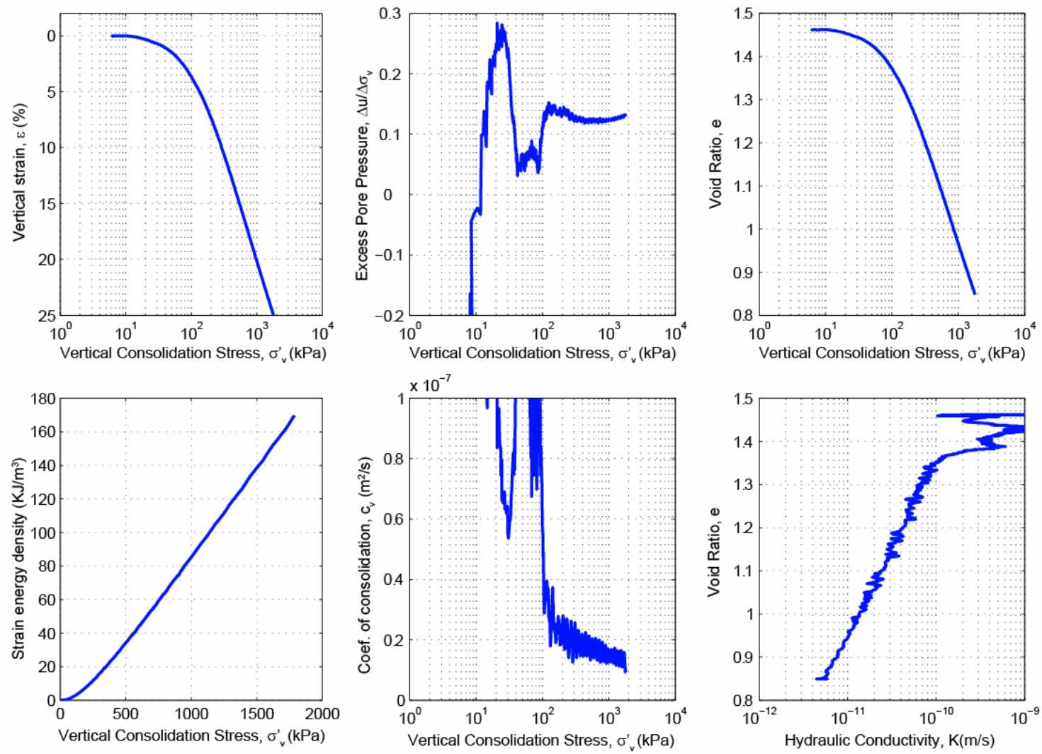
Figure B.5: CRS799 consolidation data for Sample U1324C-1H-1WR, 51.31 mbsf.
