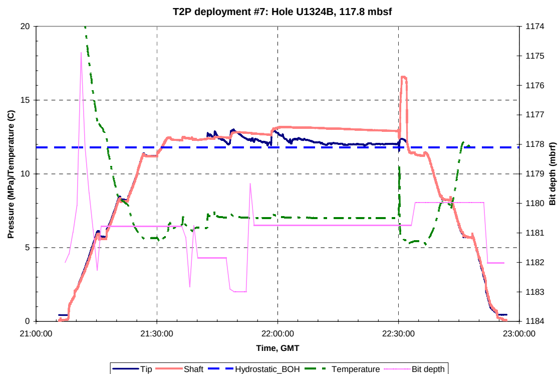
Figure A.B.14.b: Pressure, temperature and Truview data for T2P deployment #7, Hole U1324B, 117.8 mbsf. GMT = Greenwich Mean Time, Hydrostatic_BOH is the hydrostatic pressure at the bottom of the hole
