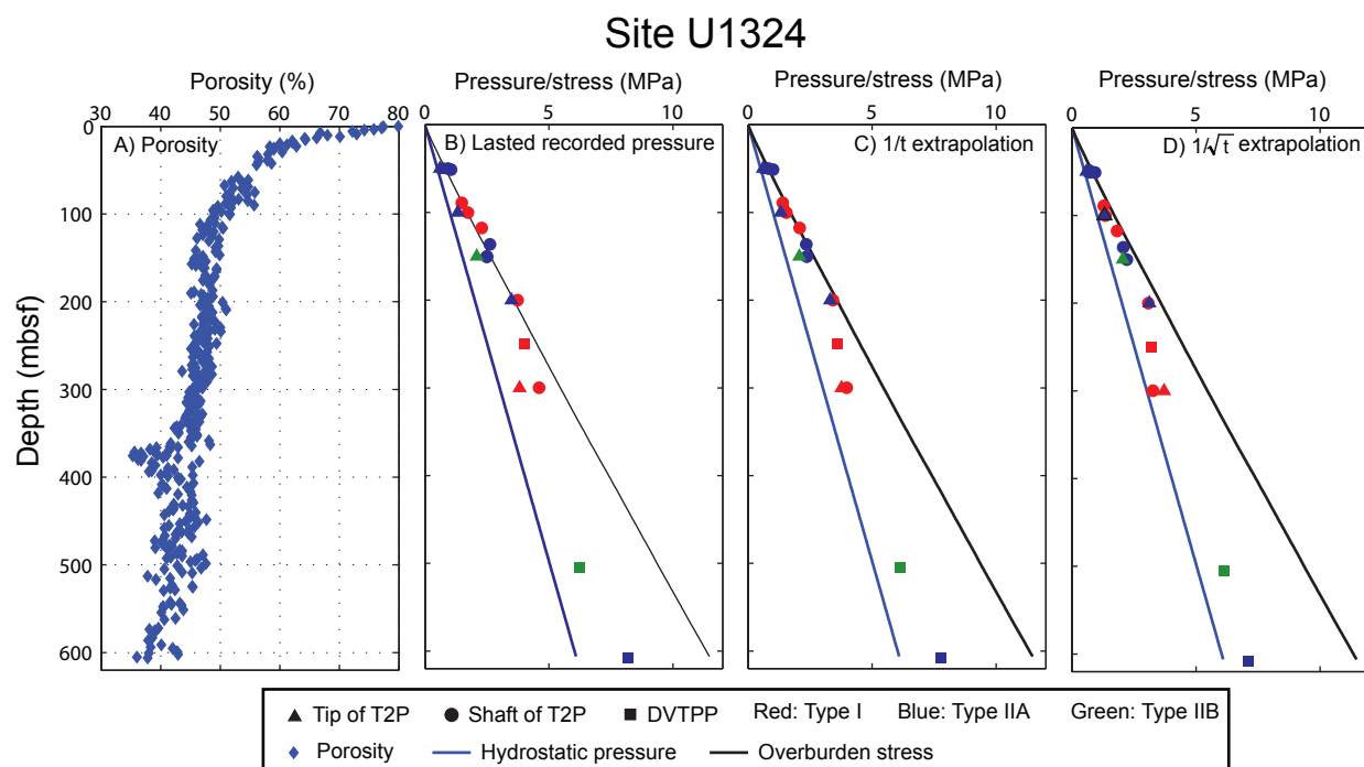
Figure A.13: Pore pressure measurements at Site U1324. The hydrostatic pressure is calculated starting from the seafloor assuming a seawater density of 1.024 g/cc. Bulk density data from shipboard Moisture and Density measurements (MAD) were integrated to calculate the overburden stress. The static pressure due to the water column above seafloor was subtracted from the pressure results. A) Porosity obtained from shipboard moisture and density (MAD) measurement. B) Last recorded pressure of the penetrometer (Table A.2, column 8). C) In situ pore pressure estimated by 1/t extrapolation (Table A.2, column 9). D) In situ pore pressure estimated by 1/\sqrt{t} extrapolation (Table A.2, column 10).
