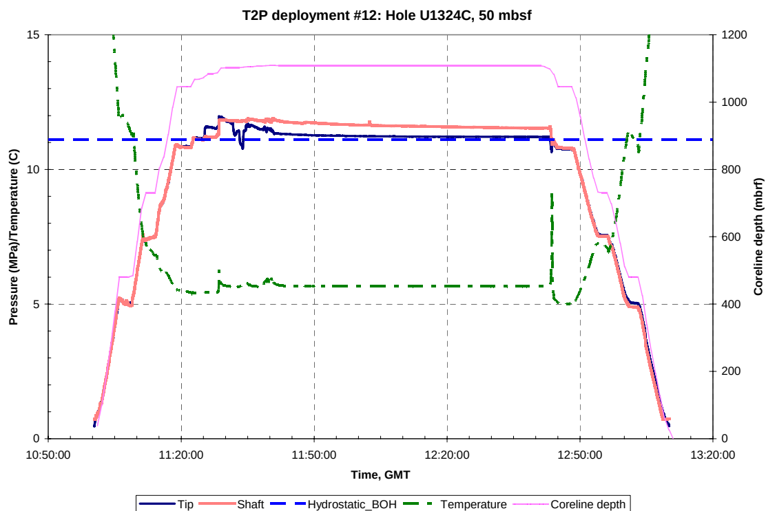
Figure A.B.18.a: Pressure, temperature and Truview data for T2P deployment #12, Hole U1324C, 50 mbsf. GMT = Greenwich Mean Time, Hydrostatic_BOH is the hydrostatic pressure at the bottom of the hole.
