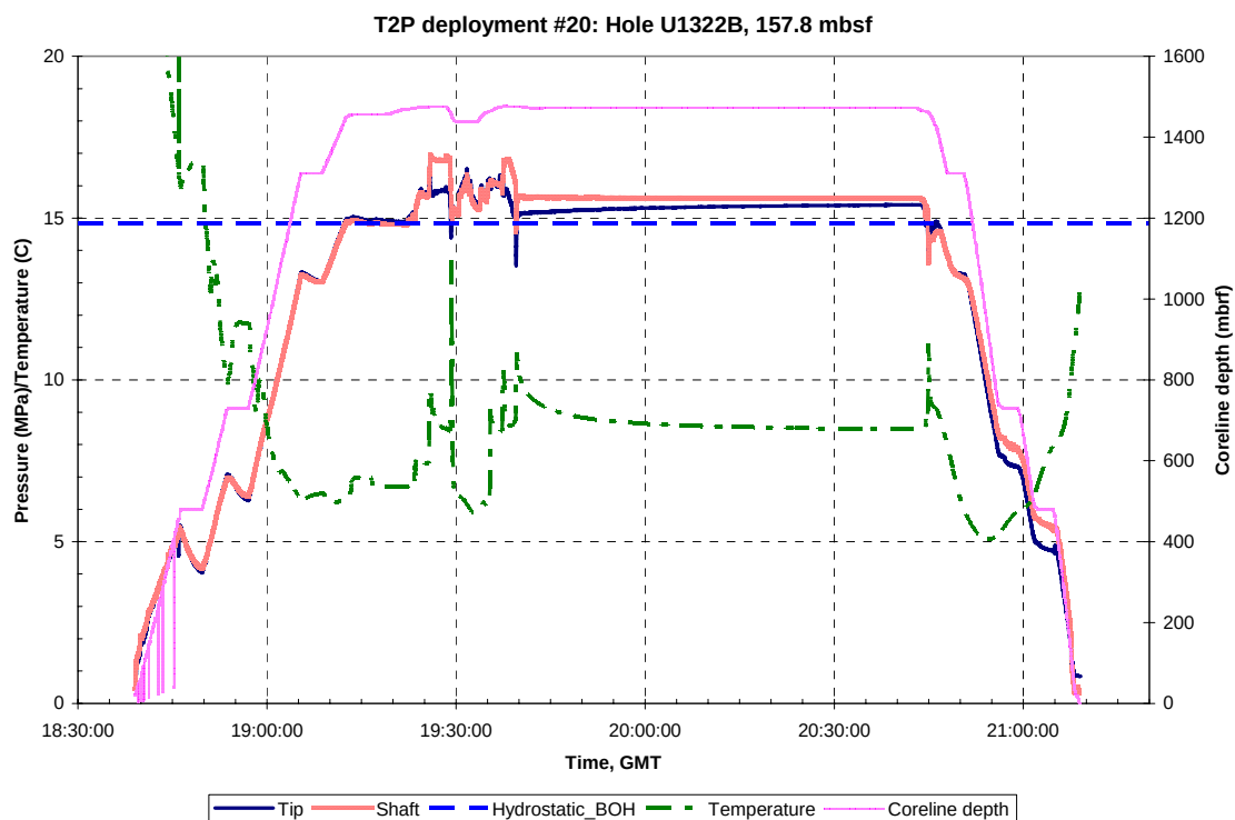
Figure A.B.25.a: Pressure, temperature and Truview data for T2P deployment #20, Hole U1322B, 157.8 mbsf. GMT = Greenwich Mean Time, Hydrostatic_BOH is the hydrostatic pressure at the bottom of the hole.
