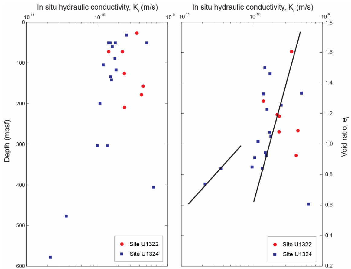
Figure B.27: In situ hydraulic conductivity for Ursa sediments (Table B.3, columns 2, 3 and 9).
