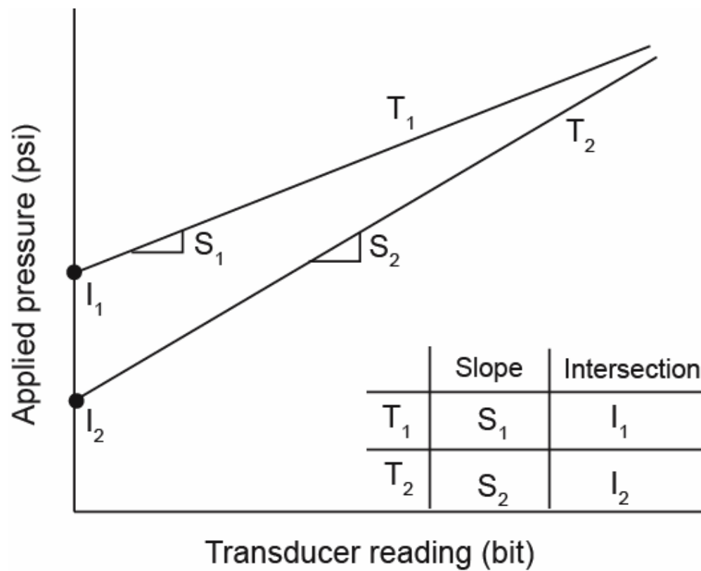
Figure A.B.2: Influence of temperature on T2P pressure transducers. The slope and intersection of the calibration curve can change with temperature.
