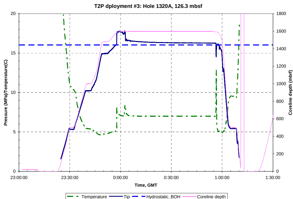
Figure A.B.10.a: Pressure, temperature and Truview data for T2P deployment #3, Hole U1320A, 126.3 mbsf. GMT = Greenwich Mean Time, Hydrostatic_BOH is the hydrostatic pressure at the bottom of the hole.
