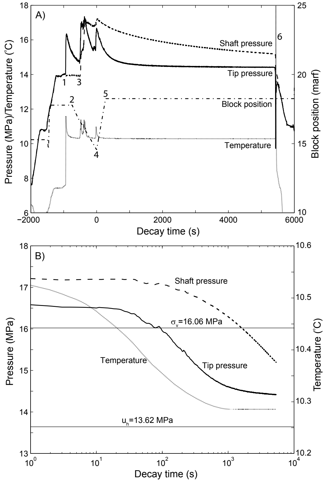
Figure 3.3: Penetration and dissipation phase of T2P deployment #16. Zero time is marked at the start of the dissipation phase of the deployment. Time is plotted in seconds. The traveling block is attached to the top end of the drill string above the rig floor. Its position was recorded in meter above rig floor (marf), which illustrates movements of the drill bit during tool deployment.
