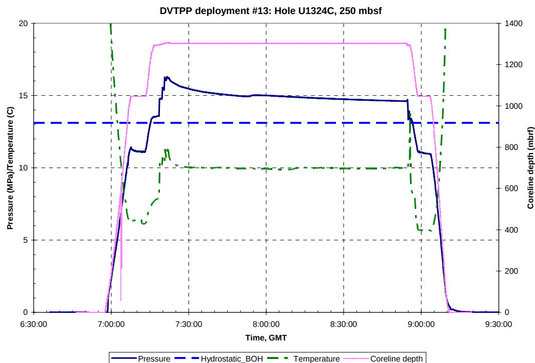
Figure A.A.12.a: Pressure, temperature and Truview data for DVTPP Deployment #13, Hole U1324C, 250 mbsf. GMT = Greenwich Mean Time, Hydrostatic_BOH is the hydrostatic pressure at the bottom of the hole.
