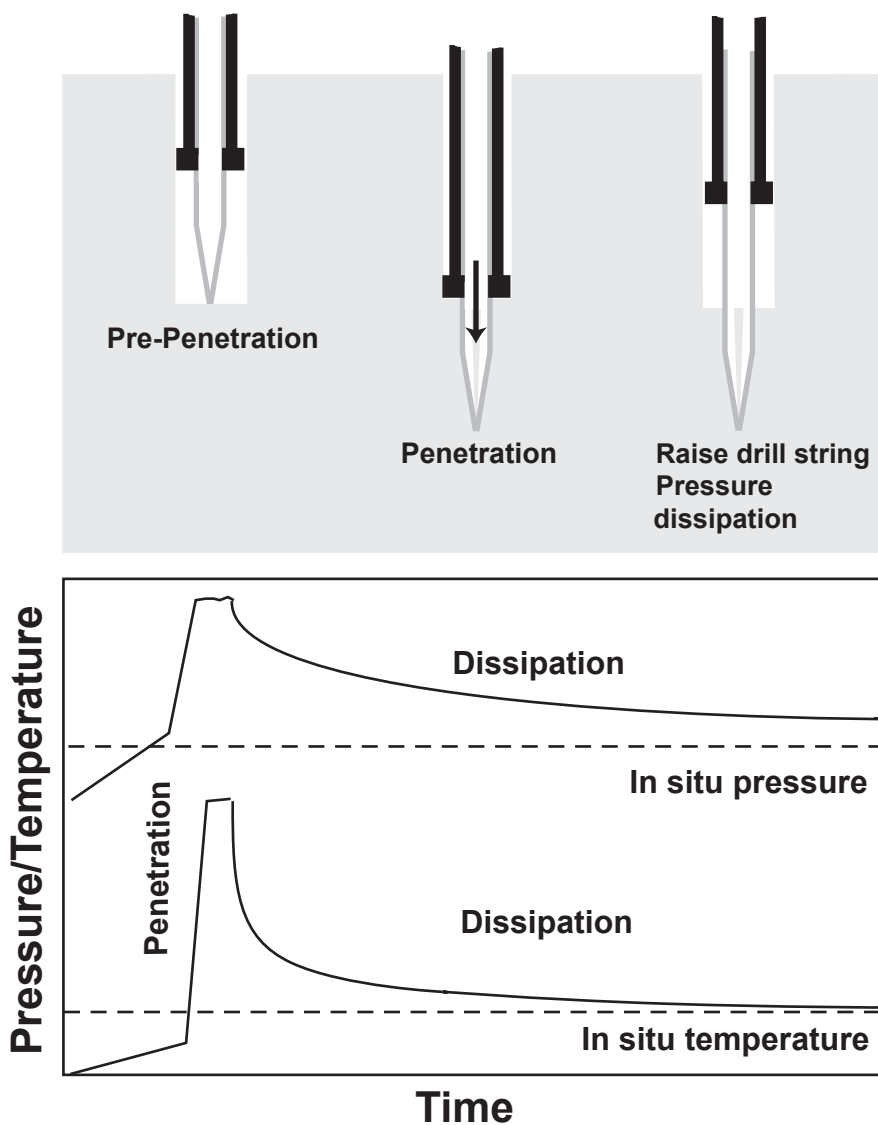
Figure A.5: Illustration of the procedure for probe penetration. The drill string pushes the probe into the formation. After penetration, the drill string is raised and the CDS telescopes to decouple the drill string from the tool. The probe stays in the formation to monitor the temperature and pressure. For a good measurement, there is an abrupt increase in pressure and temperature during penetration and then there is a slow dissipation of pressure and temperature when the tool stays in the formation.
