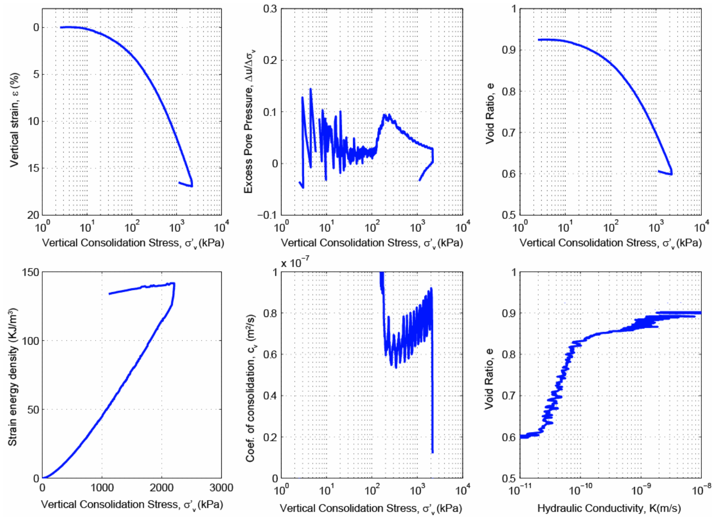
Figure B.7: CRS801 consolidation data for Sample U1324B-16H-5WR, 142.13 mbsf.
