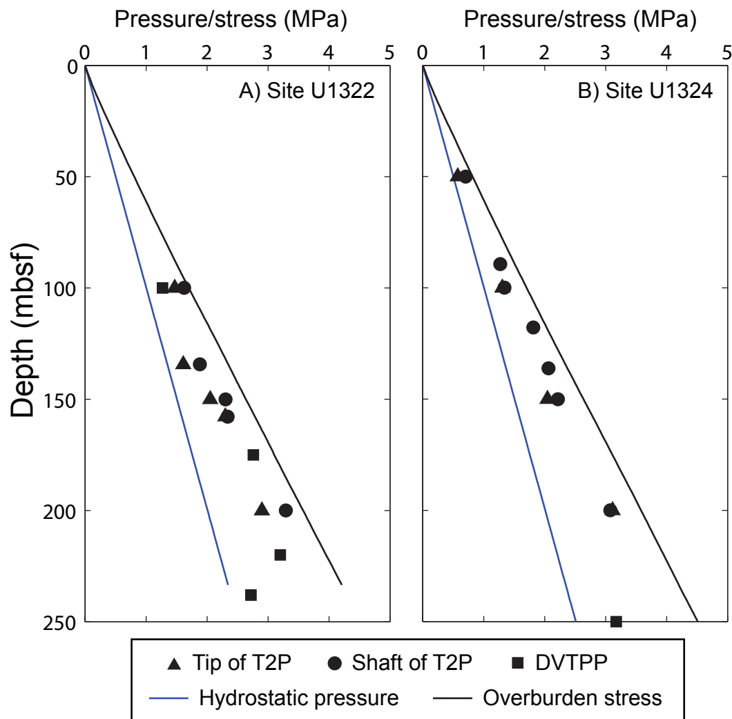
Figure A.14: In situ pressure estimates by 1/\sqrt{t} extrapolation in the upper 250 mbsf at Site U1322 and Site U1324. The hydrostatic pressure is calculated starting from the seafloor assuming a seawater density of 1.024 g/cc. Bulk density data from shipboard Moisture and Density measurements (MAD) were integrated to calculate the overburden stress. The static pressure due to the water column above seafloor was subtracted from the pressure results.
