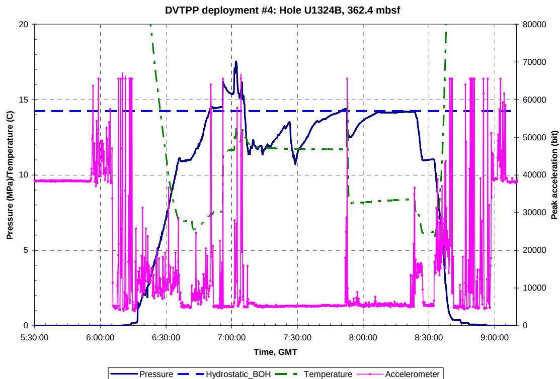
Figure A.A.5: Pressure, temperature and acceleration data for DVTPP Deployment #4, Hole U1324B, 362.4 mbsf. GMT = Greenwich Mean Time, Hydrostatic_BOH is the hydrostatic pressure at the bottom of the hole.
