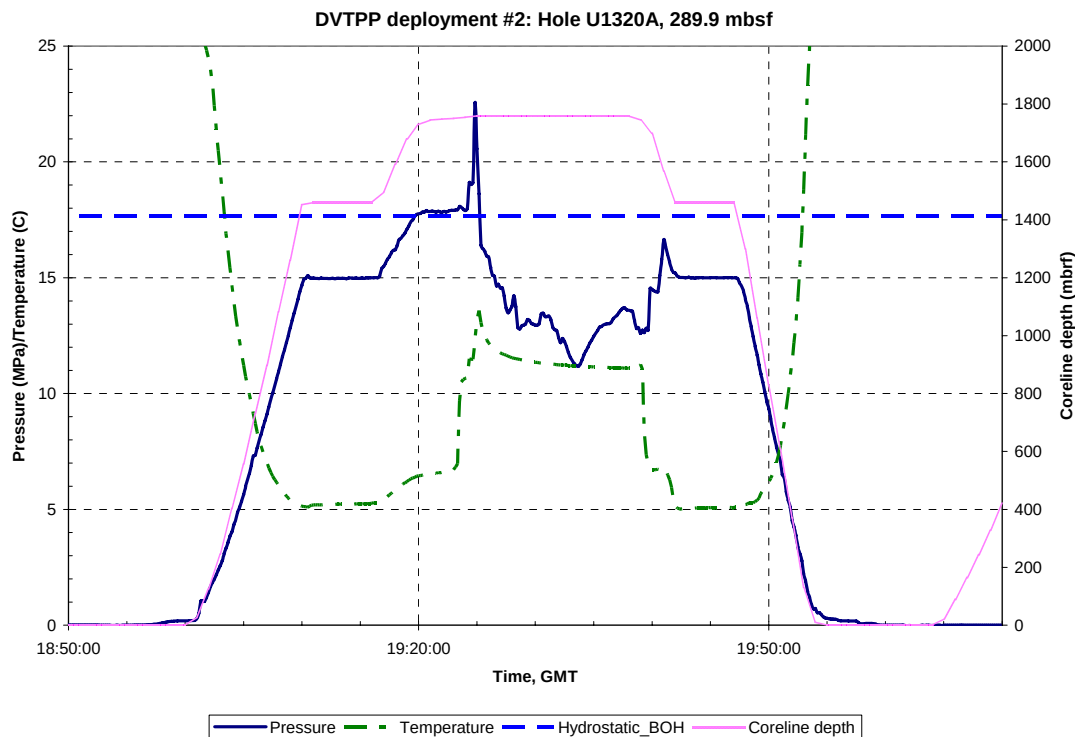
Figure A.A.3.a: Pressure, temperature and Truview data for DVTPP Deployment #2, Hole U1320A, 289.9 mbsf. GMT = Greenwich Mean Time, Hydrostatic_BOH is the hydrostatic pressure at the bottom of the hole.
