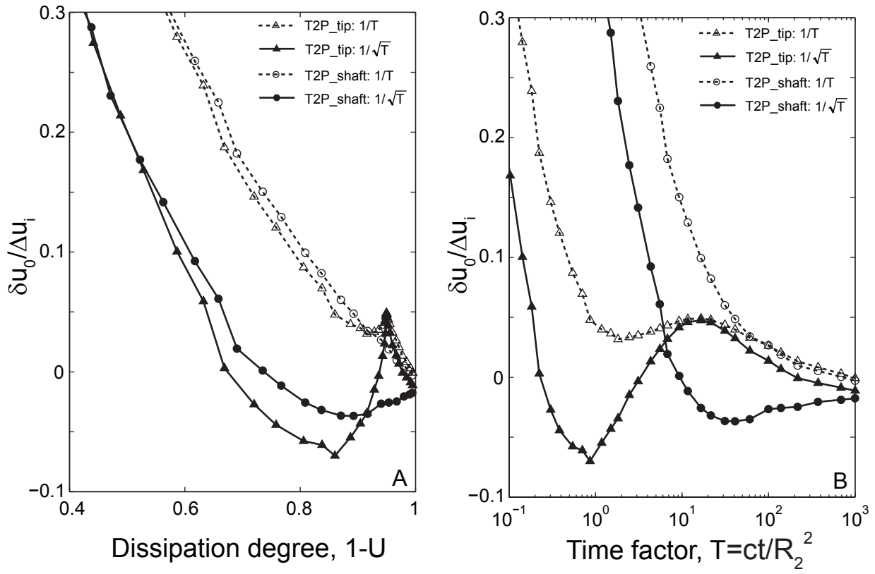
Figure 3.18: Theoretical prediction of errors in estimating u_0 by 1/t and 1/\sqrt{t} extrapolations. Full MIT-T1 predictions for the Ursa clay are used (Figure 3.8). A) Errors as a function of dissipation degree. B) Error as a function of dissipation time factor ( T ).
