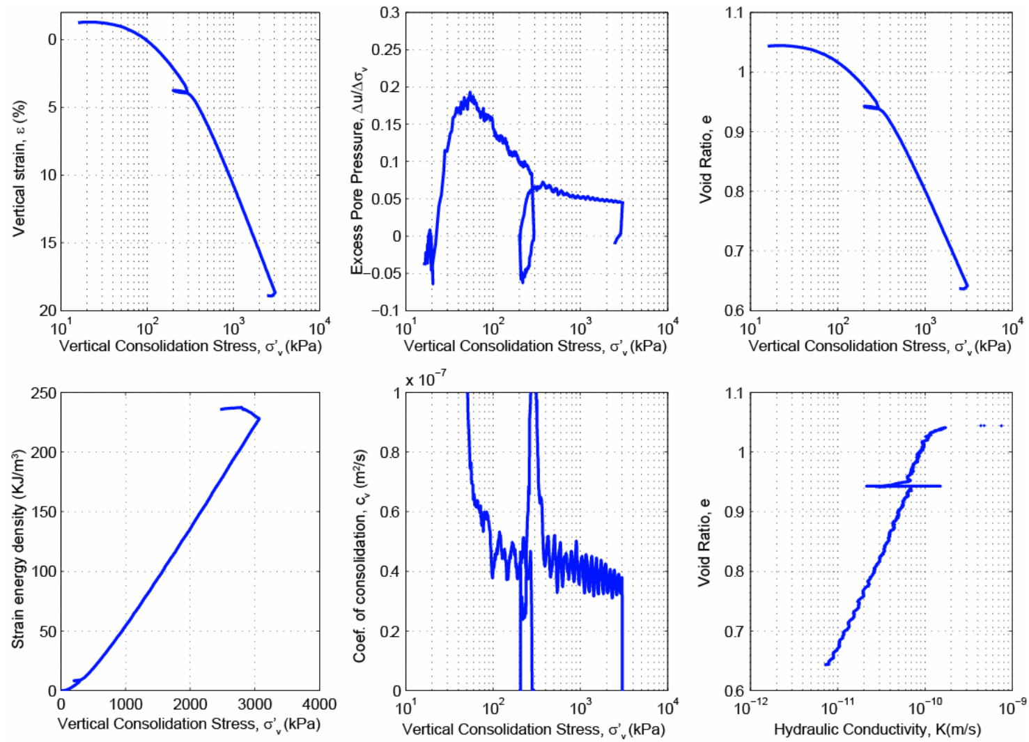
Figure B.10: CRS807 consolidation data for Sample U1324C-2H-4WR, 105.48 mbsf.
