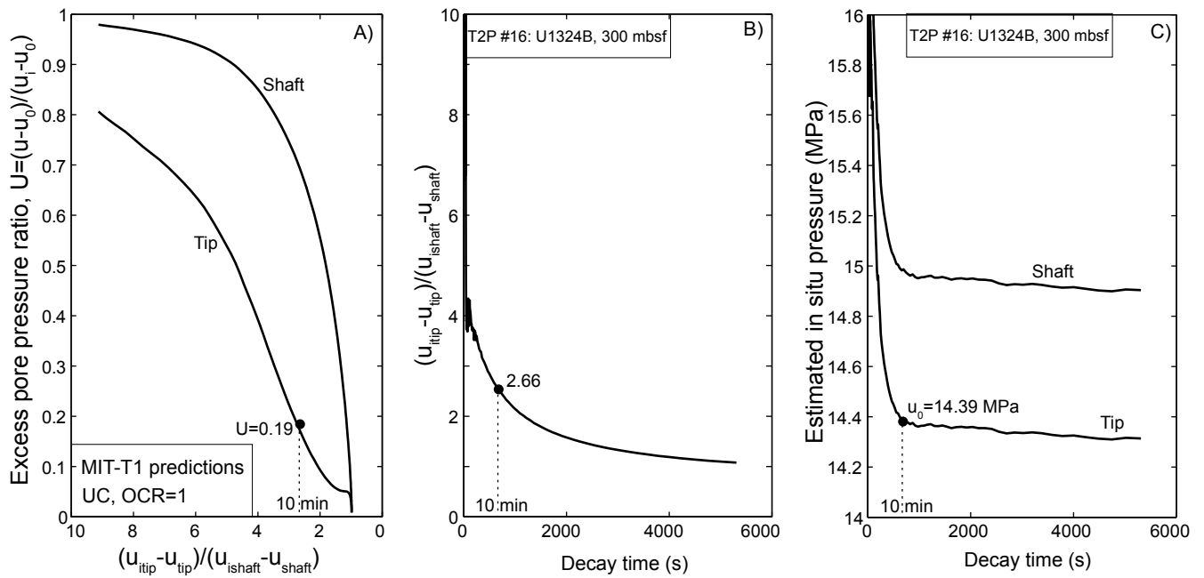
Figure 3.13: Estimating in situ pressure from the ratio of dissipated pressures at the tip and shaft pressure ports. A) Excess Pore Pressure ( U ) vs. the ratio of the total dissipation at the tip and the shaft. These results are derived directly from the full MIT-T1 model for the Ursa Clay (Figure 3.10, solid line). As time increases, the excess pore pressure declines and the fractional dissipation becomes equal at the tip and shaft. B) The ratio of total dissipation at the tip and shaft vs. time for T2P deployment 16. C) Estimated in situ pressure calculated from Equation 3.5.
