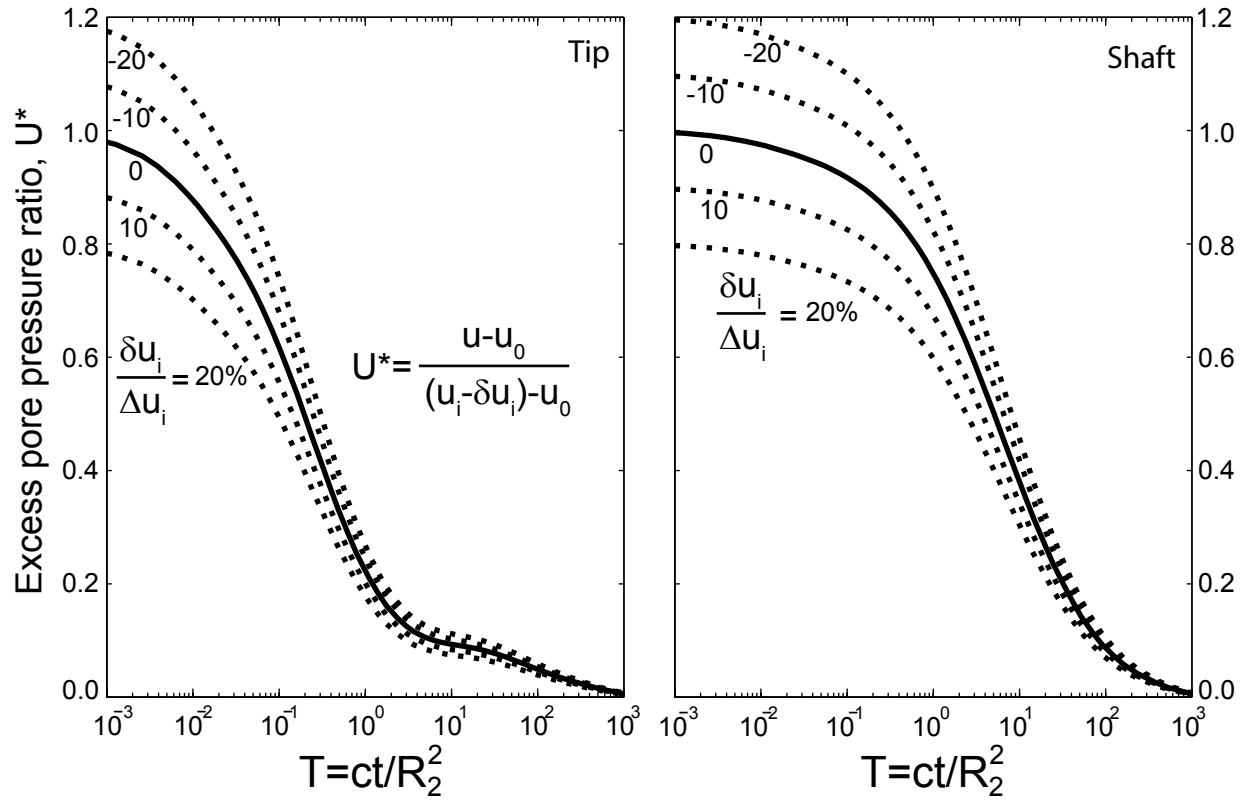
Figure 3.15: Effect of the error in the initial excess pore pressure on the dissipation curve. The solid lines represent modeled behavior by full MIT-T1 soil model for the Boston Blue Clay (Figure 3.10, dotted line). "Apparent" dissipation curves (dotted lines) are given for \delta u_i / \Delta u_i = 20\% , 10, -10 and -20%.
