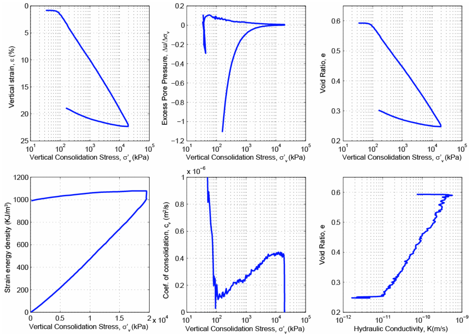
Figure B.25: CRS008 consolidation data for Sample U1324C-7H-1WR, 405.81 mbsf.
