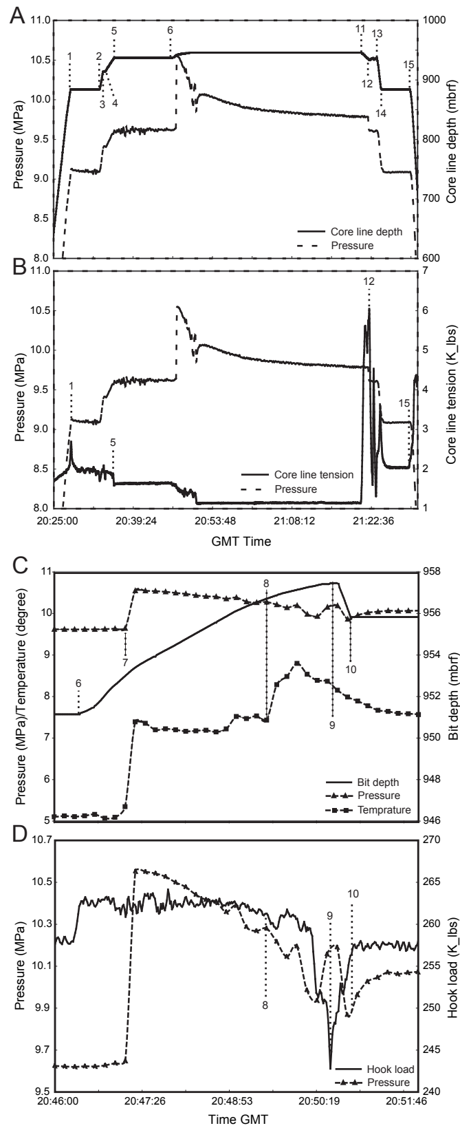
Figure 1.A1: Summary of DVTPP deployment. The deployment events are identified by numbers and are explained in Table 1.2. A) Pressure record and core line depth. B) Pressure record and core line tension. C) Pressure, temperature and bit depth. D) Pressure record and hook load. See
