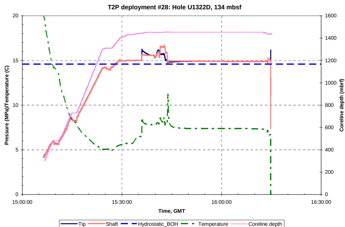
Figure A.B.31.a: Pressure, temperature and Truview data for T2P deployment #28, Hole U1322D, 134 mbsf. GMT = Greenwich Mean Time, Hydrostatic_BOH is the hydrostatic pressure at the bottom of the hole.
