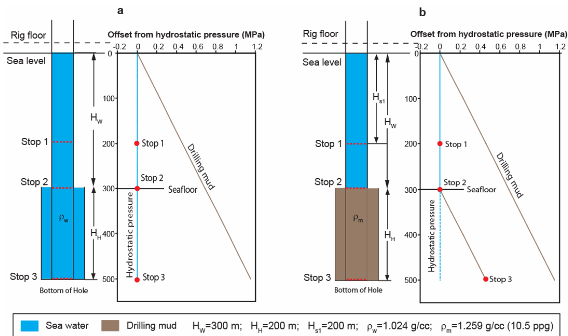
Figure A.C.3 : Two ideal scenarios of fluid condition in drill-pipe. The solid brown line represents the predicted static pressure by assuming the borehole was filled with a 10.5 ppg drilling mud. a) Predicted fluid pressure profile for cases with no drilling mud was used and the seawater was not contaminant with the drilling cuttings. b) Predicted fluid pressure profile for cases with drilling mud was used and the mud elevations inside and outside the pipe are at seafloor.
