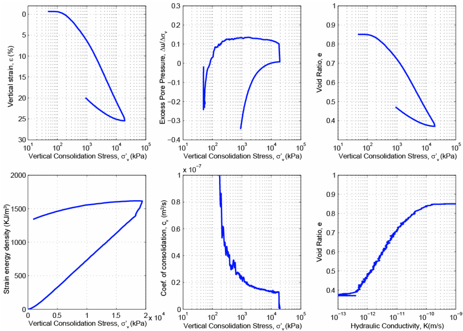
Figure B.24: CRS007 consolidation data for Sample U1324B-60X-2WR, 476.86 mbsf.
