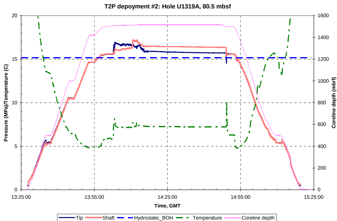
Figure A.B.9.a: Pressure, temperature and Truview data for T2P deployment #2, Hole U1319A, 80.5 mbsf. GMT = Greenwich Mean Time, Hydrostatic_BOH is the hydrostatic pressure at the bottom of the hole.
