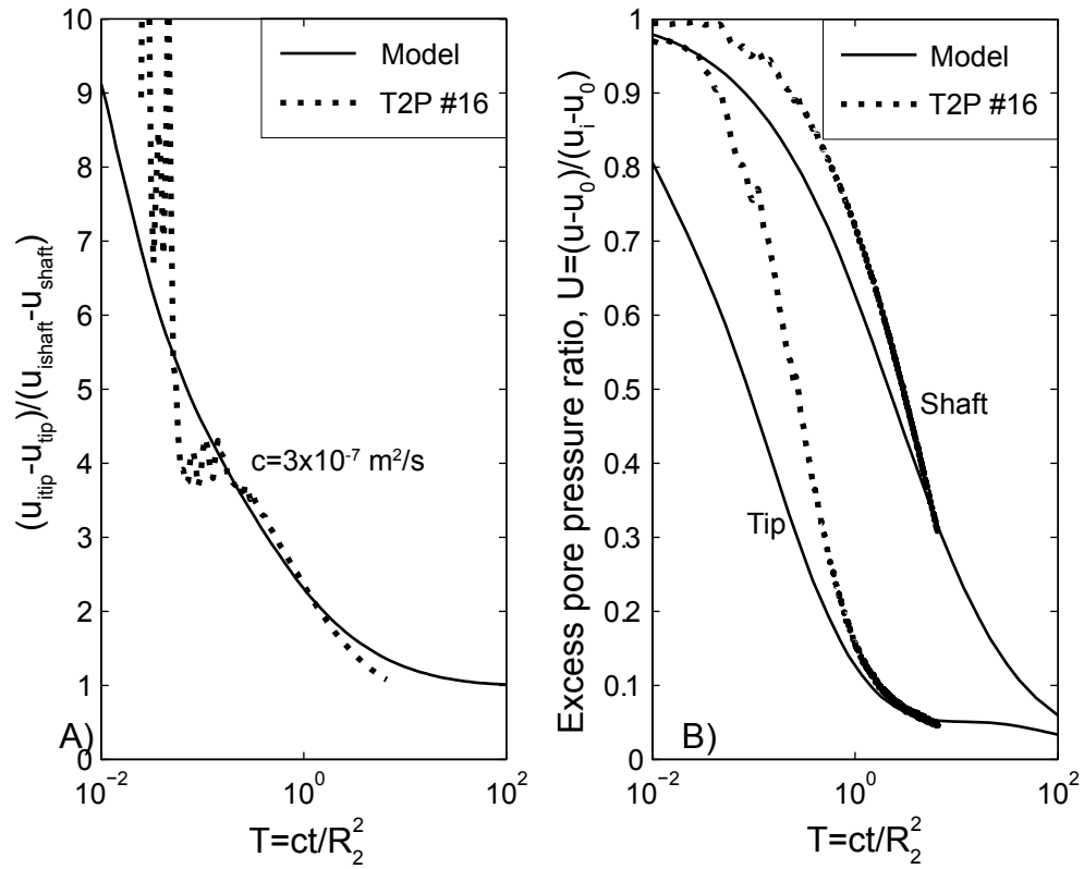
Figure 3.14: Interpretation of hydraulic diffusivity. The solid lines represent modeled behavior by full MIT-T1 soil model for the Ursa Clay (Figure 3.10, solid line). The dotted lines represent the measured data. A) Determining the hydraulic diffusivity by curve matching. B) Comparison of predicted and measured dissipation behavior.
