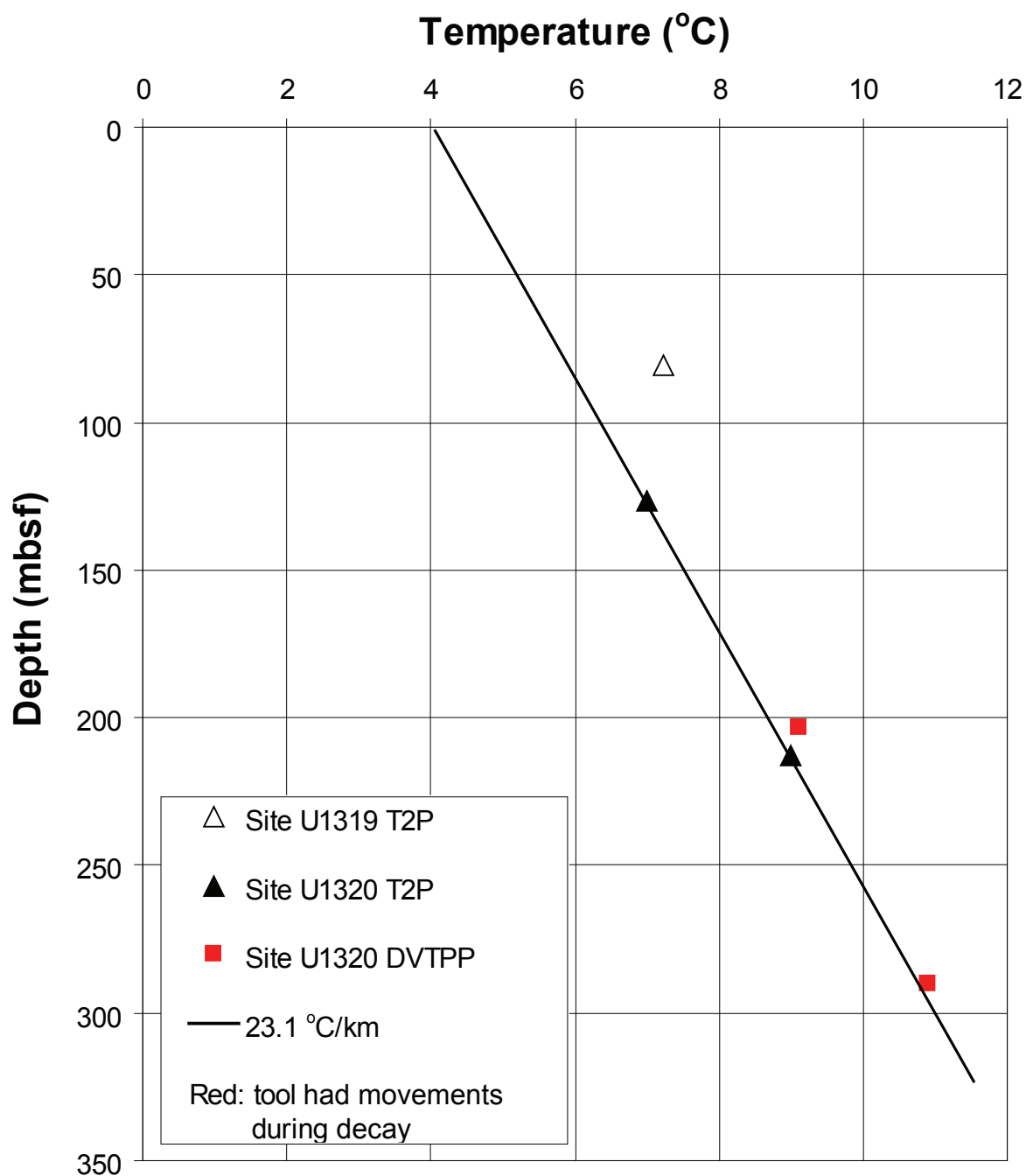
Figure A.8: In situ temperature in Brazos Trinity IV Basin at Site U1319 and Site U1320. T2P temperature reached equilibrium with the formation temperature at the end of the deployment (Table A.2, column 11). However the DVTPP temperature did not equilibrate with the formation temperature at the end of the deployment. In situ temperatures were estimated using 1/t extrapolation (Table A.2, column 12). Red symbols represent temperature measurements that were subjected to influence of tool movements during the dissipation phase.
