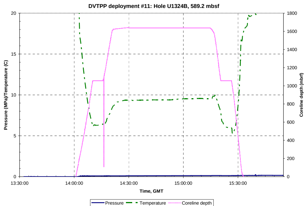
Figure A.A.10.a: Pressure, temperature and Truview data for DVTPP Deployment #11, Hole U1324B, 589.2 mbsf. GMT = Greenwich Mean Time, Hydrostatic_BOH is the hydrostatic pressure at the bottom of the hole.
