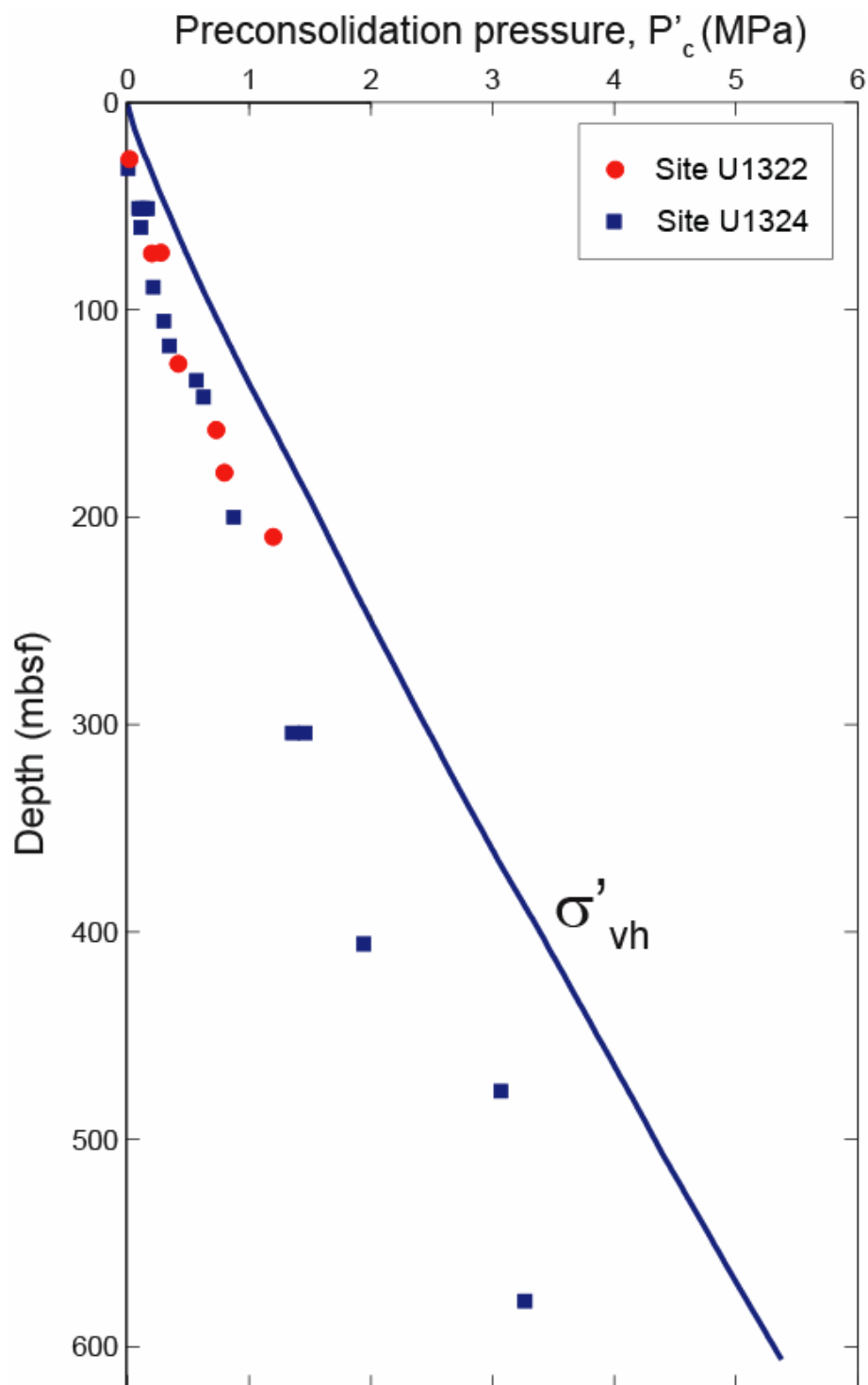
Figure B.29: Pre-consolidation pressure for Ursa sediments (Table B.3, columns 2 and 8). The pre-consolidation stress is determined using the work-stress method proposed by Becker, (1987). The hydrostatic vertical effective stress is calculated using the shipboard bulk density data assuming a seawater density of 1.024 g/cc.
