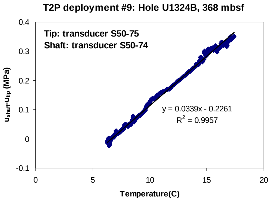
Figure A.B.8: Pressure difference between the tip pressure and shaft pressure for T2P Deployment #9, Hole U1324B, 368 mbsf. The tip pressure was calibrated using the post-cruise calibration data of transducer S50-75. The shaft pressure was calibrated using the onboard calibration factors of transducer S50-74. The tip and shaft pressures prior to penetration were used.
