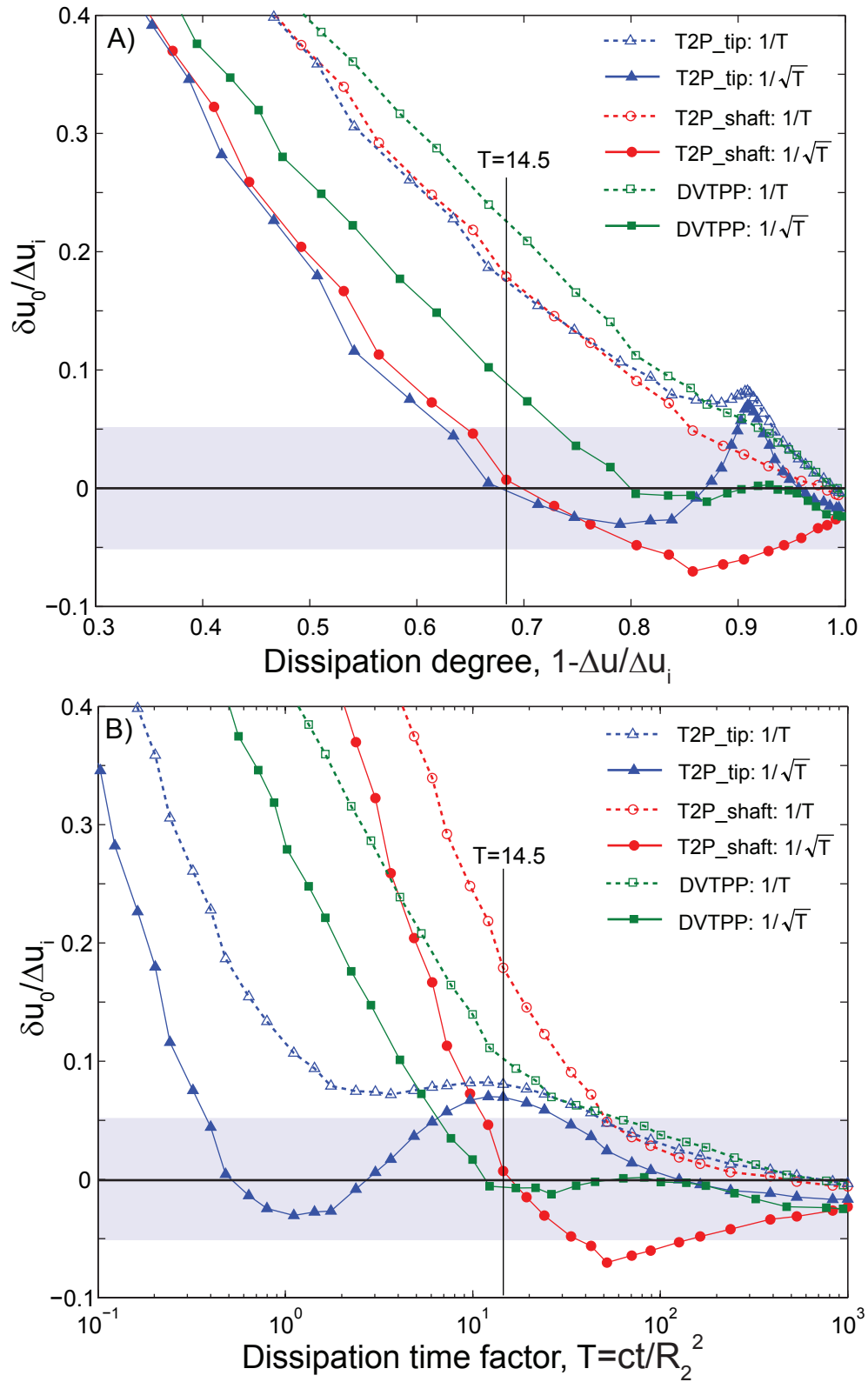
Figure 2.8: Theoretical prediction of errors in estimating u_0 by 1/\sqrt{t} and 1/t extrapolation. The colored band marks an error window of \pm 5\% of the installation pressure ( \Delta u_i ). A) Errors as a function of dissipation degree. B) Error as a function of dissipation time factor ( T ).
