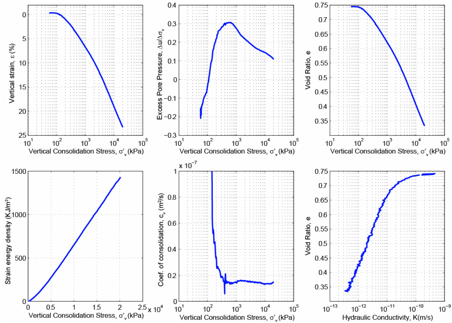
Figure B.23: CRS006 consolidation data for Sample U1324B-70X-6WR, 578.13 mbsf.
