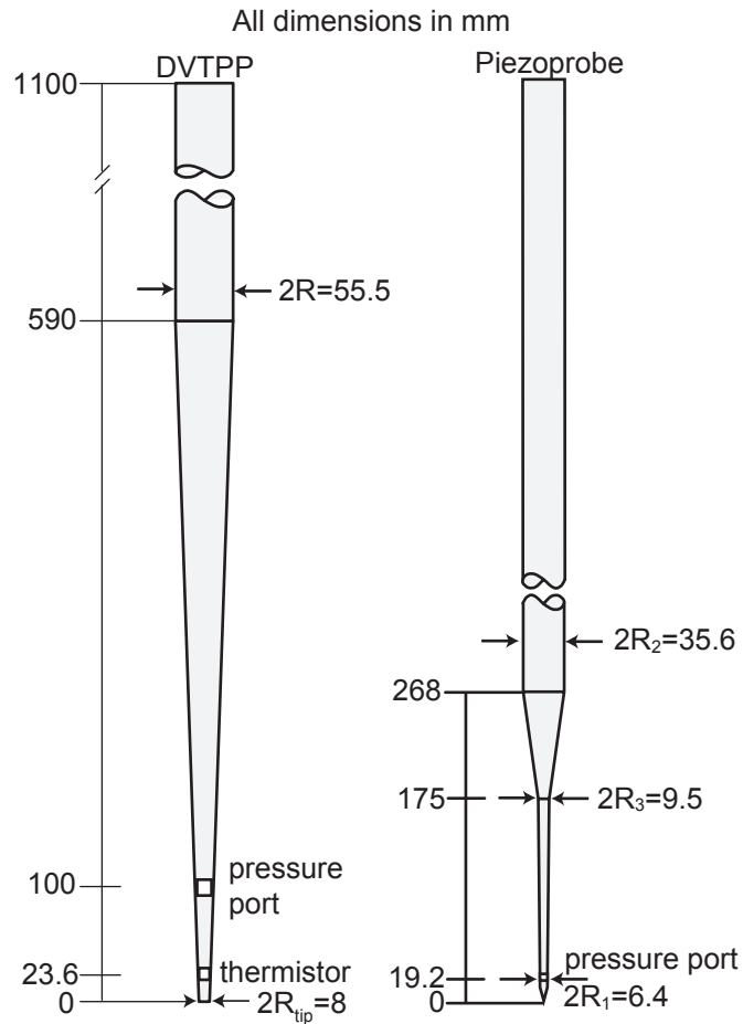
Figure 1.1: The DVTTP and Piezoprobe pore pressure penetrometers have very different geometries. The DVTTP (left) has a long, tapered tip that extends beyond the constant diameter shaft. Its tip tapers continuously from 8 to 55.5 mm in diameter. The pressure port is located 100 mm above the tip. The Piezoprobe (right) has a tapered extension piece 268 mm long which fits onto the end of a standard 35.6 mm diameter cone rod. The tip of the probe is 175 mm long and it has a 9.5 mm diameter at the top and a 6.4 mm diameter near the tip. Pore pressures are measured through a porous filter element located 19.2 mm above the tip, where the probe has a 6.4 mm.
