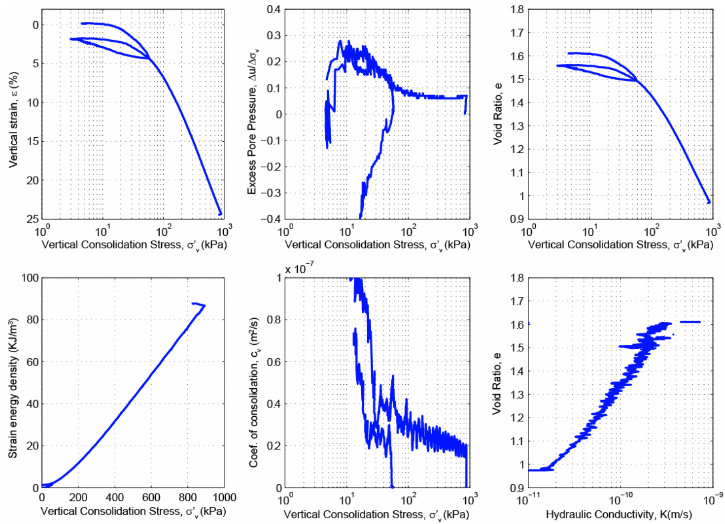
Figure B.15: CRS815 consolidation data for Sample U1322B-4H-3WR, 27.21 mbsf.
