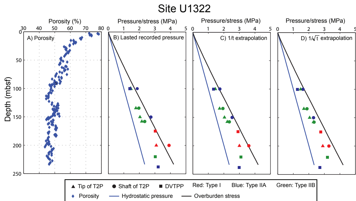
Figure A.12: Pore pressure measurements at Site U1322. The hydrostatic pressure is calculated starting from the seafloor assuming a seawater density of 1.024 g/cc. Bulk density data from shipboard Moisture and Density measurements (MAD) were integrated to calculate the overburden stress. The static pressure due to the water column above seafloor was subtracted from the pressure results. A) Porosity obtained from shipboard moisture and density (MAD) measurement. B) Last recorded pressure of the penetrometer (Table A.2, column 8). C) In situ pore pressure estimated by 1/t extrapolation (Table A.2, column 9). D) In situ pore pressure estimated by 1/\sqrt{t} extrapolation (Table A.2, column 10).
