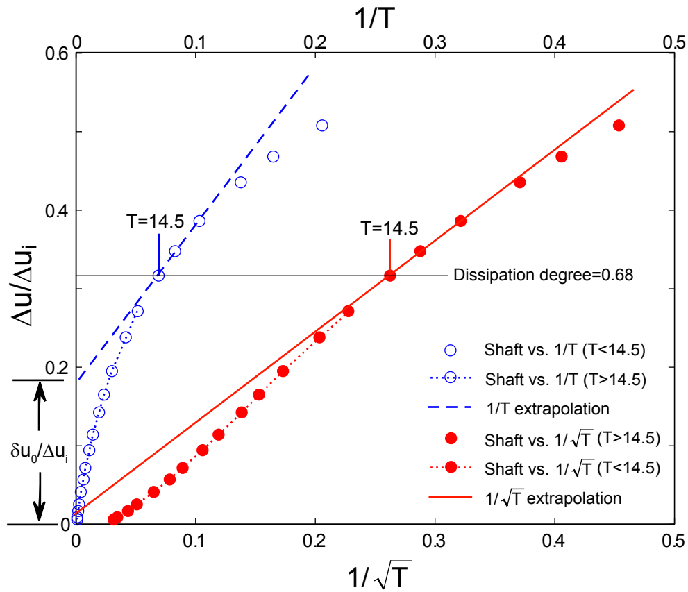
Figure 2.7: Estimating in-situ pressure from incomplete dissipation record using 1/\sqrt{t} and 1/t extrapolation. The excess pore pressure ratio prediction of the shaft of T2P (Figure 2.6) is plotted with 1/\sqrt{T} and 1/T respectively. Linear extrapolations are conducted on data with the dissipation time T = 14.5 (hollow and solid circles with no lines). The circles with dashed line represent the modeled dissipation curve for T > 14.5 .
