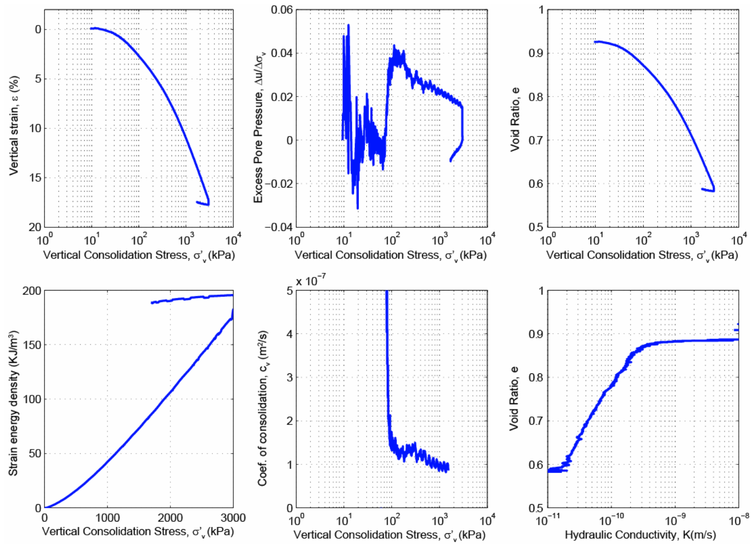
Figure B.17: CRS825 consolidation data for Sample U1322B-21H-3WR, 178.7 mbsf.
