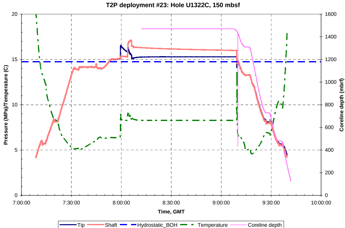
Figure A.B.26.a: Pressure, temperature and Truview data for T2P deployment #23, Hole U1322C, 150 mbsf. GMT = Greenwich Mean Time, Hydrostatic_BOH is the hydrostatic pressure at the bottom of the hole.
