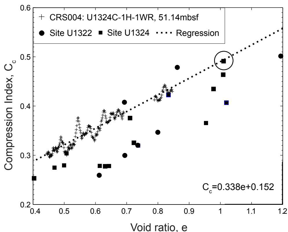
Figure 4.6: Compression indices for Ursa mudstones. The values of C_c for individual consolidation tests are determined over a stress range of 1.5 to 2.5 times the hydrostatic vertical effective stress at the corresponding depth. They are plotted with the mean void ratio over the stress range. Data within the rectangles in Figure 4.7 were used to calculate the C_c values for test CRS004. C_c was computed over a data interval with a load increment ratio of 1.1.
