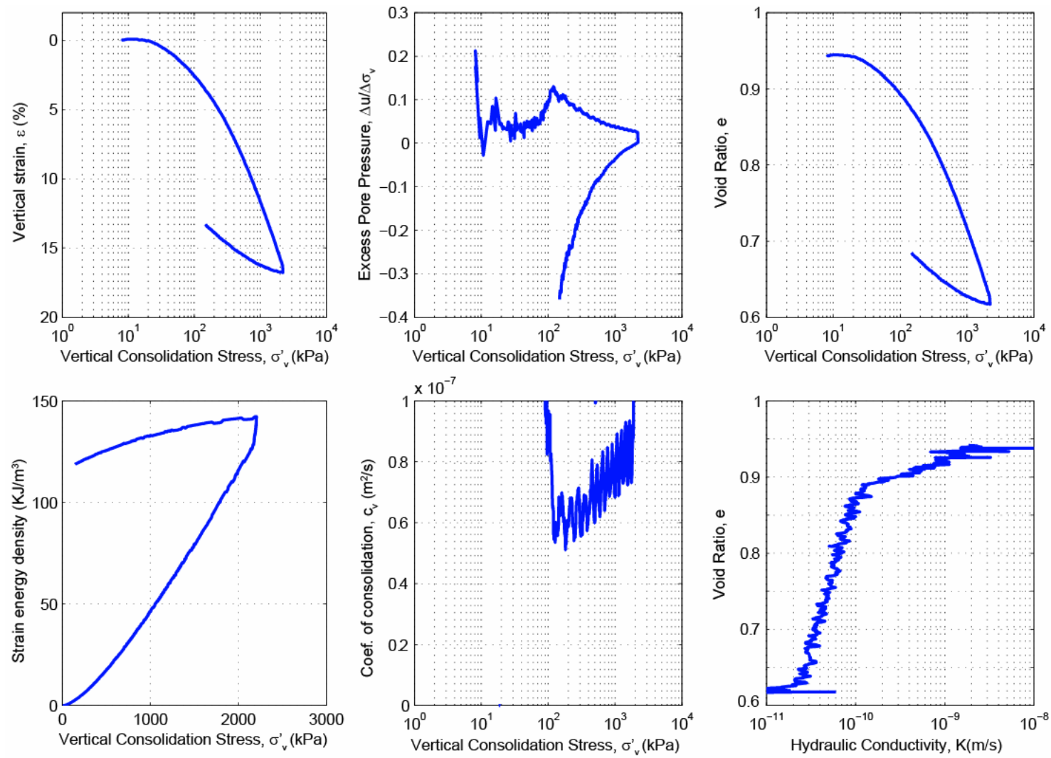
Figure B.9: CRS803 consolidation data for Sample U1324B-15H-5WR, 134.2 mbsf.
