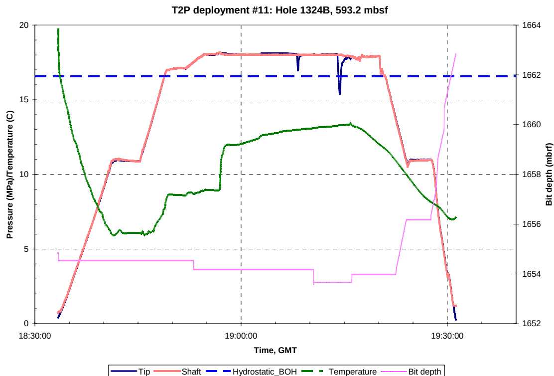
Figure A.B.17.a: Pressure, temperature and Truview data for T2P deployment #11, Hole U1324B, 593.2 mbsf. GMT = Greenwich Mean Time, Hydrostatic_BOH is the hydrostatic pressure at the bottom of the hole.
