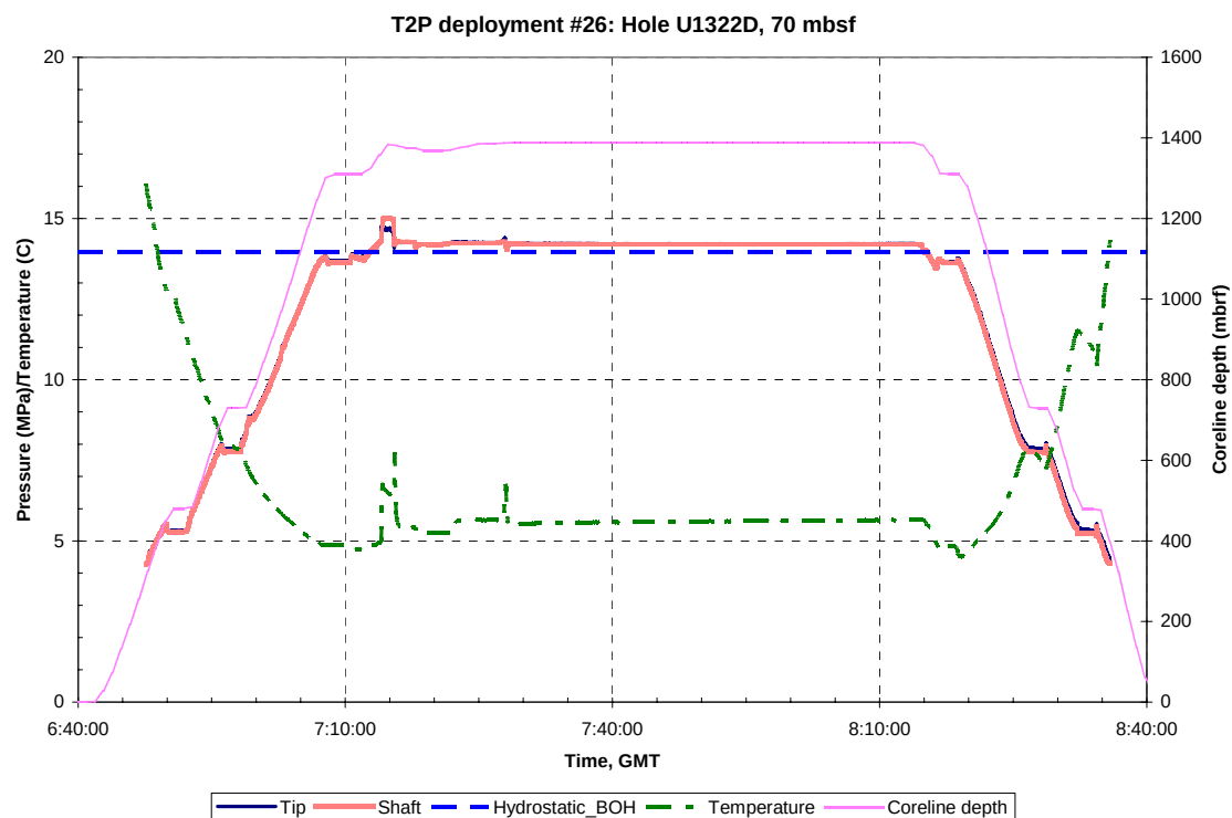
Figure A.B.29.a: Pressure, temperature and Truview data for T2P deployment #26, Hole U1322D, 70 mbsf. GMT = Greenwich Mean Time, Hydrostatic_BOH is the hydrostatic pressure at the bottom of the hole.
