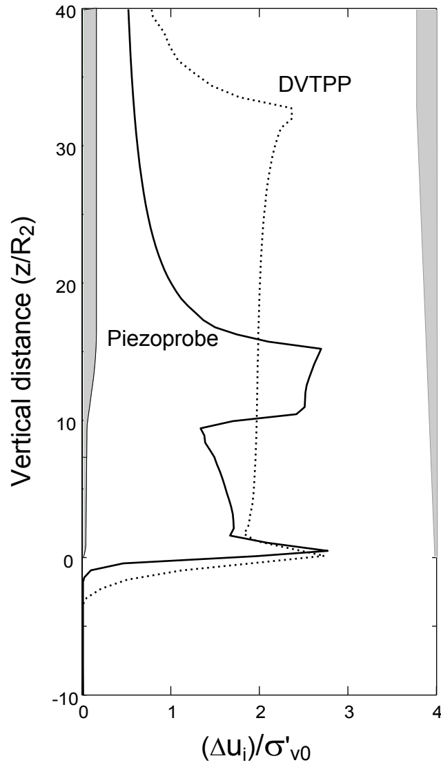
Figure 1.11: Initial excess pore pressure along the surface of the DVTPP and Piezoprobe. The Piezoprobe has peaks in pore pressure at the tip and at the tip-shaft transition. In contrast the DVTPP has a broad zone of elevated pressure associated with its tapered geometry (right). Here, \Delta u_i is normalized by the vertical effective stress ( \sigma'_{v0} ) prior to penetration.
