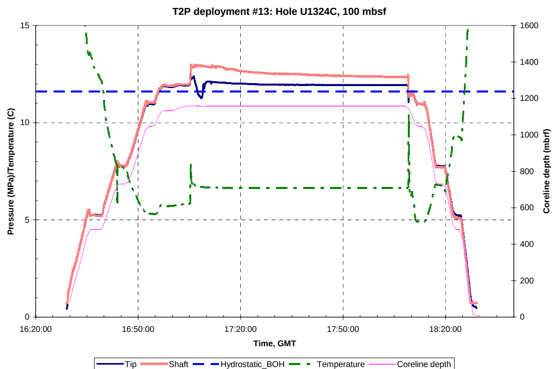
Figure A.B.19.a: Pressure, temperature and Truview data for T2P deployment #13, Hole U1324C, 100 mbsf. GMT = Greenwich Mean Time, Hydrostatic_BOH is the hydrostatic pressure at the bottom of the hole.
