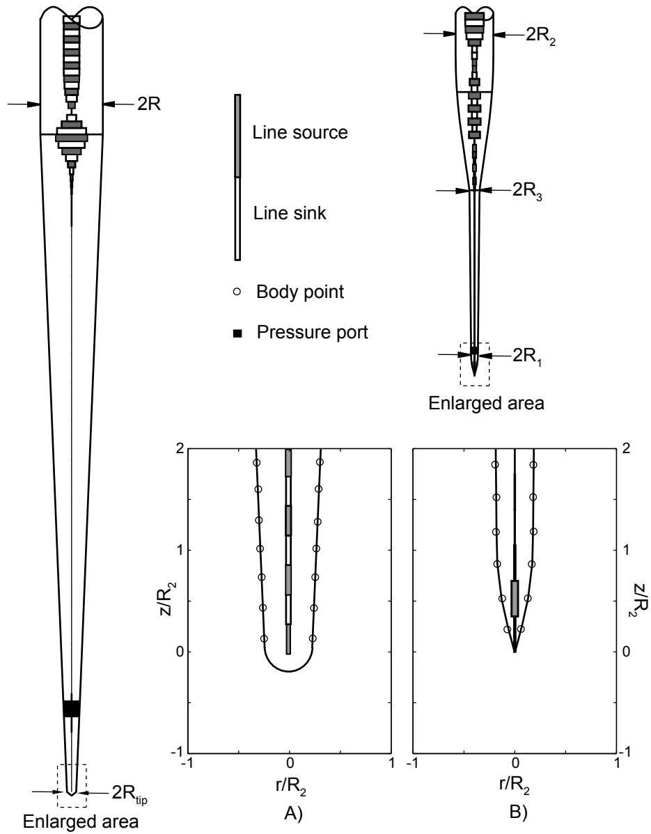
Figure 1.7: Source-sink combinations used to simulate inviscid flow around A) the DVTTP and B) the Piezoprobe. Sources/sinks are located along the centerline of probe. The line weights represent their relative strengths. The small circles on the probe surface represent the body points selected to simulate probe geometry.
