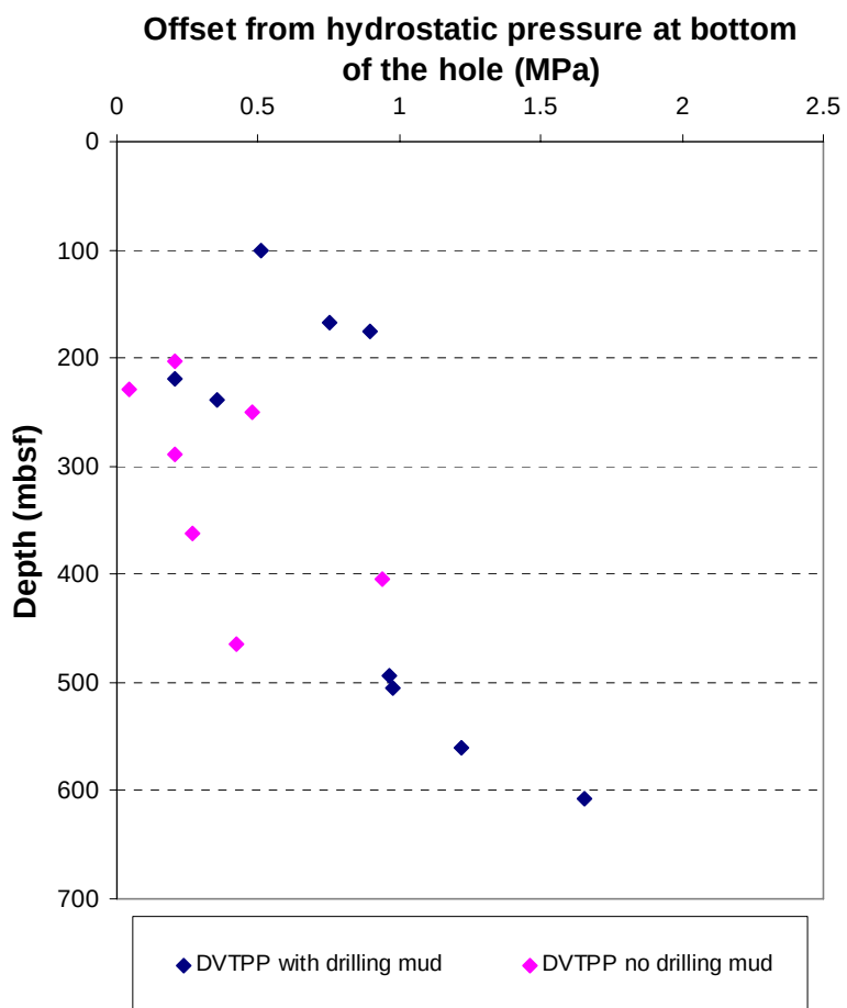
Figure A.C.2 : Offset between the tool pressure and the hydrostatic pressure at the bottom of the hole. The hydrostatic pressure was calculated assuming a seawater density of 1.024 g/cc.
