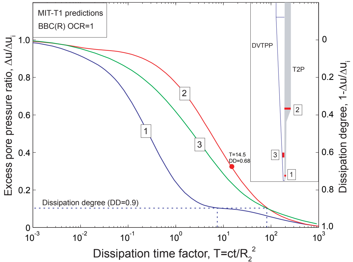
Figure 2.6: Modeled pressure dissipation for the T2P (tip #1; shaft #2) and the DVTPP (#3). Excess pore pressure ratio is plotted in log time. Dissipation time factor is normalized by the diffusivity and the radius of the shaft of the T2P. The geometries and locations of pressure ports of the T2P and the DVTPP are shown in the inset figure.
