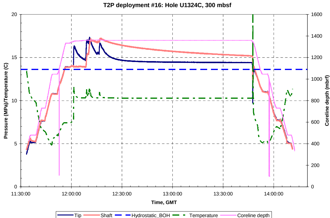
Figure A.B.22.a: Pressure, temperature and Truview data for T2P deployment #16, Hole U1324C, 300 mbsf. GMT = Greenwich Mean Time, Hydrostatic_BOH is the hydrostatic pressure at the bottom of the hole.
