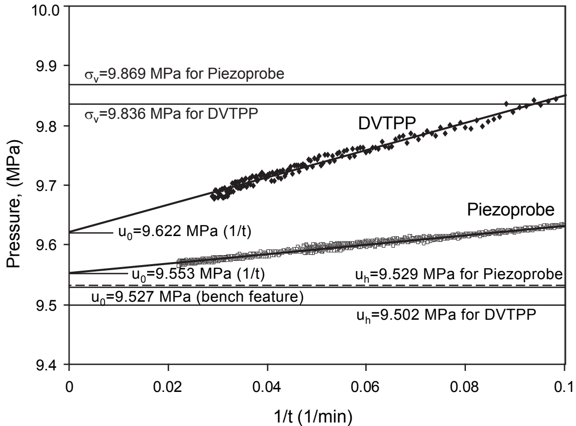
Figure 1.13: The predicted in situ pore pressure from the DVTTP and the Piezoprobe data from an inverse time ( 1/t ) approach and from using the "bench" predicted from the modeled dissipation of the Piezoprobe ("bench feature"). The "bench" feature yields an estimate of 9.527 MPa based on the Piezoprobe data. The in situ pore pressures estimated using 1/t technique are shown for comparison. The in situ pressure extrapolated from the DVTTP data is much higher than that extrapolated from the Piezoprobe data. Hydrostatic pressure ( u_h ) and overburden stress ( \sigma_v ) at the depth of the DVTTP and Piezoprobe deployments are shown for reference.
