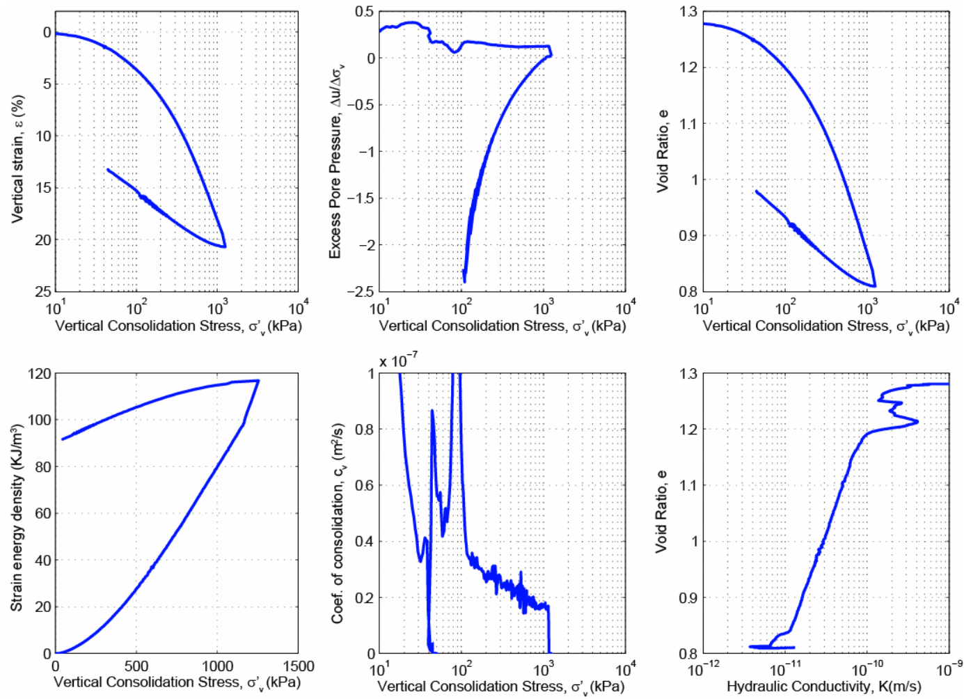
Figure B.2: CRS796 consolidation data for Sample U1322D-2H-2WR, 72.78 mbsf.
