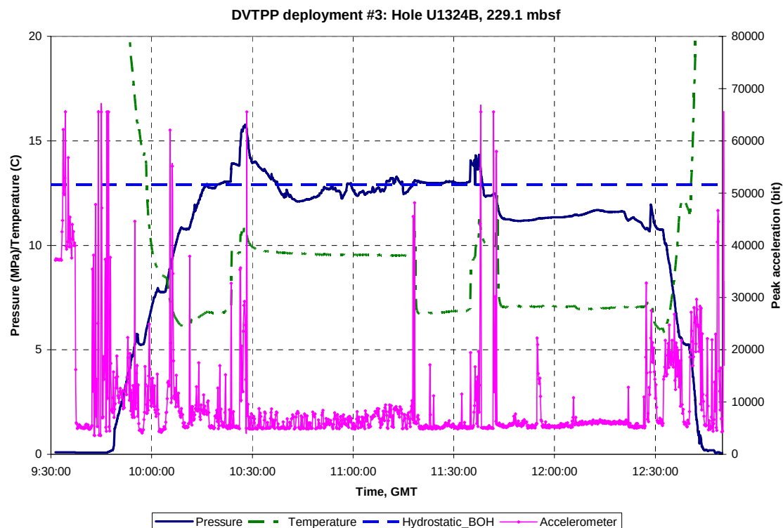
Figure A.A.4: Pressure, temperature and acceleration data for DVTPP Deployment #3, Hole U1324B, 229.1 mbsf. GMT = Greenwich Mean Time, Hydrostatic_BOH is the hydrostatic pressure at the bottom of the hole.
