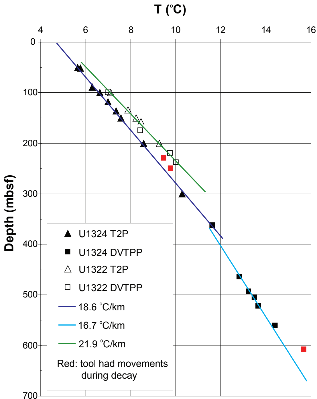
Figure A.9: Temperature data for Ursa Basin at Site U1322 and Site U1324. T2P temperature reached equilibrium with the formation temperature at the end of the deployment (Table A.2, column 11). However the DVTTP temperature did not equilibrate with the formation temperature at the end of the deployment. In situ temperatures were estimated using 1/t extrapolation (Table A.2, column 12). Red symbols represent temperature measurements that were subjected to influence of tool movements during the dissipation phase.
