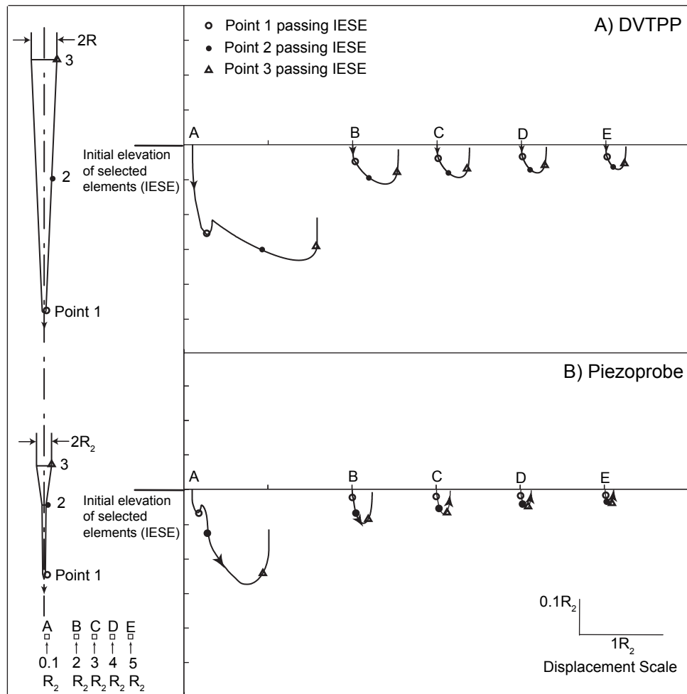
Figure 1.8: Modeled soil deformation paths during penetration. The selected soil elements (A, B, C, D, and E, lower left) are initially located far ahead of the probe tip. The small squares shows the initial radial distance from selected soil elements to the centerline of the probe. As the penetration proceeds, three selected locations on the probe surface (Point 1, Point 2, and Point 3) will sequentially pass by the soil elements. Deformations at the corresponding time are illustrated on the right hand side.
