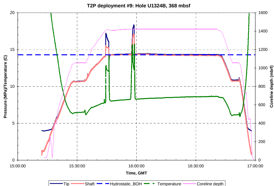
Figure A.B.16.a: Pressure, temperature and Truview data for T2P deployment #9, Hole U1324B, 368 mbsf. GMT = Greenwich Mean Time, Hydrostatic_BOH is the hydrostatic pressure at the bottom of the hole.
