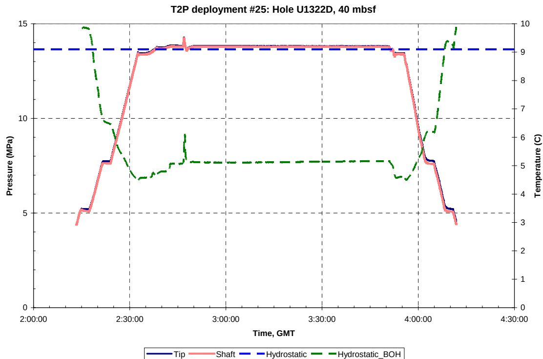
Figure A.B.28: Pressure and temperature data for T2P deployment #25, Hole U1322D, 40 mbsf. GMT = Greenwich Mean Time, Hydrostatic_BOH is the hydrostatic pressure at the bottom of the hole.
