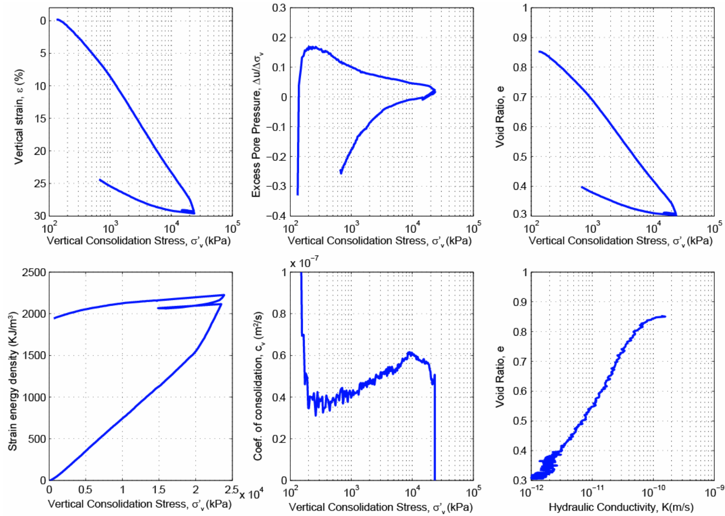
Figure B.19: CRS002 consolidation data for Sample U1324C-6H-3WR, 303.94 mbsf.
