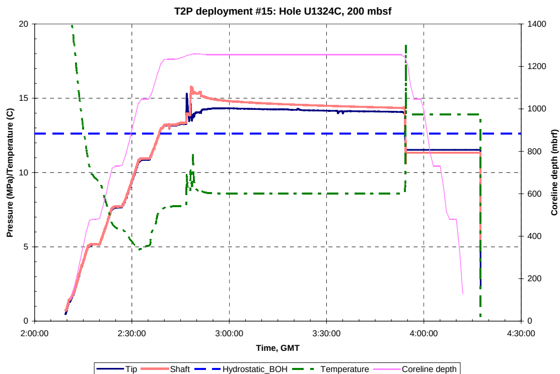
Figure A.B.21.a: Pressure, temperature and Truview data for T2P deployment #15, Hole U1324C, 200 mbsf. GMT = Greenwich Mean Time, Hydrostatic_BOH is the hydrostatic pressure at the bottom of the hole.
