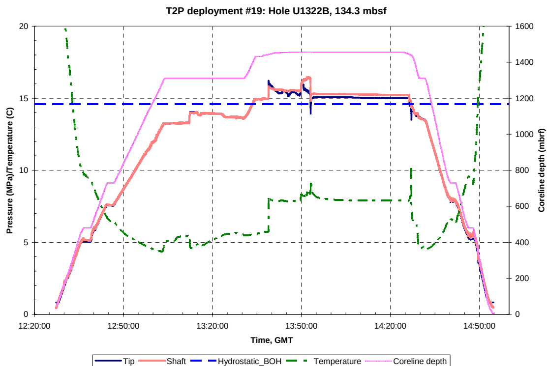
Figure A.B.24.a: Pressure, temperature and Truview data for T2P deployment #19, Hole U1322B, 134.3 mbsf. GMT = Greenwich Mean Time, Hydrostatic_BOH is the hydrostatic pressure at the bottom of the hole.
