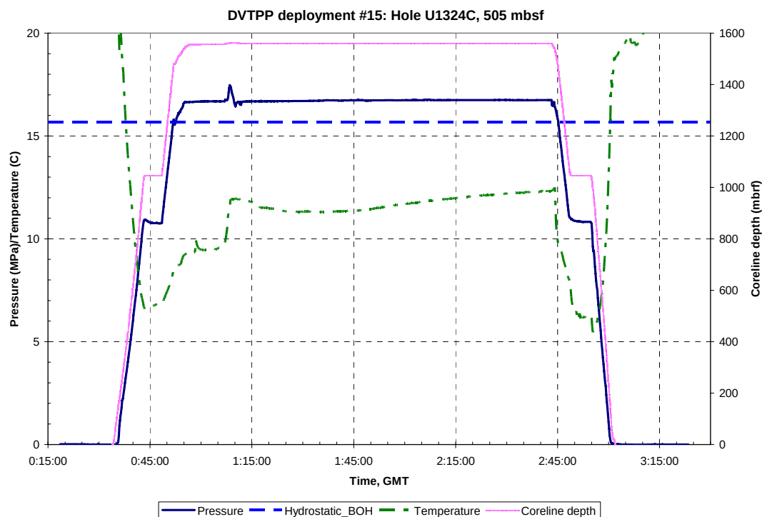
Figure A.A.14.a: Pressure, temperature and Truview data for DVTPP Deployment #15, Hole U1324C, 505 mbsf. GMT = Greenwich Mean Time, Hydrostatic_BOH is the hydrostatic pressure at the bottom of the hole.
