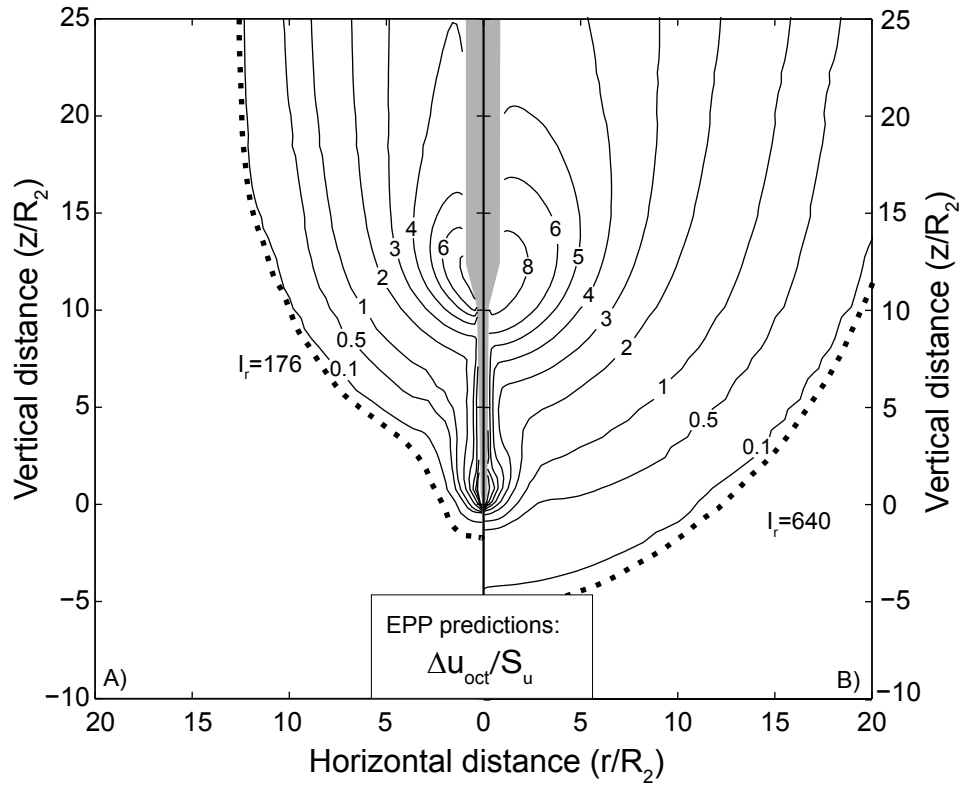
Figure 3.5: Initial excess pore pressure fields around the T2P predicted by EPP model. Left: Pressure field predicted for an I_r of 176. Right: pore pressure field predicted for an I_r =640. The dashed line marks the boundary of the failure zone. Shear-induced pore pressure is not included in this analysis (see text).
