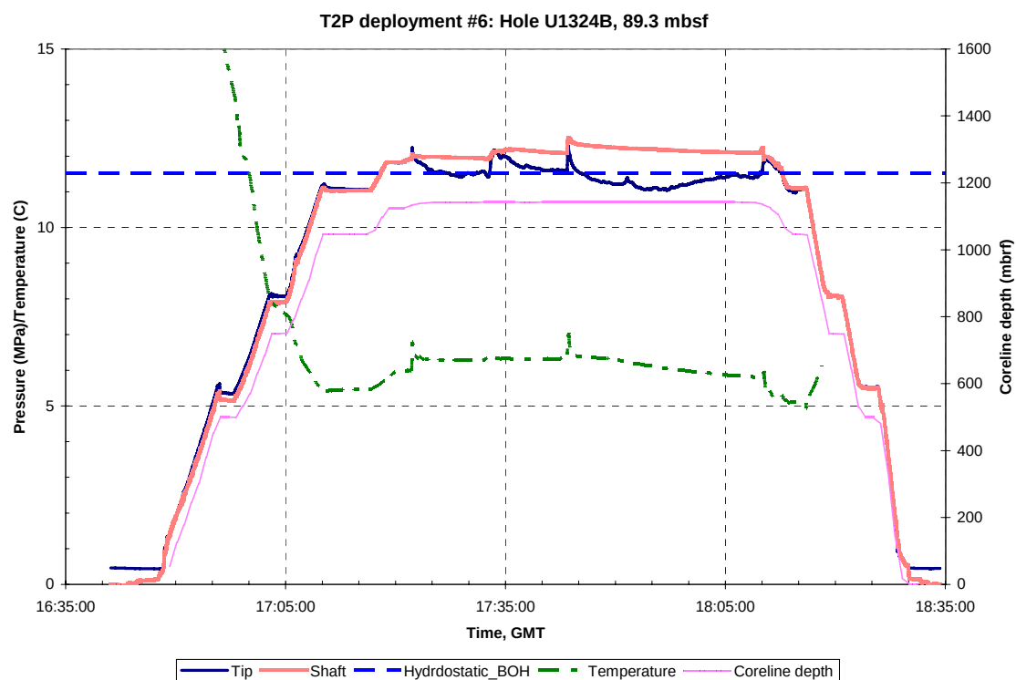
Figure A.B.13.a: Pressure, temperature and Truview data for T2P deployment #6, Hole U1324B, 89.3 mbsf. GMT = Greenwich Mean Time, Hydrostatic_BOH is the hydrostatic pressure at the bottom of the hole.
