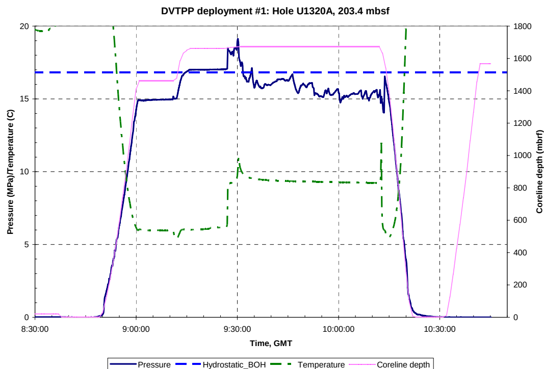
Figure A.A.2.a: Pressure, temperature and Truview data for DVTPP Deployment #1, Hole U1320A, 203.4 mbsf. GMT = Greenwich Mean Time, Hydrostatic_BOH is the hydrostatic pressure at the bottom of the hole.
