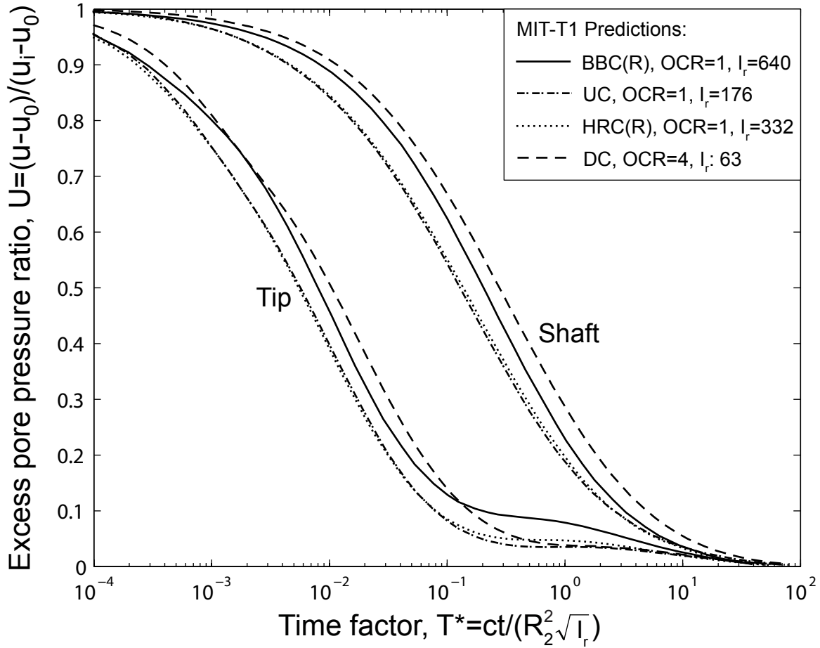
Figure 3.12: Pressure dissipation predicted by the MIT-T1 model ( \Delta u_s is neglected). Excess pore pressure ratio ( U ) is plotted against modified time factor T^* . BBC=Boston Blue Clay, UC=Ursa Clay, HRC=Hydrate Ridge Clay, DC= Drammen Clay. OCR= overconsolidation ratio. I_r values are calculated according to the method illustrated in Figure 3.4.
