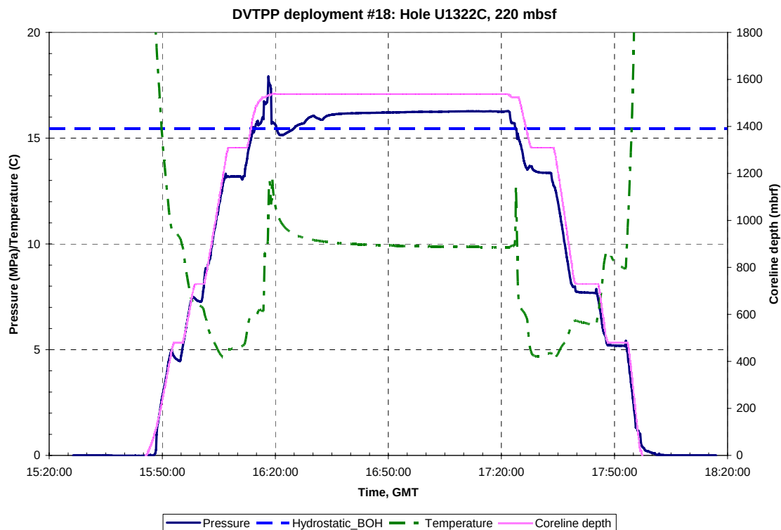
Figure A.A.17.a: Pressure, temperature and Truview data for DVTPP Deployment #18, Hole U1322C, 220 mbsf. GMT = Greenwich Mean Time, Hydrostatic_BOH is the hydrostatic pressure at the bottom of the hole.
