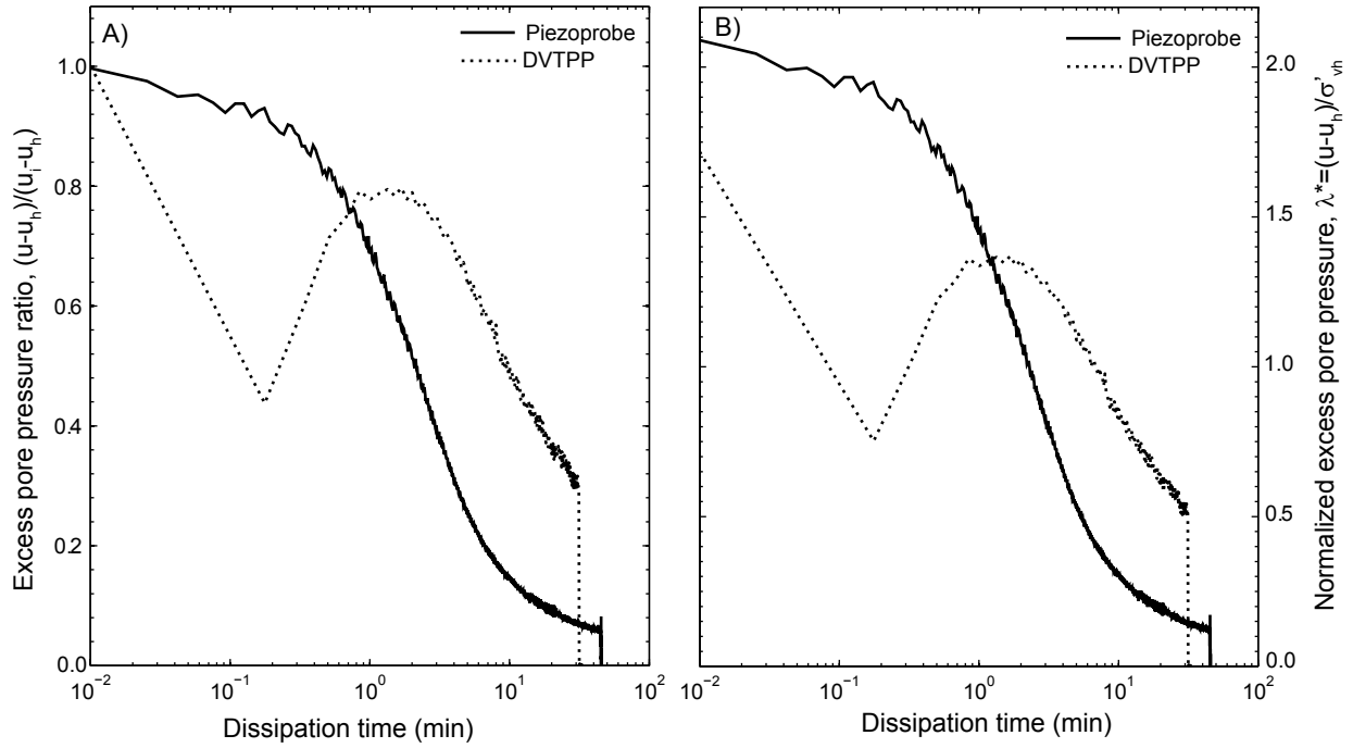
Figure 1.5: Comparison of DVTTP pressure dissipation (dotted line) and Piezoprobe pressure dissipation (solid line). A) Excess pore pressure ratio. Here, u_i is the peak pore pressure upon insertion, and u_h is the hydrostatic pressure at penetration depth. The Piezoprobe has dissipated 94% of its induced pressure while the DVTTP has dissipated only 70% of its induced pressure at the end of deployment. B) Normalized excess pore pressure. The DVTTP has an initial excess pore pressure 1.75 times the hydrostatic vertical effective stress ( \sigma'_{vh} ) and dissipates to 0.5\sigma'_{vh} . The Piezoprobe has an insertion pressure of 2.05\sigma'_{vh} and declines to 0.12\sigma'_{vh} .
