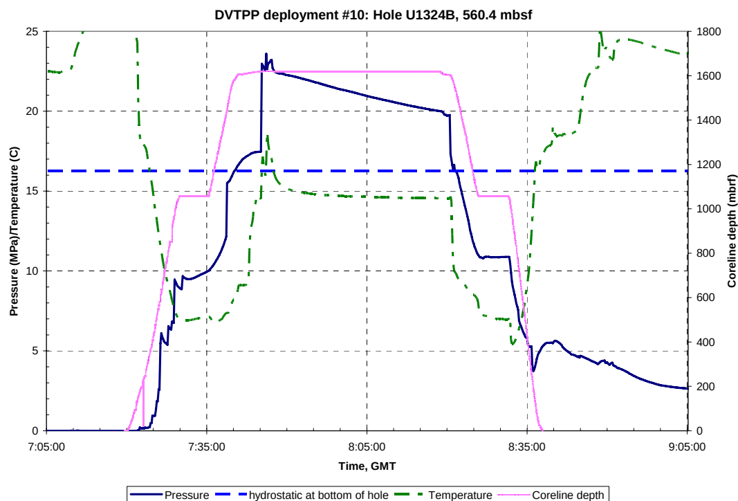
Figure A.A.9.a: Pressure, temperature and Truview data for DVTPP Deployment #10, Hole U1324B, 560.4 mbsf. GMT = Greenwich Mean Time, Hydrostatic_BOH is the hydrostatic pressure at the bottom of the hole.
