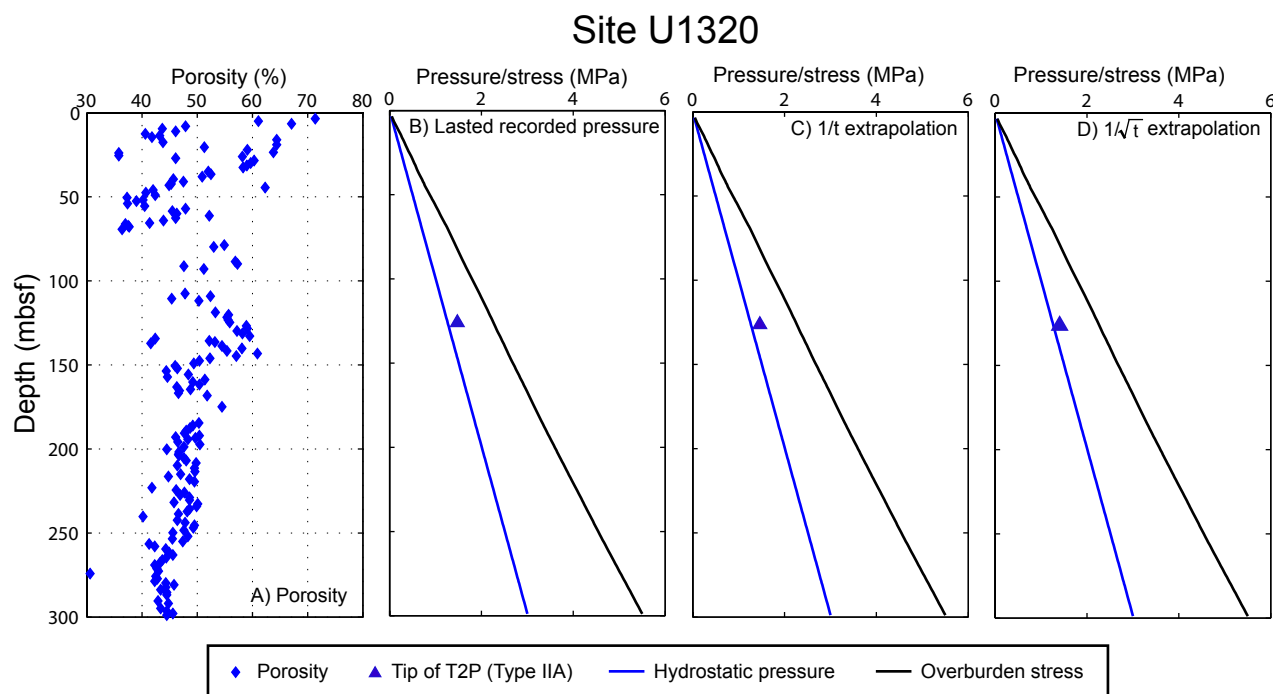
Figure A.11: Pore pressure measurements at Site U1320. The hydrostatic pressure is calculated starting from the seafloor assuming a seawater density of 1.024 g/cc. Bulk density data from shipboard Moisture and Density measurements (MAD) were integrated to calculate the overburden stress. The static pressure due to the water column above seafloor was subtracted from the pressure results. A) Porosity obtained from shipboard moisture and density (MAD) measurement. B) Last recorded pressure of the penetrometer (Table A.2, column 8). C) In situ pore pressure estimated by 1/t extrapolation (Table A.2, column 9). D) In situ pore pressure estimated by 1/\sqrt{t} extrapolation (Table A.2, column 10).
