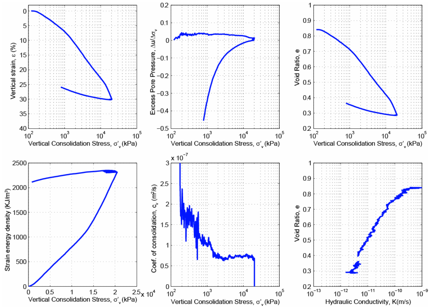
Figure B.18: CRS001 consolidation data for Sample U1324C-6H-3WR, 304.02 mbsf.
