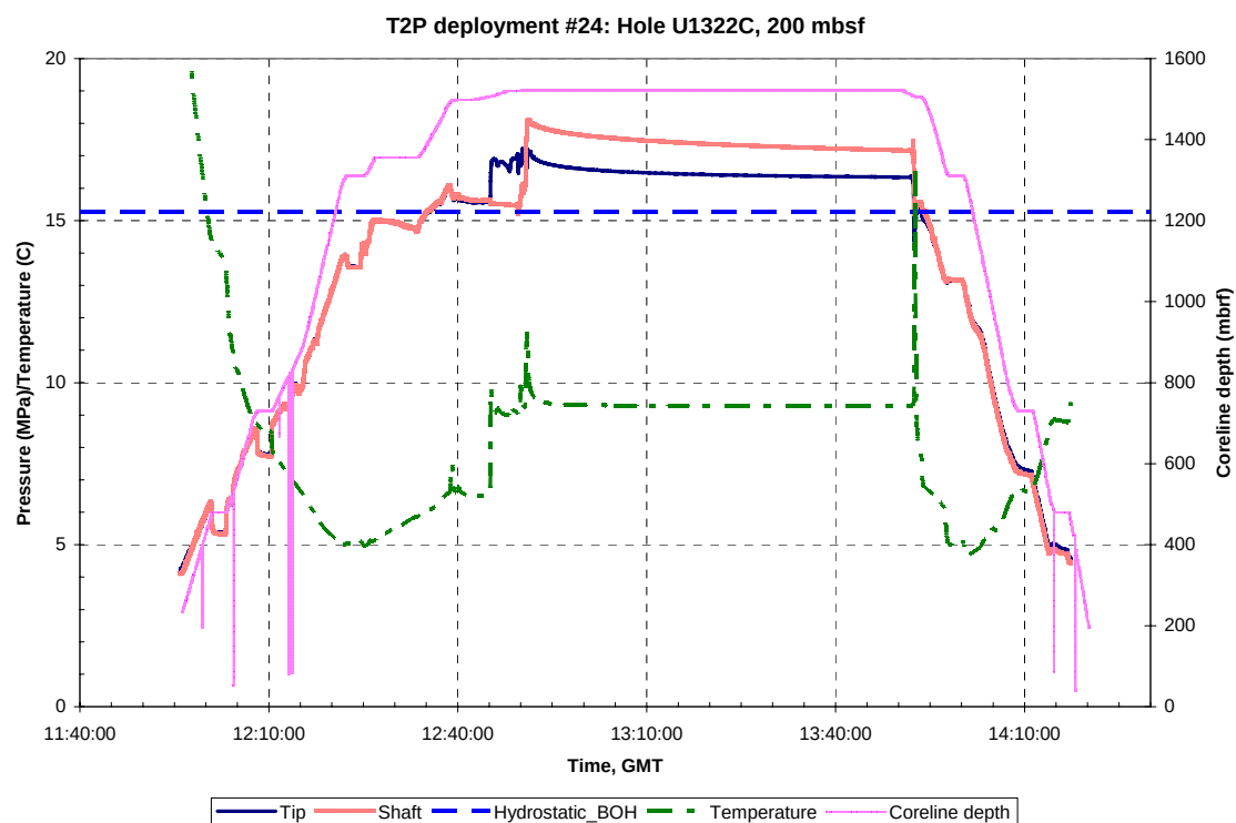
Figure A.B.27.a: Pressure, temperature and Truview data for T2P deployment #24, Hole U1322C, 200 mbsf. GMT = Greenwich Mean Time, Hydrostatic_BOH is the hydrostatic pressure at the bottom of the hole.
