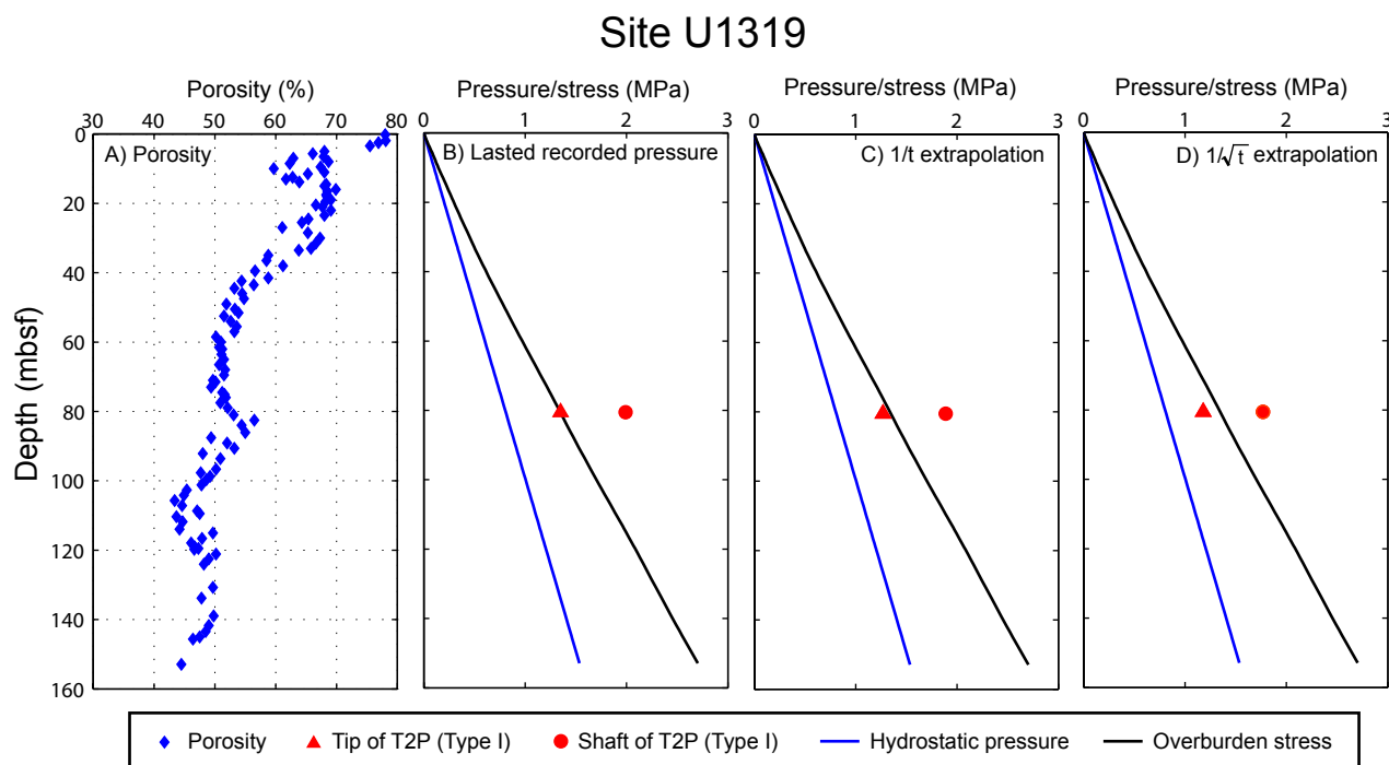
Figure A.10: Pore pressure measurements at Site U1319. The hydrostatic pressure is calculated starting from the seafloor assuming a seawater density of 1.024 g/cc. Bulk density data from shipboard Moisture and Density measurements (MAD) were integrated to calculate the overburden stress. The static pressure due to the water column above seafloor was subtracted from the pressure results. A) Porosity obtained from shipboard moisture and density (MAD) measurement. B) Last recorded pressure of the penetrometer (Table A.2, column 8). C) In situ pore pressure estimated by 1/t extrapolation (Table A.2, column 9). D) In situ pore pressure estimated by 1/\sqrt{t} extrapolation (Table A.2, column 10).
