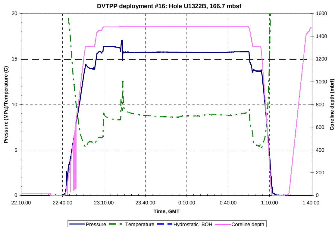
Figure A.A.15.a: Pressure, temperature and Truview data for DVTPP Deployment #16, Hole U1322B, 166.7 mbsf. GMT = Greenwich Mean Time, Hydrostatic_BOH is the hydrostatic pressure at the bottom of the hole.
