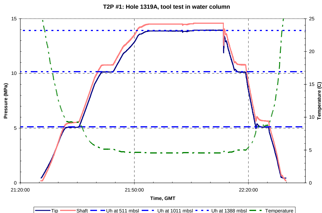
Figure A.B.7.a: T2P deployment #1: pressure test in water column. Transducer S50-73 measures the tip pressure. Transducer Z59-72 measures the shaft pressure. GMT = Greenwich Mean Time. a) pressure data calculated using the calibration coefficients from the onboard pressure calibration (Table A.B.2). b) pressure data calculated using the calibration coefficients interpreted from the post-cruise pressure calibration (Figure A.B.4 and A.B.5). c) Correction of shift of the intersection on y-axis due to oven drying: the tip pressure (Figure A.B.7.b) was added 0.25 MPa and the shaft pressure (Figure A.B.7.b) was added 3.57 MPa to match the hydrostatic pressure at the tool stops.
