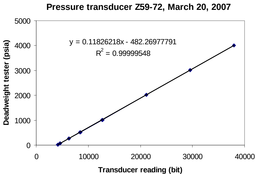
Figure A.B.3: Post-cruise pressure calibration of transducer Z59-72. The calibration was done at 19.976 °C in a temperature bath. The deadweight tester run up to 4015 psi from atmosphere pressure and then stepped down to atmosphere pressure.
