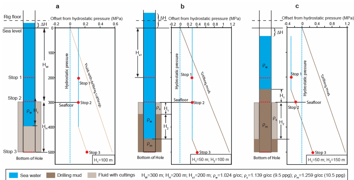
Figure A.C.4: Three possible scenarios that could be encountered at tool stops. The drill-pipe above the rig floor was assumed to be sufficiently long, and three fluids with different density do not mix. The solid brown line represents the predicted static pressure by assuming the borehole was filled with a 10.5 ppg drilling mud. a) Predicted fluid pressure profile for cases with no drilling mud was used whereas fluid in the borehole was contaminated with drilling cuttings. b) Predicted fluid pressure profile for cases with drilling mud was used to stabilize the borehole and the mud elevation within the pipe is lower than the mud elevation outside the pipe. c) Predicted fluid pressure profile for cases with drilling mud was used to stabilize the borehole and the mud elevation within the pipe is higher than the mud elevation outside the pipe.
