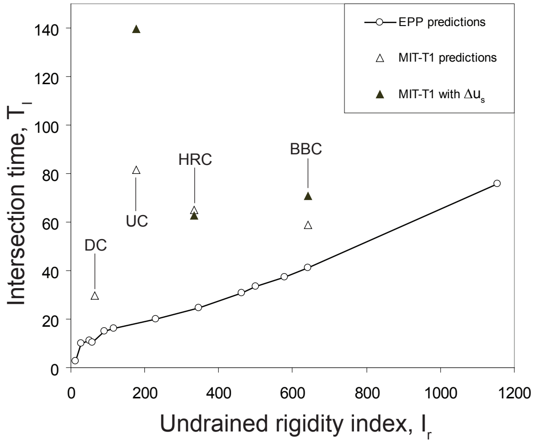
Figure 3.21: Prediction of the intersection time for the two-point matching approach. T_I defines the time factor ( T ) when the dissipated pore pressures are identical for the tip and shaft pressures of the T2P. No shear-induced pore pressure data and model are available for the DC.
