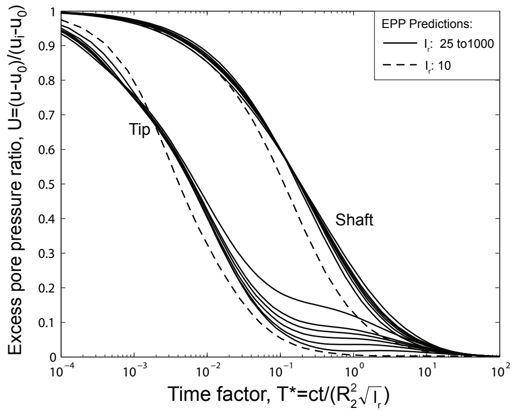
Figure 3.7: Excess pore pressure ratio plotted against time factor T^* for EPP model for increasing values of I_r .
