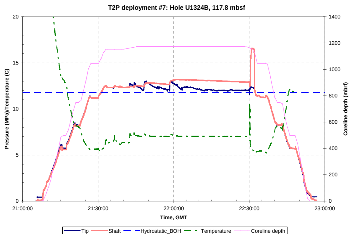
Figure A.B.14.a: Pressure, temperature and Truview data for T2P deployment #7, Hole U1324B, 117.8 mbsf. GMT = Greenwich Mean Time, Hydrostatic_BOH is the hydrostatic pressure at the bottom of the hole.
