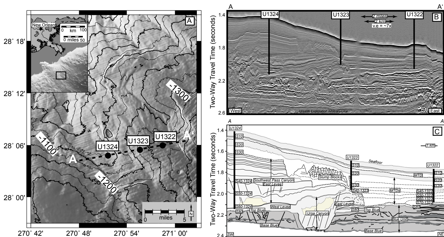
Figure 4.1: A) IODP Expedition 308 Site locations, and bathymetry contours. The Ursa Basin is located 210 km SE of New Orleans, Louisiana, USA (inset map). Three drilled Sites are delineated with black dots. Contour interval is 100 m. (B) East-West seismic cross section A-A' (Flemings, 2006). (C) Interpreted cross section A-A' (Flemings, 2006). The Blue Unit is composed of sand and mud. The darkest gray represents sand-rich channel fill. Mass transport deposits have occurred in the mud-rich levee deposits above the Blue Unit. Detachment surfaces are dotted lines.
