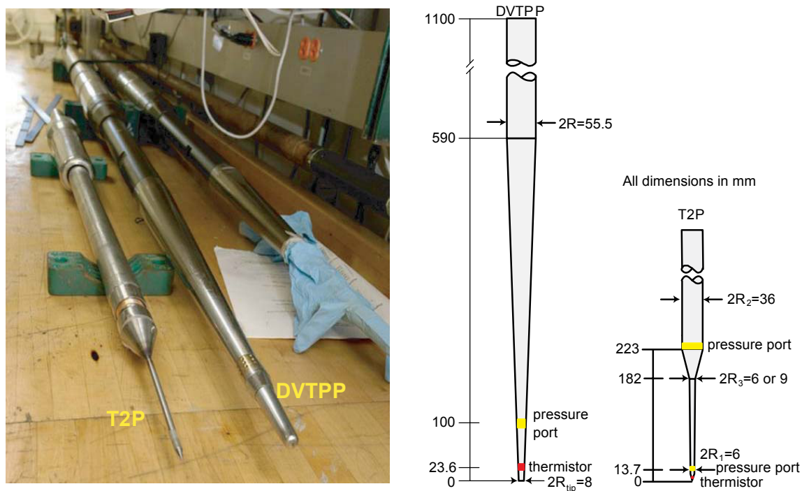
Figure A.4: The DVTPP and T2P pressure penetrometers. The DVTPP has a long, tapered tip that extends beyond the constant diameter shaft. Its tip tapers continuously from 8 to 55.5 mm in diameter. The pressure port is located 100 mm above the tip. The T2P has a tapered extension piece 223 mm long which fits onto the end of a standard 36 mm diameter cone rod. Its modular design allows the use of multiple tip geometries and it measures pore pressure at its narrow tip and at the larger diameter shaft behind the narrow tip.
