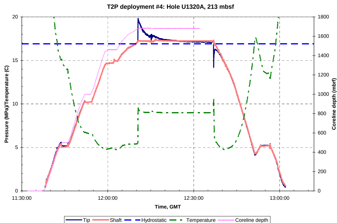
Figure A.B.11.a: Pressure, temperature and Truview data for T2P deployment #4, Hole U1320A, 213 mbsf. GMT = Greenwich Mean Time, Hydrostatic_BOH is the hydrostatic pressure at the bottom of the hole.
