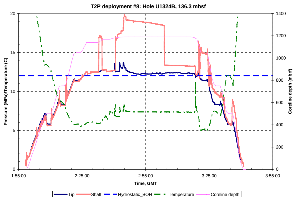
Figure A.B.15.a: Pressure, temperature and Truview data for T2P deployment #8, Hole U1324B, 136.3 mbsf. GMT = Greenwich Mean Time, Hydrostatic_BOH is the hydrostatic pressure at the bottom of the hole.
