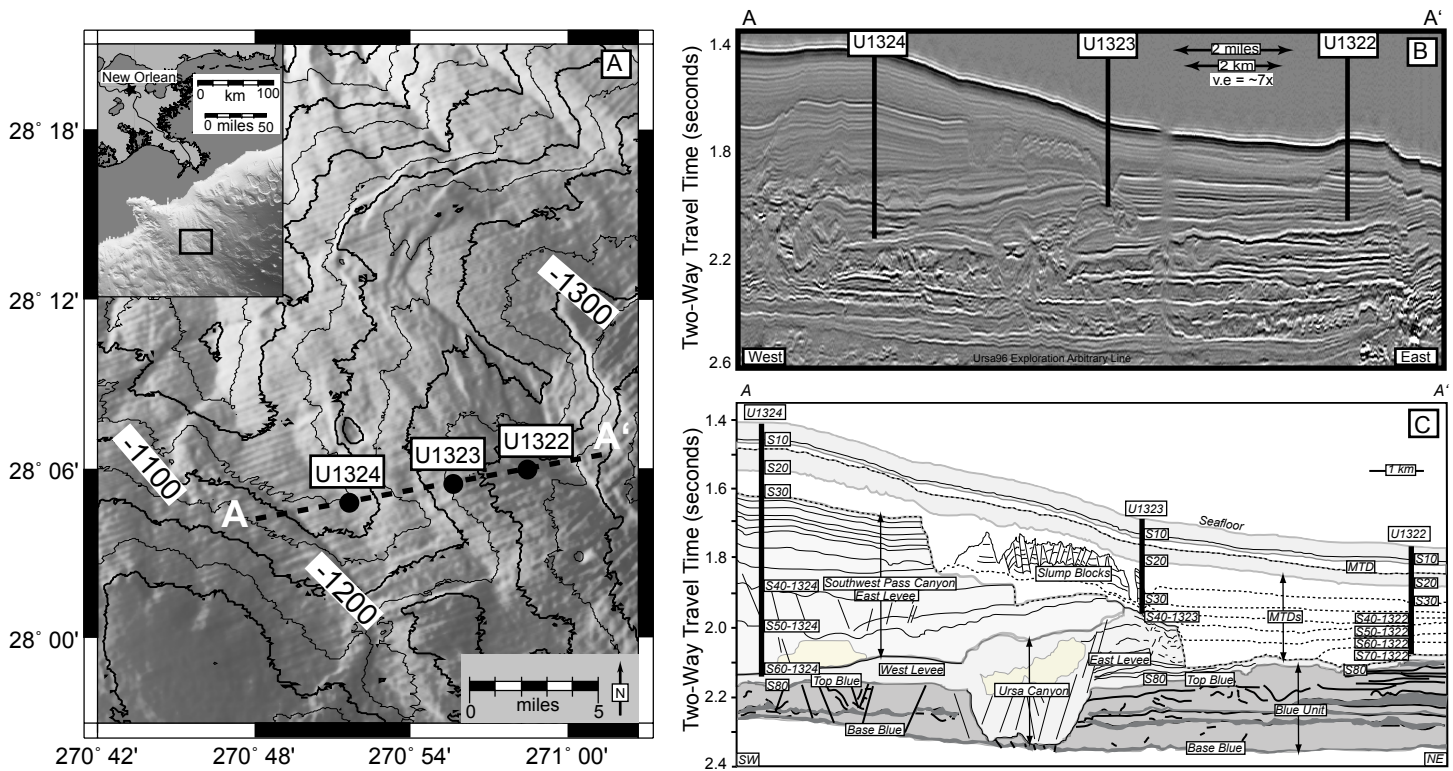
Figure 3.2: Geological setting. A) IODP Expedition 308 Site locations, and bathymetry contours. The Ursa Basin is located 210 km SE of New Orleans, Louisiana, USA (inset map). Three drilled Sites are delineated with black dots. Contour interval is 100 m. (B) East-West seismic cross section A-A' (located in Figure 3.2A). (C) Interpreted cross section A-A'. The Blue Unit is composed of sand and mud. The darkest gray represents sand-rich channel fill. Mass transport deposits have occurred in the mud-rich levee deposits above the Blue Unit. Detachment surfaces are dotted lines.
