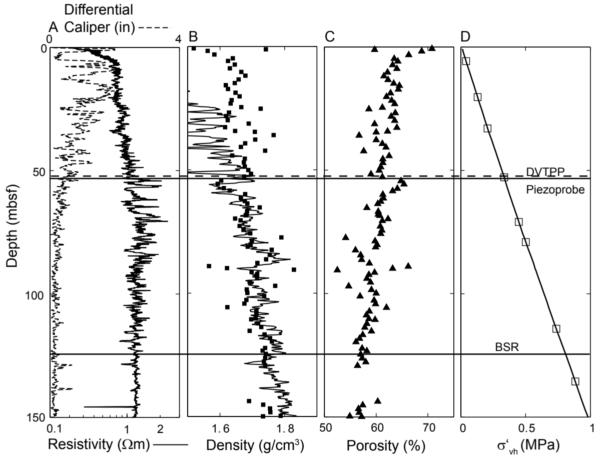
Figure 1.3: Core and log data from ODP Site 1244. The horizontal dashed line and horizontal solid line show where the DVTTP and the Piezoprobe were deployed at approximately 52 meters below sea floor (mbsf). A) Logging While Drilling (LWD) deep resistivity (solid line) and caliper log (dashed line) from Hole 1244D. B) LWD bulk density from Hole 1244D (solid line) and core derived Moisture and Density (MAD) bulk density from Hole 1244C (squares). C) Porosity from Hole 1244C is based on shipboard MAD measurements. D) Hydrostatic effective stress ( \sigma'_{vh} ) is determined by integrating MAD bulk density measured in Hole 1244C and assuming a seawater density of 1.024 g/cm 3 . \sigma'_{vh} is the total overburden stress less the hydrostatic pressure ( \sigma'_{vh} = \sigma_v - u_h ). The squares show where geotechnical samples were taken. Laboratory analysis of these samples provided parameters for modeling presented in the text (Appendix 1.B). BSR= bottom simulating reflector.
