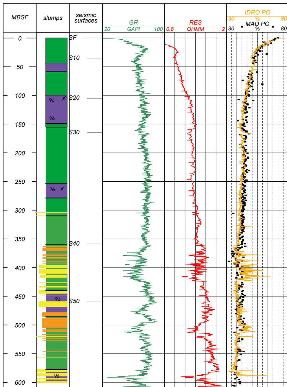
Figure 2.4: IODP Site U1324. A) Depth in meters below sea floor (mbsf). B) Lithologic section. Mass Transport Complexes are delineated in purple. C) Seismic surfaces (see Figure 2.3) are delineated with the letter 'S'. D) Gamma Ray (GR) log. E) Resistivity log (RES) log. F) Porosity log interpreted from shipboard moisture and density (MAD) measurements (solid symbols). Porosity interpreted from logging while drilling (LWD) bulk density log assuming a grain density of 2.74 g/cc.
