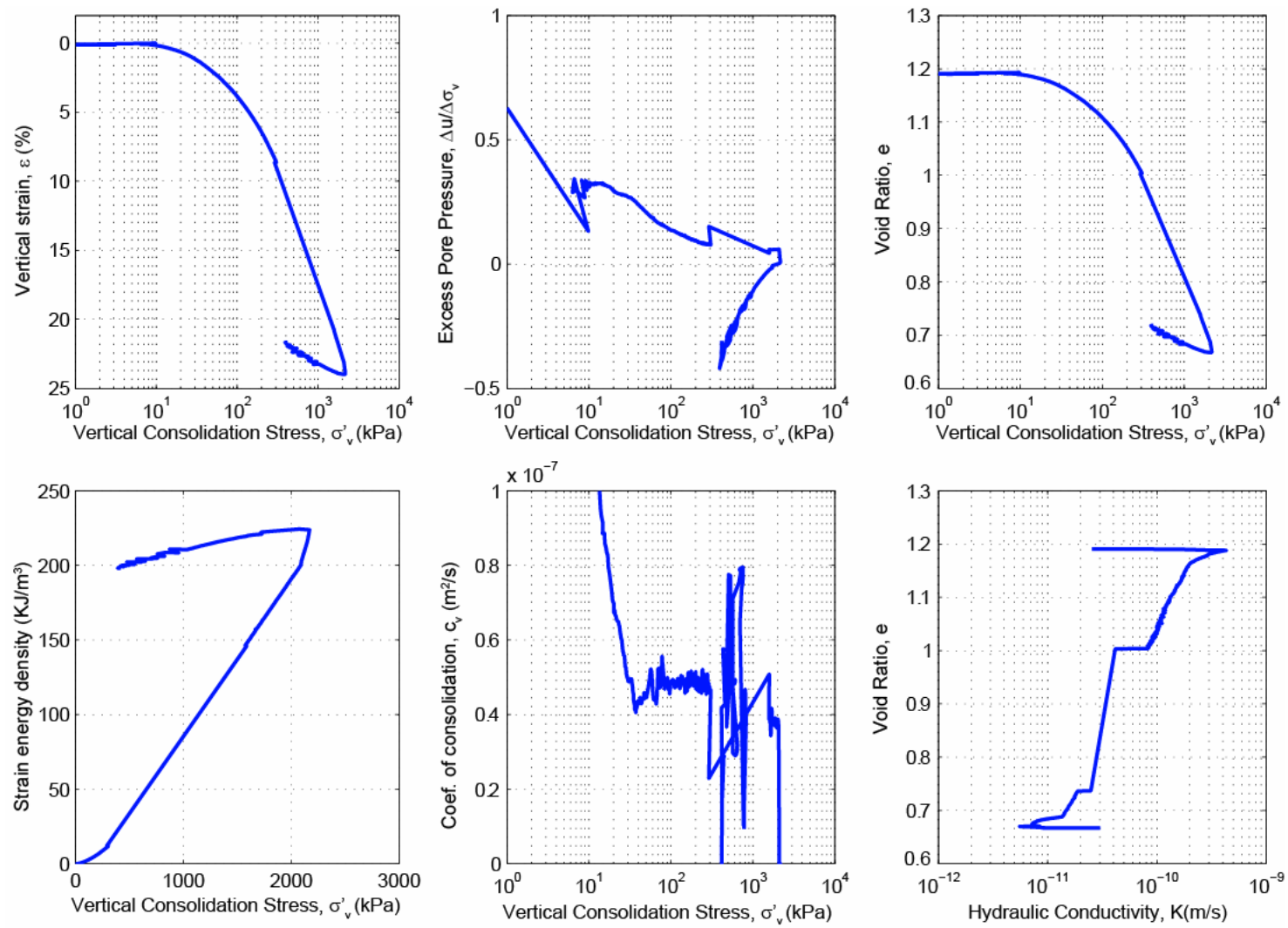
Figure B.4: CRS798 consolidation data for Sample U1322D-2H-2WR, 72.83 mbsf.
