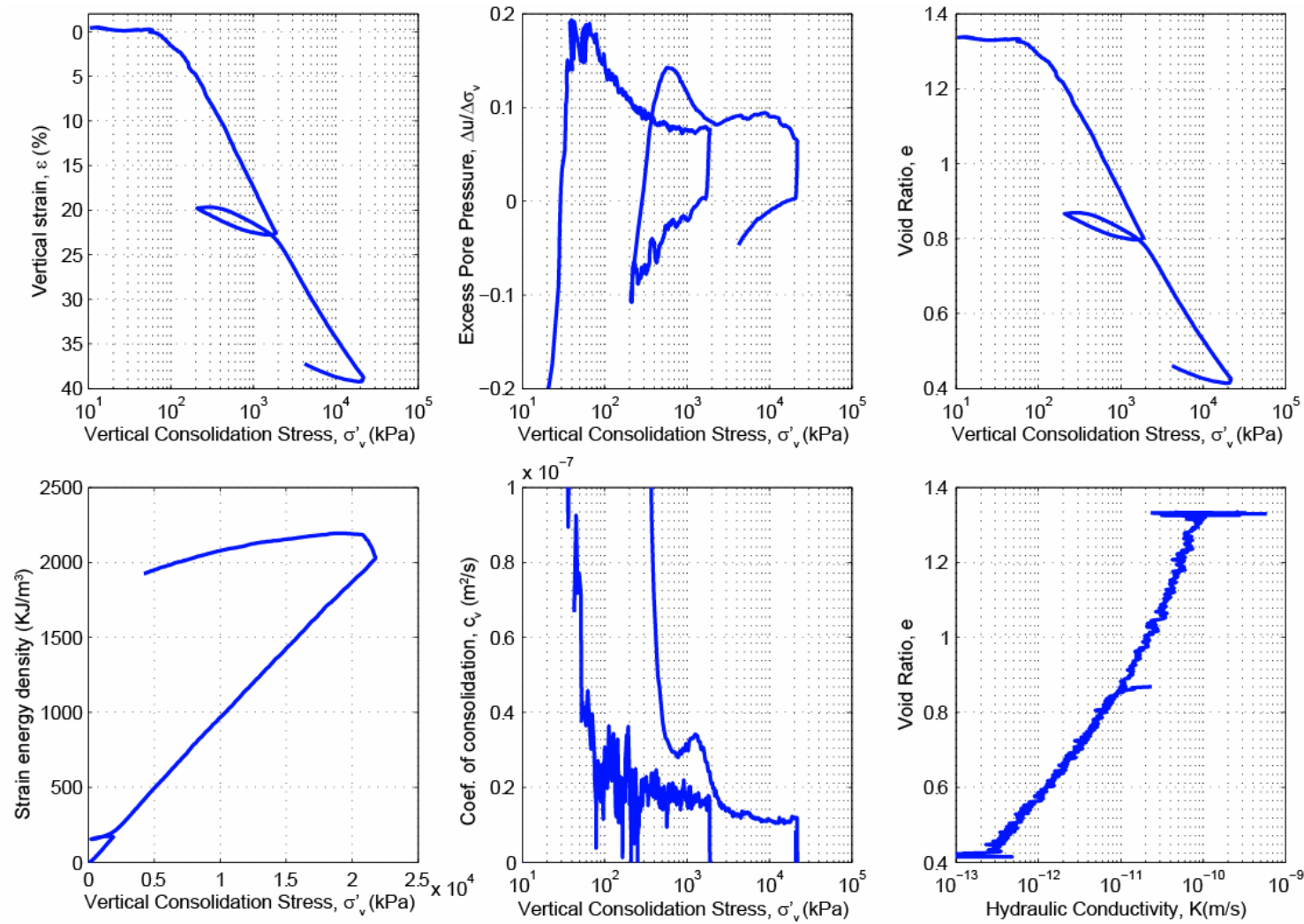
Figure B.21: CRS004 consolidation data for Sample U1324C-1H-1WR, 51.14 mbsf.
