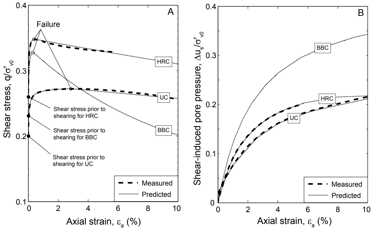
Figure 3.9: Data and predictions of K_0 -consolidated undrained compression test. The dashed lines represent experimental data and the dotted lines represent predictions of the MIT-T1 model. A) The stress-strain curve derived from compression test. The tested Ursa clay was from whole core sample U1324D-2H-2WR, 72 mbsf. B) The shear-induced pore pressure for compression test.
