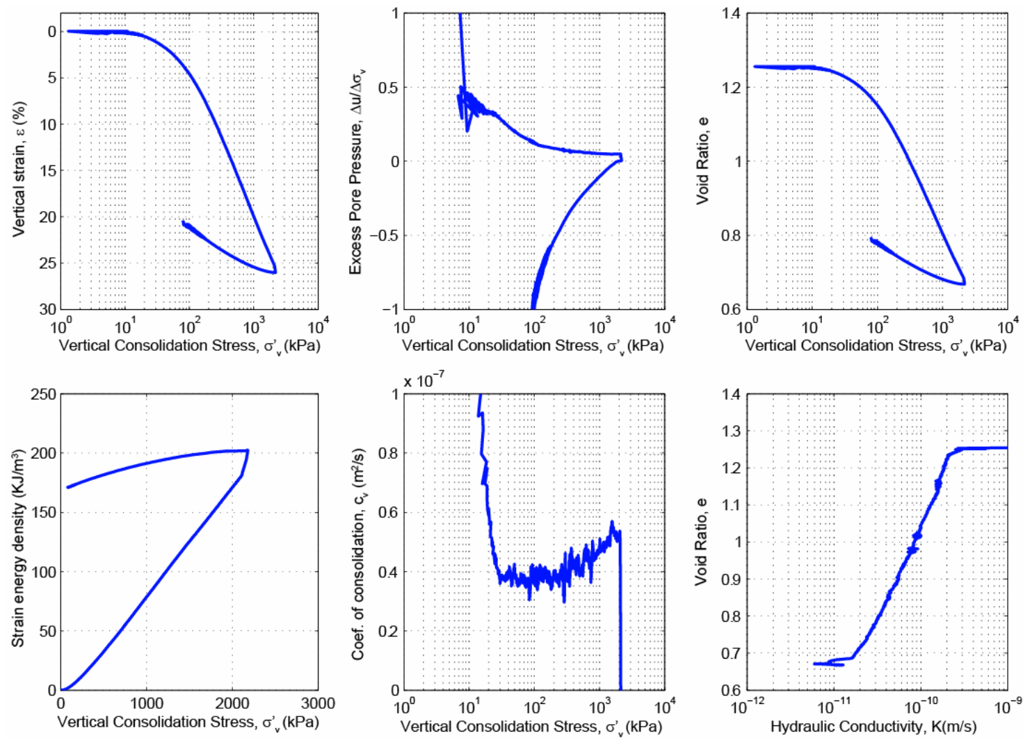
Figure B.6: CRS800 consolidation data for Sample U1324B-4H-7WR, 31.86 mbsf.
