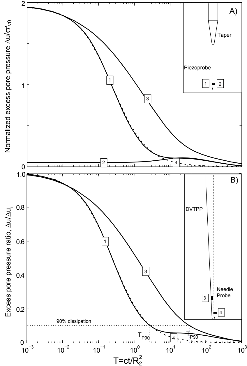
Figure 1.12: Modeled pressure dissipation for the Piezoprobe (#1, solid line) and the DVTPP (#3, solid line) penetrometers. A) Normalized excess pore pressure vs. dimensionless time. B) Excess pore pressure ratio vs. dimensionless time. The geometry of the Piezoprobe is shown in the top inset and the geometry of the DVTPP is shown in the bottom inset. Also shown is the dissipation response to a constant diameter thin probe ( R=3.2 mm) (Line #4, dotted line) measured at location 1 (Fig. 1.12A, inset) and the dissipation response to just the upper tapered shoulder and the overlying shaft at location 2 (Fig. 1.12A, inset) (Line #2, solid line). Dissipation time is normalized by the coefficient of consolidation and the radius of the shaft of the Piezoprobe.
