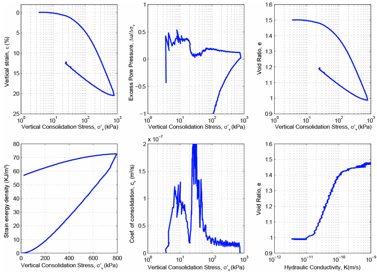
Figure B.3: CRS797 consolidation data for Sample U1324C-1H-1WR, 51.27 mbsf.
