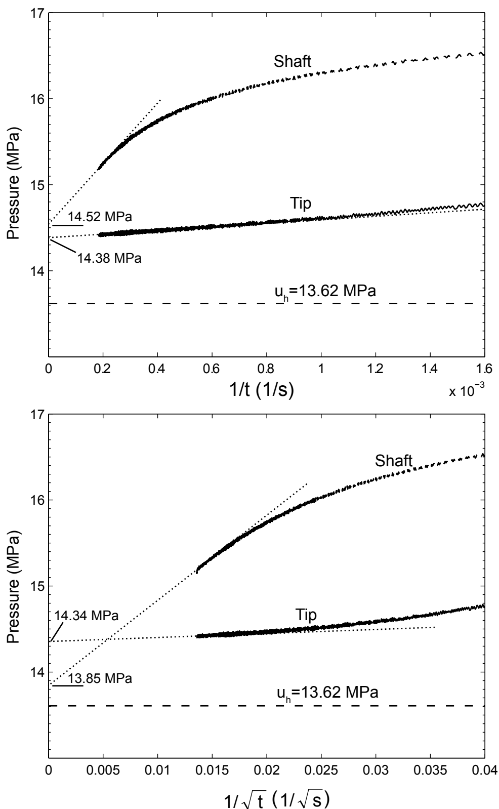
Figure 3.19: Estimating in situ pressure by 1/t and 1/\sqrt{t} extrapolations. A) Pressure dissipation plotted on inverse time ( 1/t ). A trend line is fit linearly to the last 5-minute dissipation data and projected to infinite time. B) Pressure dissipation plotted on inverse square root of time ( 1/\sqrt{t} ). A trend line is fit linearly to the last 5-minute dissipation data and projected to infinite time.
