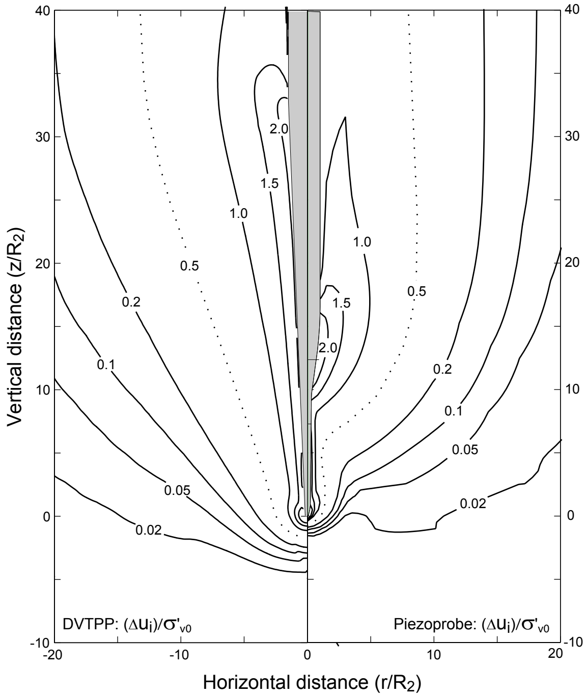
Figure 1.10: Penetration-induced pore pressures for the DVTPP (left) and the Piezoprobe (right). The DVTPP generates much larger pressures at equivalent radial distances from the tip. The initial excess pore pressure due to penetration, \Delta u_i , is normalized by the vertical effective stress ( \sigma'_{v0} ) prior to penetration.
