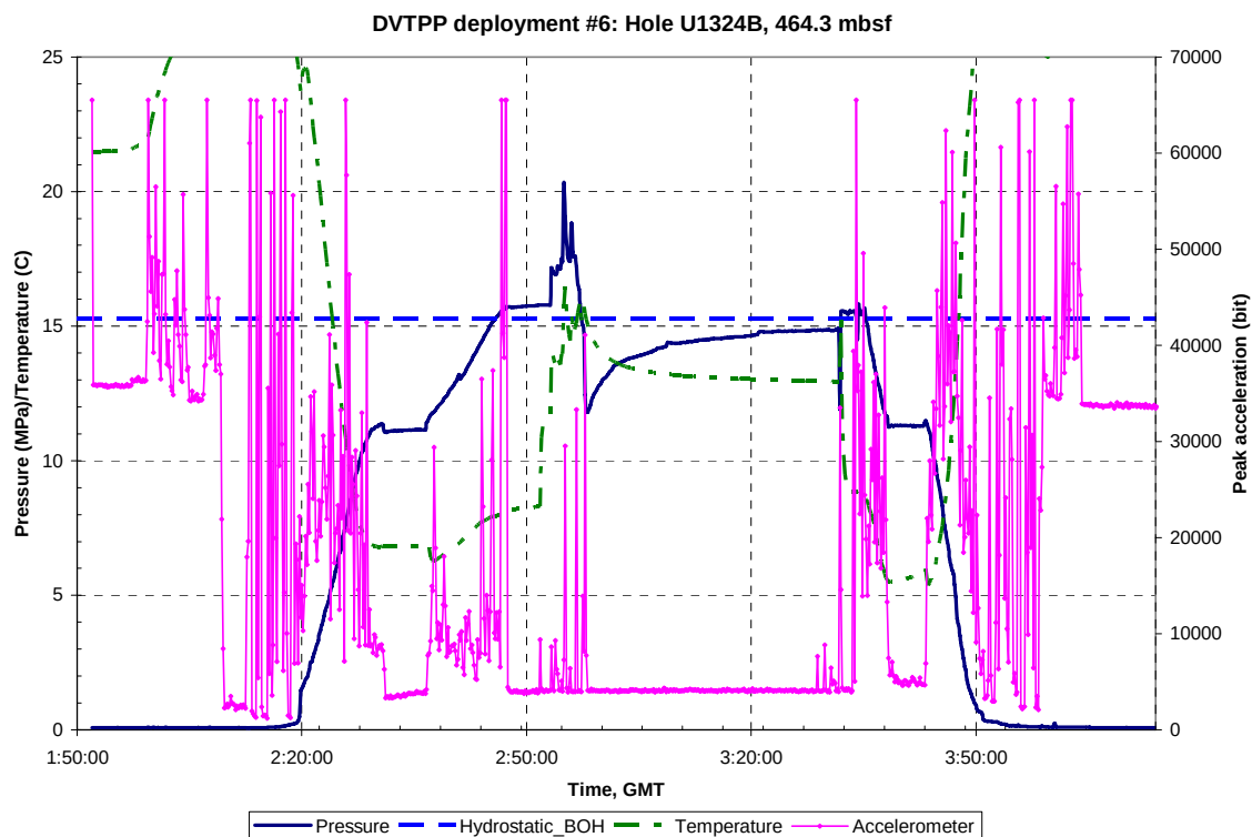
Figure A.A.6: Pressure, temperature and acceleration data for DVTPP Deployment #6, Hole U1324B, 464.3 mbsf. GMT = Greenwich Mean Time, Hydrostatic_BOH is the hydrostatic pressure at the bottom of the hole.
