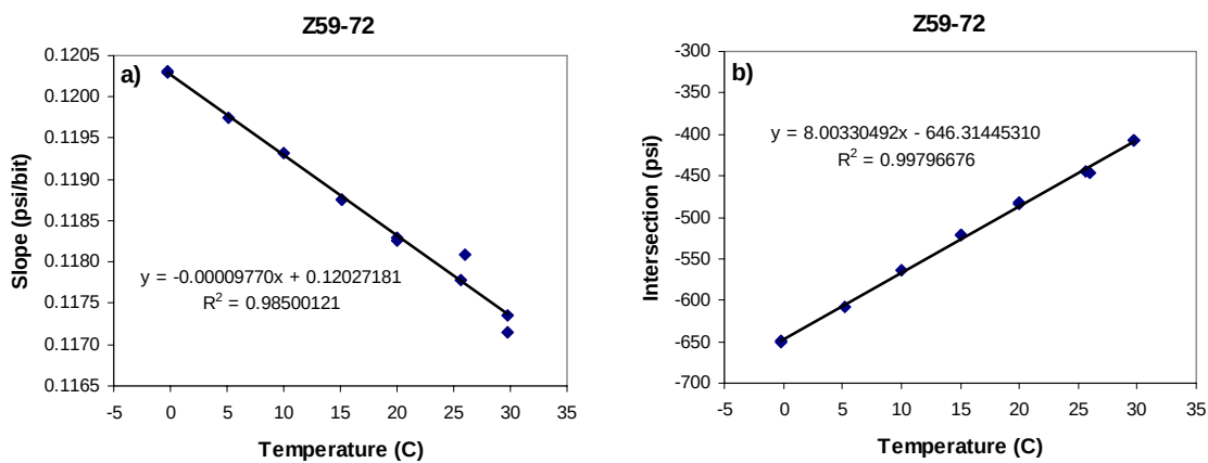
Figure A.B.5: Calibration coefficients of transducer Z59-72 vs. temperature. A) The slope of the calibration curve vs. temperature. b) The intersection on y-axis of the calibration curve vs. temperature.
