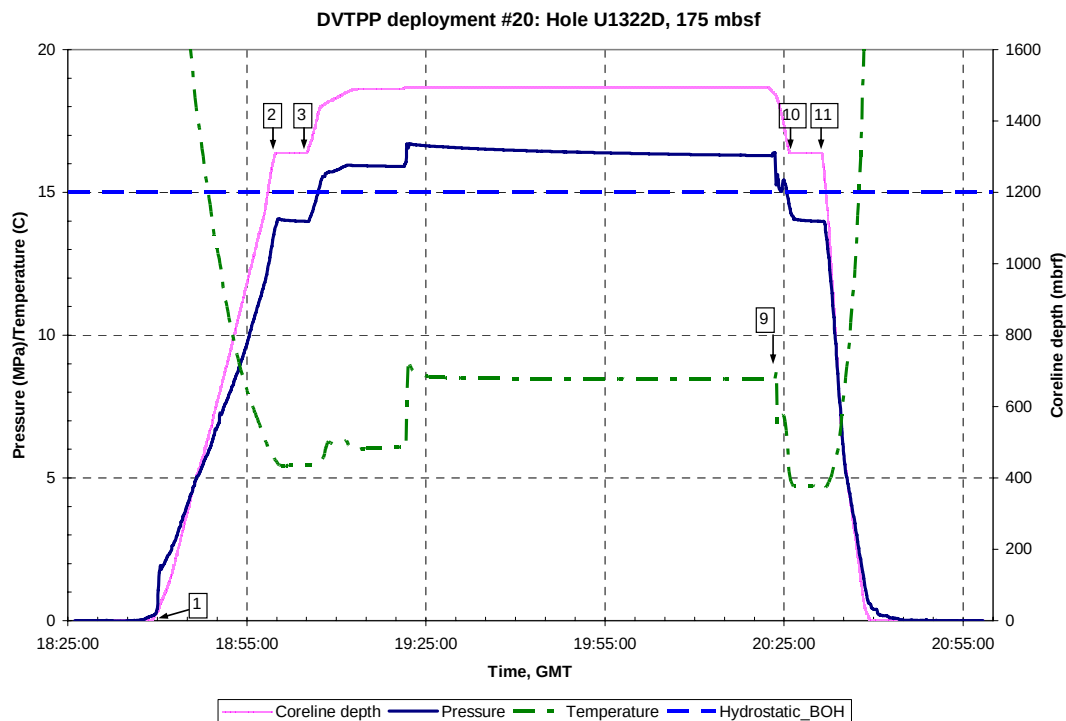
Figure A.A.1.a: Pressure, temperature and Truview data for DVTPP Deployment #20, Hole U1322D, 175 mbsf. GMT = Greenwich Mean Time, Hydrostatic_BOH is the hydrostatic pressure at the bottom of the hole.
