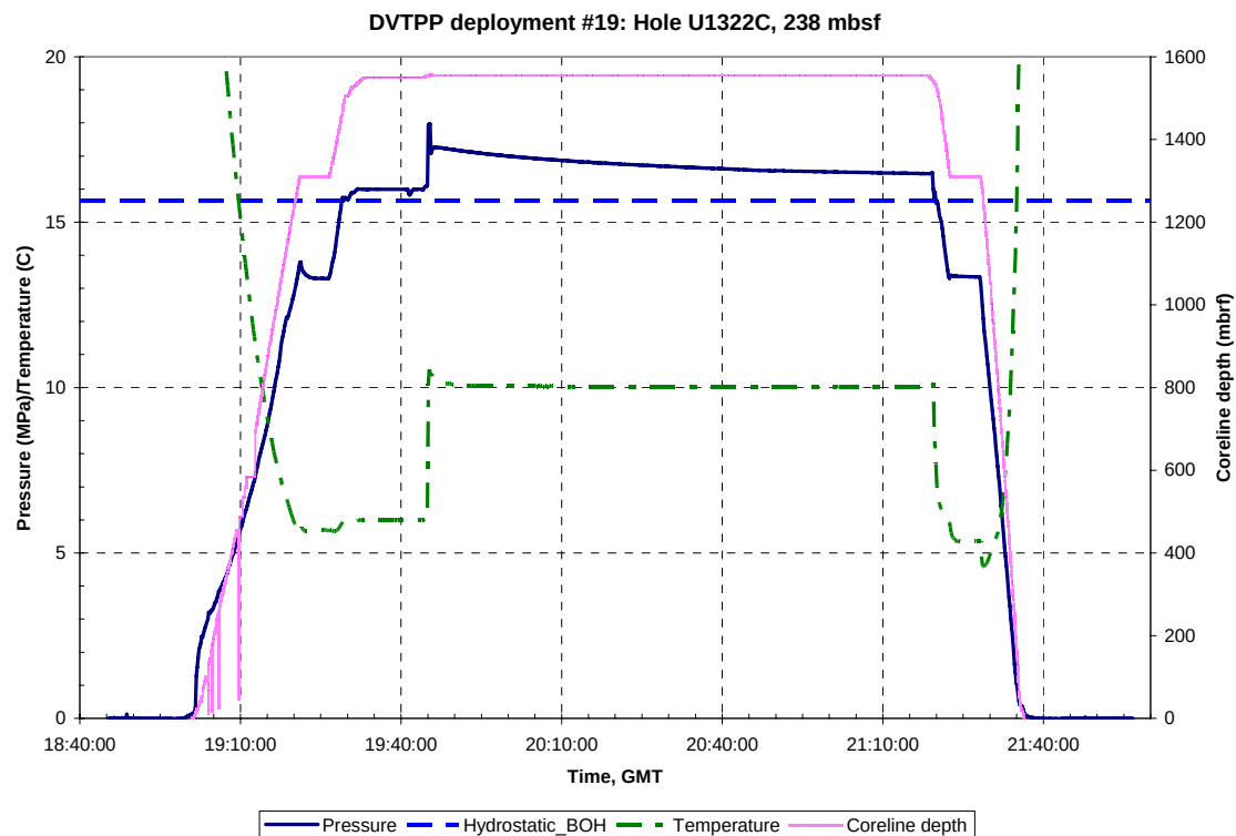
Figure A.A.18.a: Pressure, temperature and Truview data for DVTPP Deployment #19, Hole U1322C, 238 mbsf. GMT = Greenwich Mean Time, Hydrostatic_BOH is the hydrostatic pressure at the bottom of the hole.
