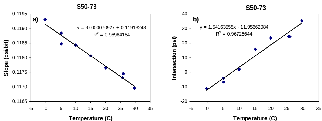
Figure A.B.4: Calibration coefficients of transducer S50-73 vs. temperature. A) The slope of the calibration curve vs. temperature. B) The intersection on y-axis of the calibration curve vs. temperature.
