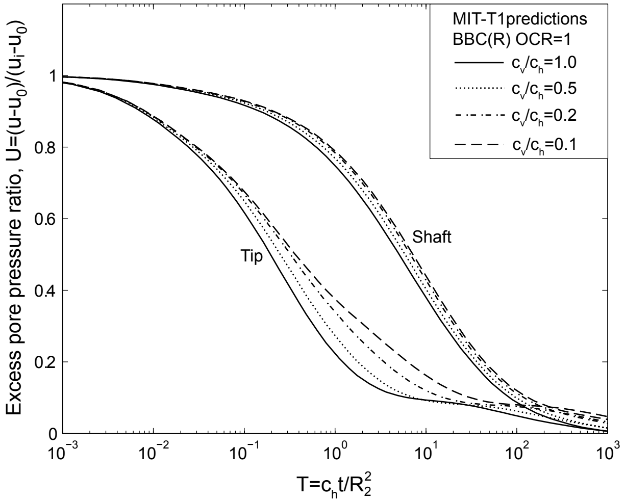
Figure 3.20: Effect of anisotropic hydraulic diffusivity on pressure dissipations.
