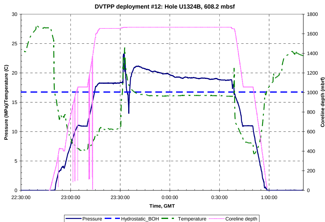
Figure A.A.11.a: Pressure, temperature and Truview data for DVTPP Deployment #12, Hole U1324B, 608.2 mbsf. GMT = Greenwich Mean Time, Hydrostatic_BOH is the hydrostatic pressure at the bottom of the hole.
