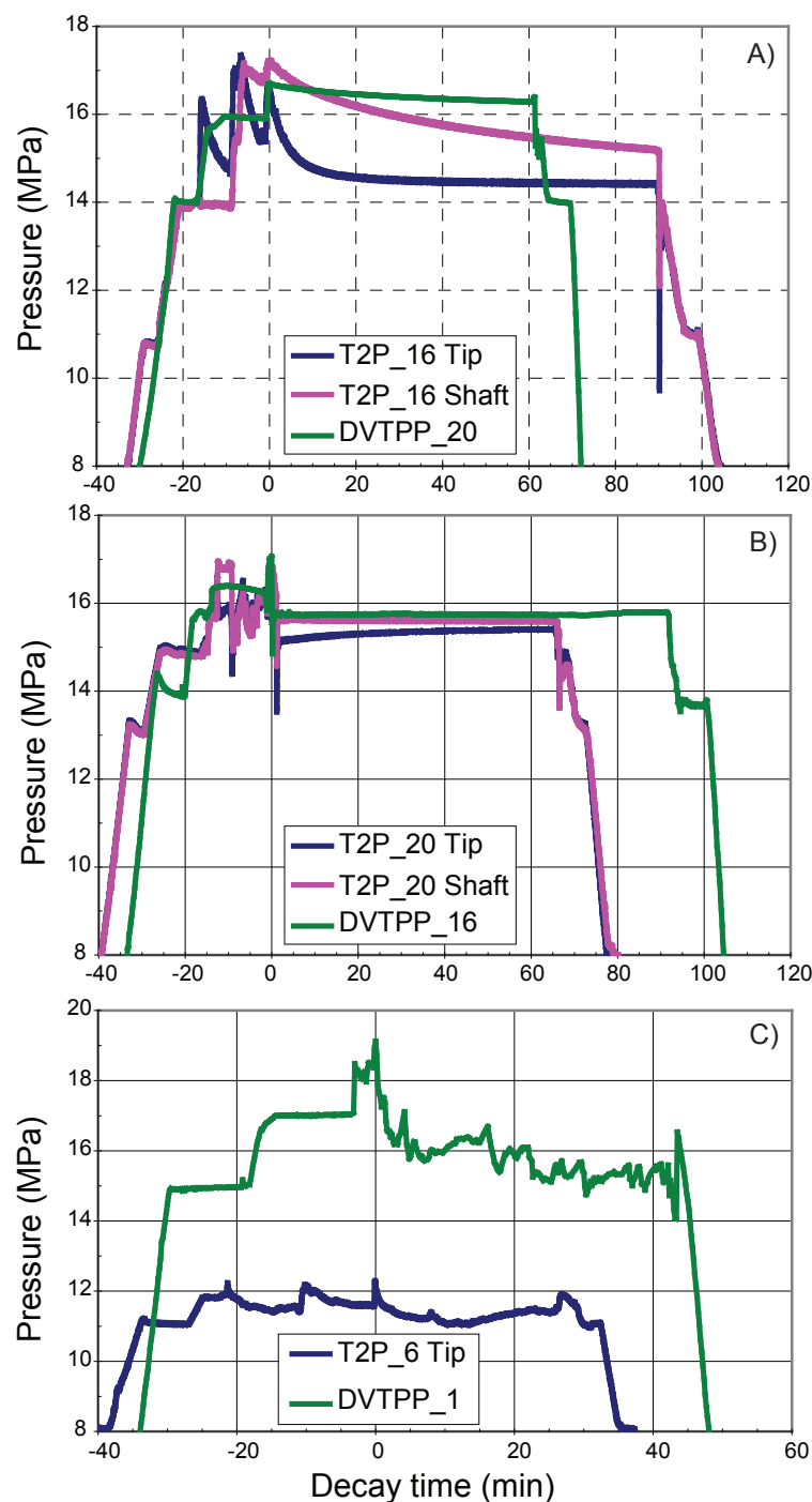
Figure A.7: Characteristic deployments of the DVTTP and T2P. A) Type I: typical pressure record for a penetration test with clear pressure buildup and clean pressure dissipation; B) Type II: pressure drops dramatically due to decoupling of the drill string from the tool. IIa) after the pressure drop, pressure decays towards in situ pressure; IIb) after the pressure drop, pressure builds up to in situ pressure; C) "Leak" deployments had abrupt and erratic changes in pressure during the dissipation phase. This is one example of a Type III deployment. Type III deployments include unsuccessful deployments due to hydraulic leaks, electronics failure, or tool damage and communication with borehole fluid.
