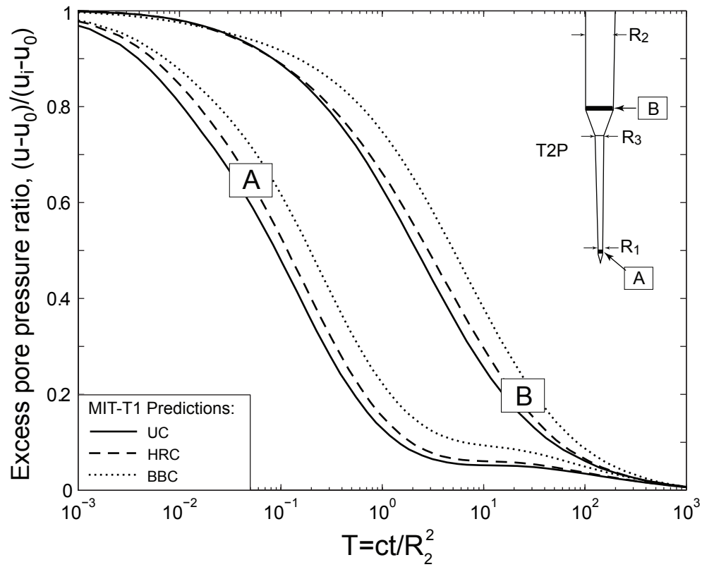
Figure 3.10: T2P pressure dissipation predicted at the tip (A) and Shaft (B) by full MIT-T1 soil model ( \Delta u_s is included) for three soil types: UC = Ursa Clay (solid line); HRC = Hydrate Ridge Clay (dashed line), BBC = Boston Blue Clay (dotted line).
