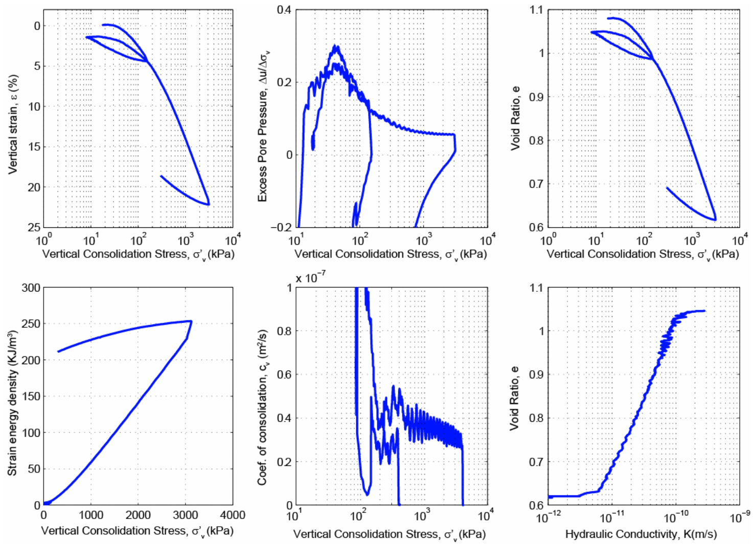
Figure B.14: CRS813 consolidation data for Sample U1324B-10H-7WR, 89.22 mbsf.
