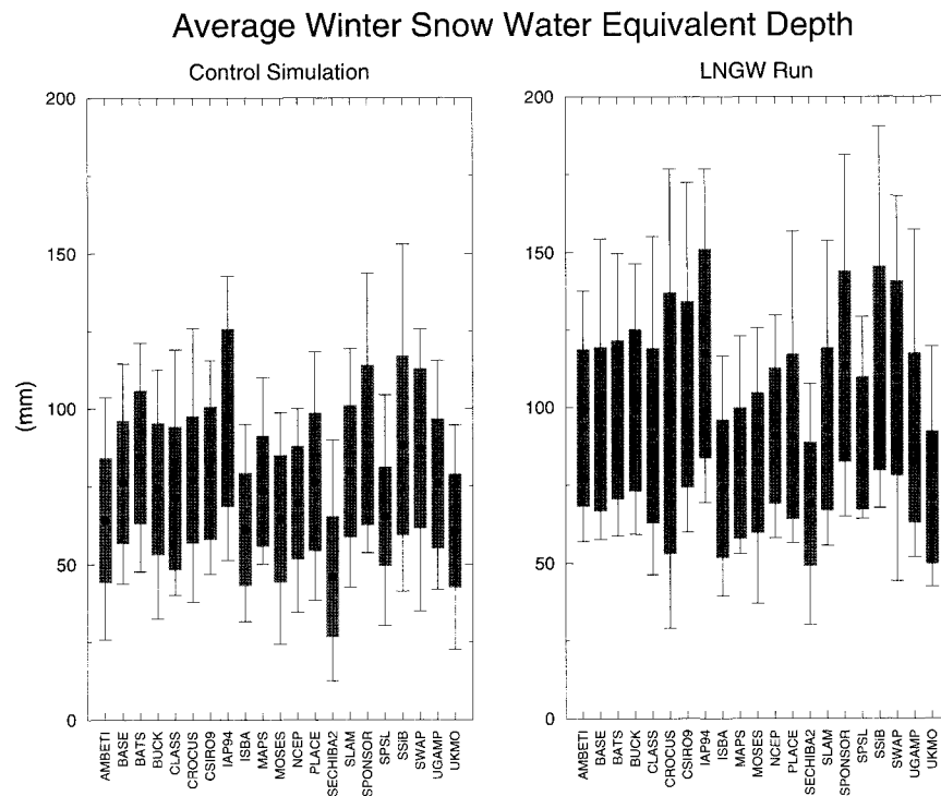
FIG. 6. As in Fig. 5 but averages are based on all of the daily averaged values of model output during the well-defined snowpack (and are therefore not compared to observations).
