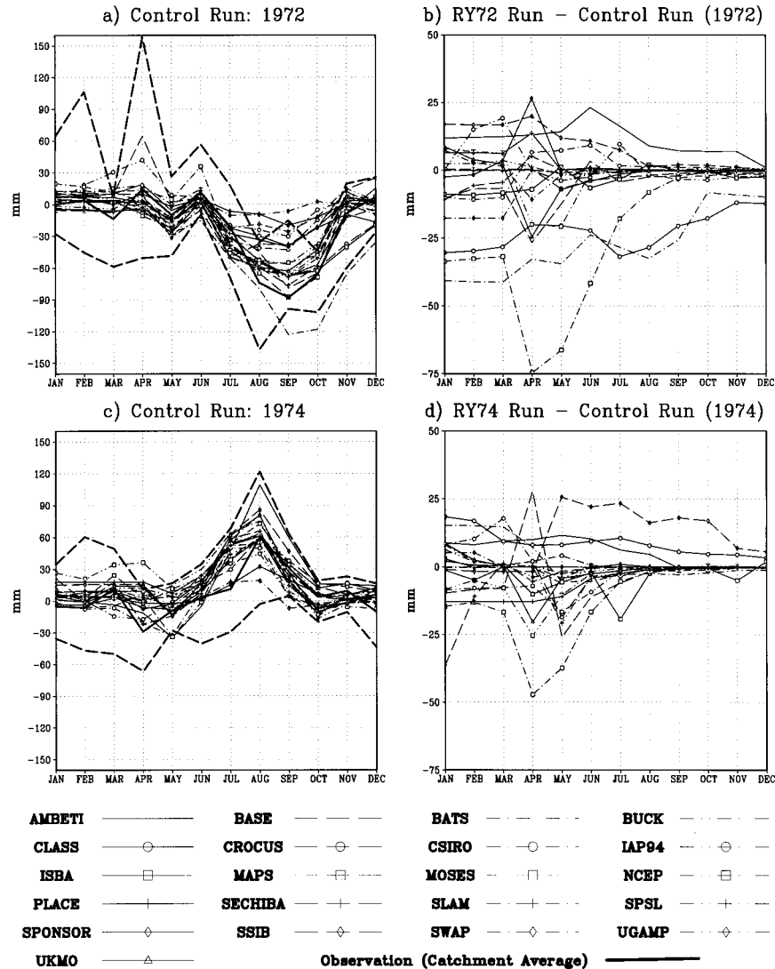
FIG. 10. Monthly anomalies (seasonal cycle removed) of root-zone total soil moisture for the model simulations and observations for the years (a) 1972 and (c) 1974. The differences in simulated soil moisture between the corresponding year of the control run and the (b) RY72 and (d) RY74 runs are also shown. Tick marks refer to the first day of the month. For observed total soil moisture, the catchment averaged value is given as a thick solid line, and the highest and lowest values of the seasonal cycles for the 11 observation sites within the catchment are indicated by the thick dashed lines.
