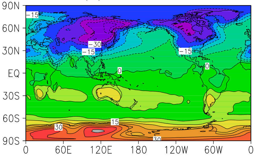
(c) DJF - JJA
