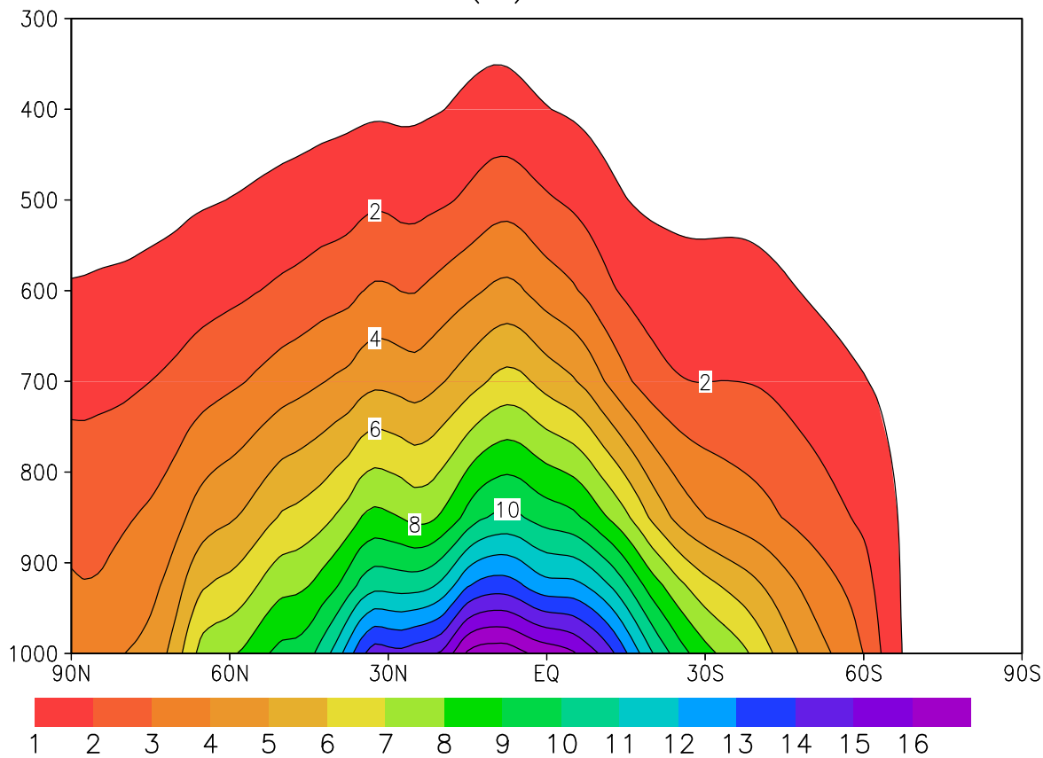
(b) JJA
