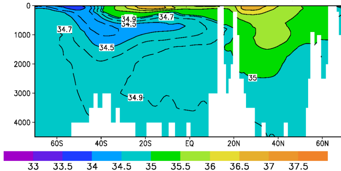
Figure 2.23c. Cross section of Atlantic salinity (psu) at 18°W.
