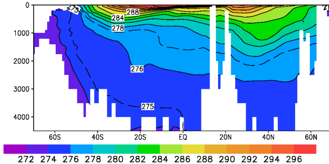
Figure 2.23b. Cross section of Atlantic temperature (K) at 18°W.
