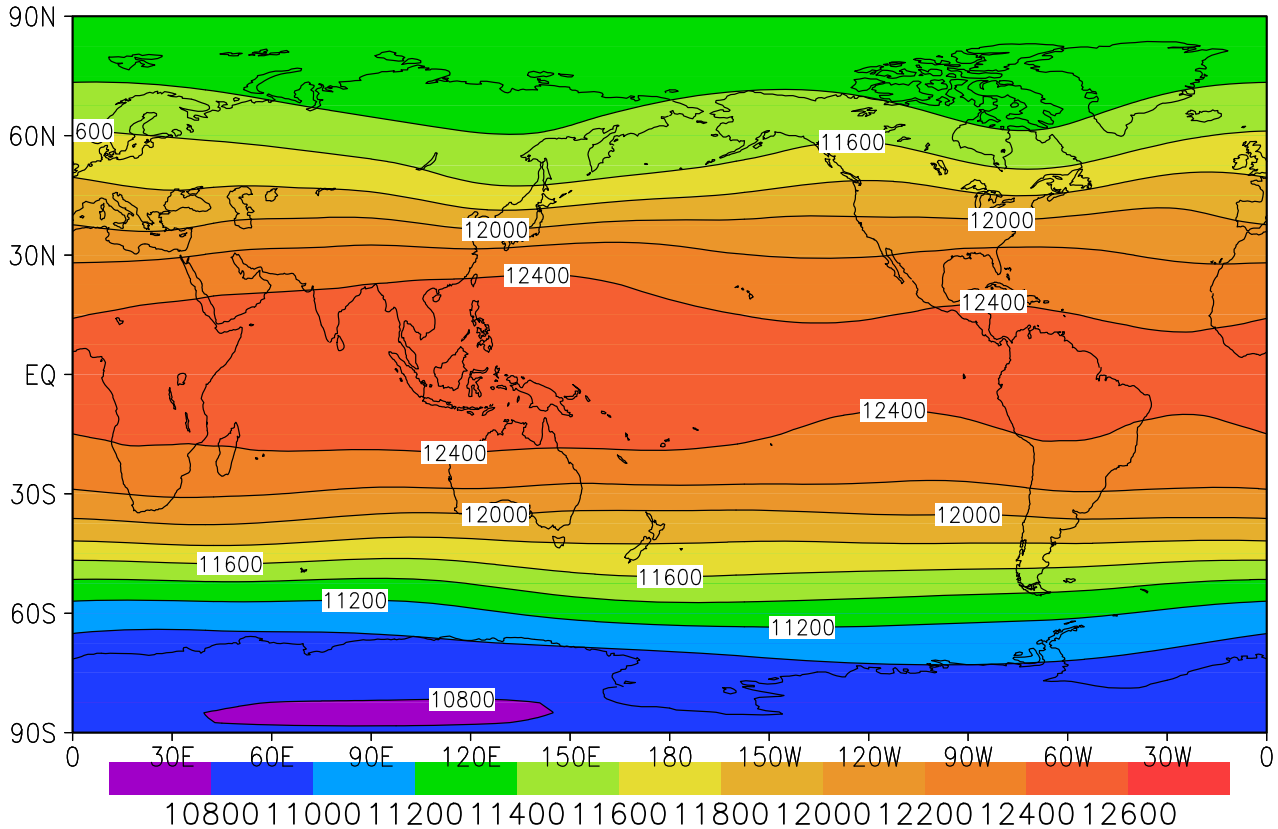
200 hPa Geopotential Height
