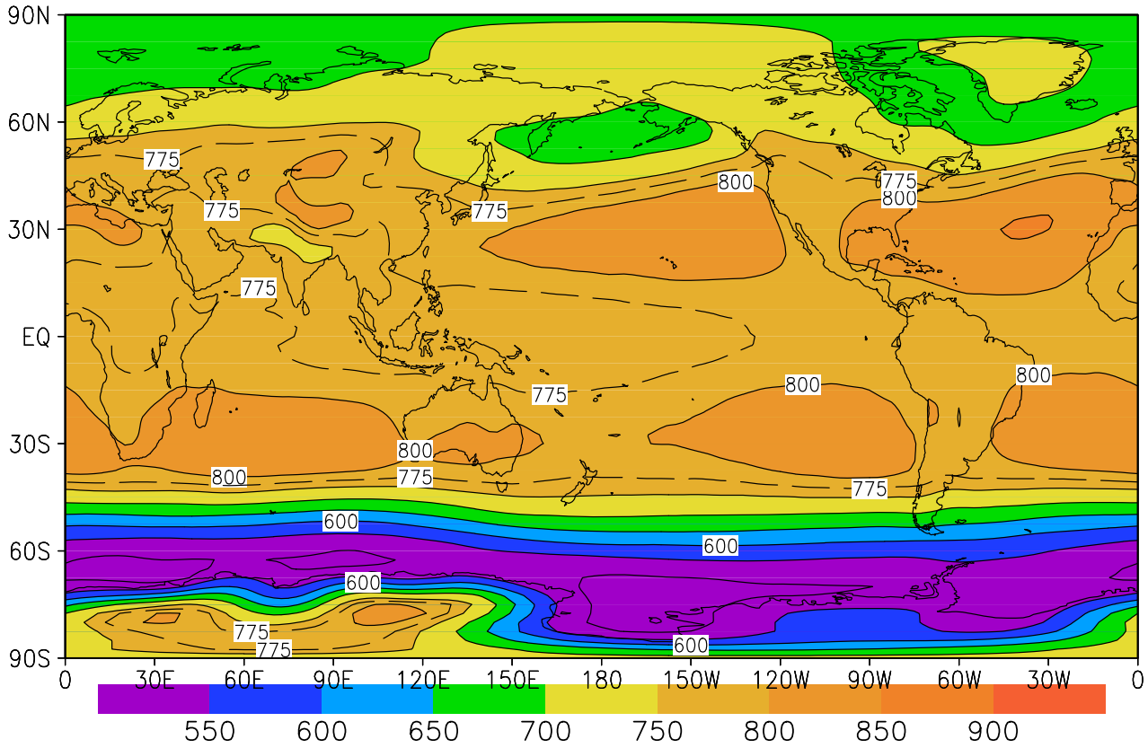
(a) 900 hPa Geopotential Height
