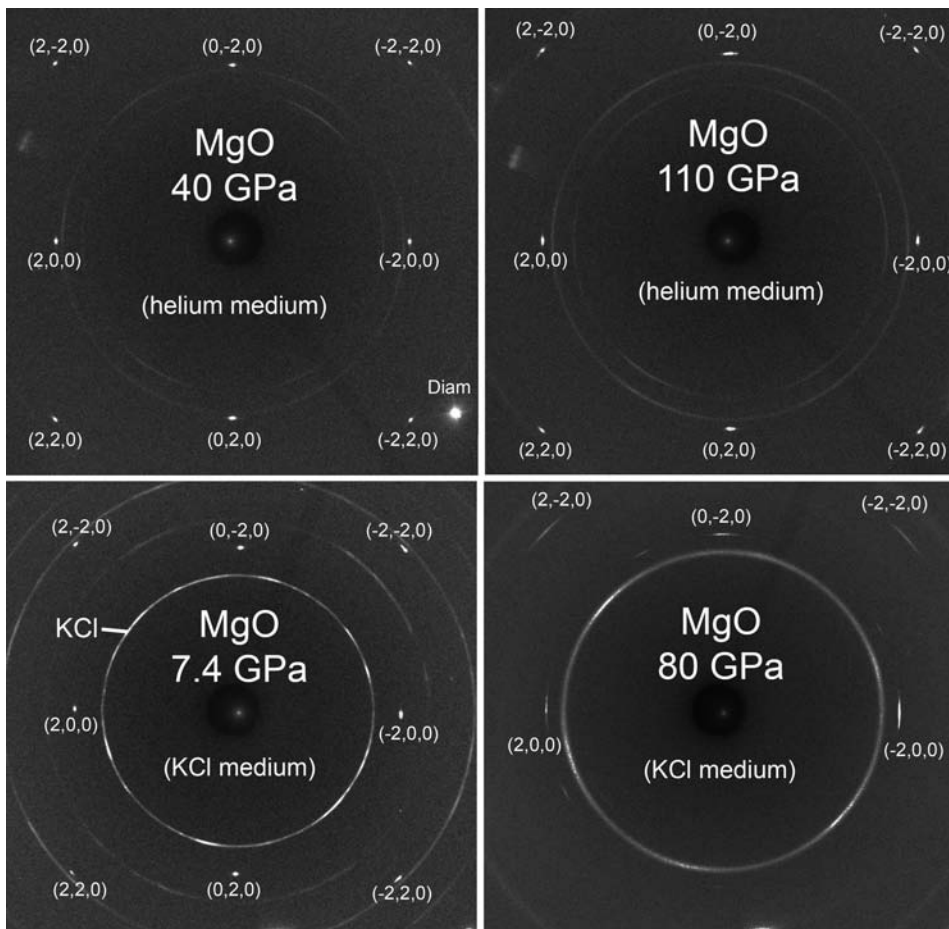
FIGURE 1. [100]-zone diffraction patterns of single-crystal MgO compressed in a helium pressure medium at 40 and 110 GPa (upper panels) and in a KCl pressure medium at 7.4 and 80 GPa (lower panels) taken with monochromatic synchrotron radiation at 45 keV. Diffraction patterns are rotated to place the (2,0,0) diffraction spots on the horizontal axis.
